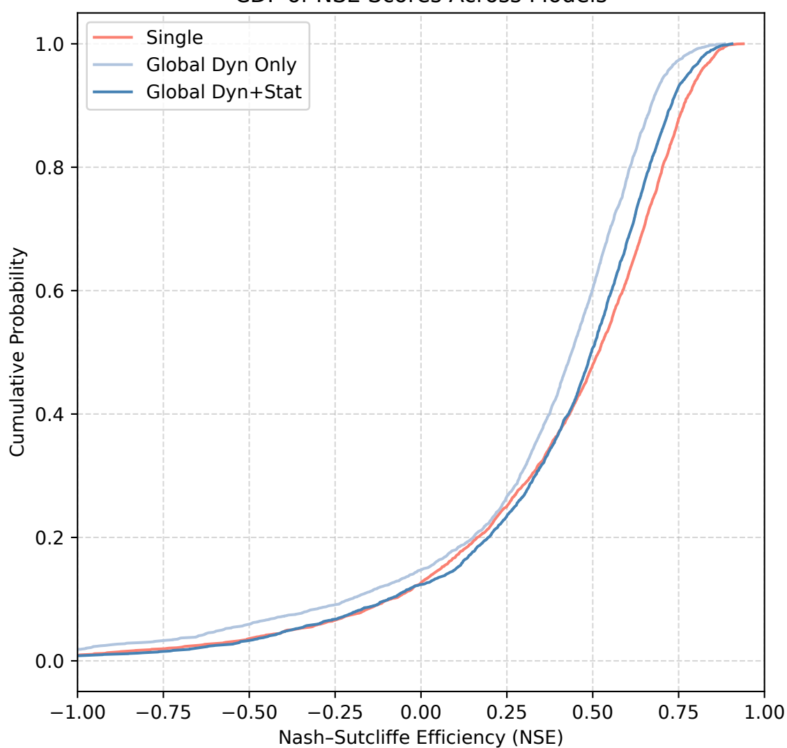
CDF of NSE Scores Across Models
