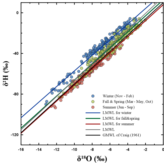
Figure 3. Local meteoric water lines (LMWLs) for precipitation on Jeju Island, South Korea. Individual samples are grouped by observation month into summer (June–September; JJAS), winter (November–February; NDJF), and transitional months (March–May and October). Seasonal regression lines summarize the observed \delta^{18}\text{O} – \delta^2\text{H} relationships, with the global meteoric water line (GMWL; Craig, 1961) shown for reference.
