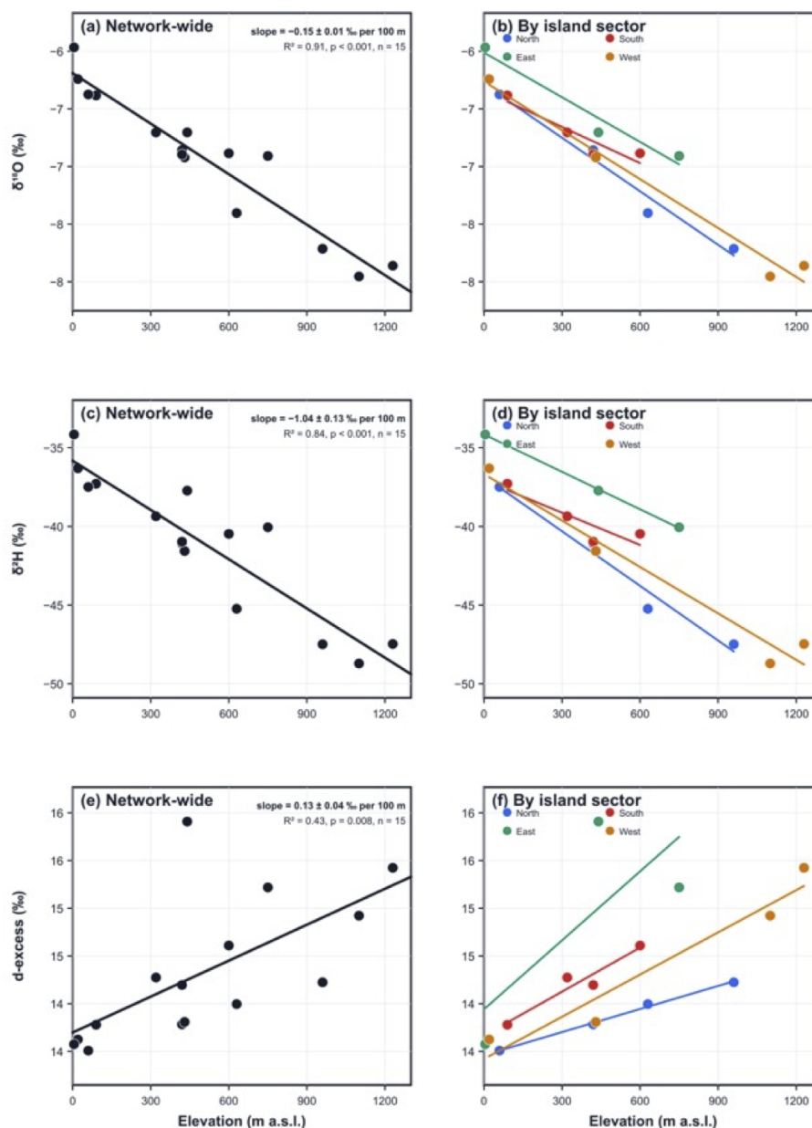
Figure 6. Relationships between station elevation and precipitation \delta^{18}\text{O} (a, b), \delta^2\text{H} (c, d), and d -excess (e, f) on Jeju Island, South Korea. Values represent unweighted station means calculated from available observations over the common 2002–2003 period. Panels (a), (c), and (e) show all 15 station means and the network-wide linear regressions. Panels (b), (d), and (f) show separate regressions for the northern, southern, eastern, and western sectors. Reported gradient uncertainties are standard errors. Sector-specific regressions are exploratory because each sector contains only three or four stations; separate fits do not establish statistically significant differences among sector slopes.
