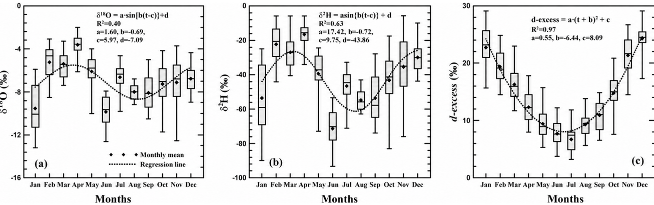
Figure 4. Calendar-month variations in precipitation isotopes on Jeju Island, South Korea. Seasonal patterns in (a) \delta^{18}\text{O} and (b) \delta^2\text{H} are summarized using sinusoidal functions with a fixed 12-month period, while (c) d -excess is summarized using a quadratic function. The fitted curves provide empirical descriptions of seasonal variability during the observation period. Boxes span the 25th–75th percentiles, and whiskers indicate the minimum and maximum values.
