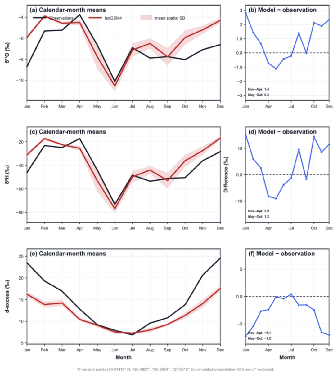
Figure 7. Calendar-month comparison of precipitation-isotope observations and IsoGSM4 output for \delta^{18}\text{O} (a, b), \delta^2\text{H} (c, d), and d -excess (e, f). Left panels show calendar-month means derived from unweighted monthly averages of available station observations (black) and retained values from three neighboring IsoGSM4 grid points (red). Red shading denotes \pm 1 standard deviation across the retained model grid points, representing spatial variability rather than model uncertainty. Right panels show IsoGSM4-minus-observation differences for each calendar month. Comparisons use matched observation months between September 2000 and December 2003. Model grid-point values with monthly mean precipitation below 0.2 \text{ mm d}^{-1} were excluded before spatial averaging. The central grid point is located on Jeju Island, while the western and eastern points are offshore; their mean therefore represents an island–nearshore regional approximation.
