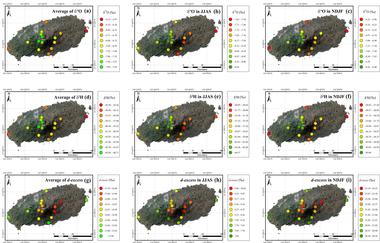
Figure 5. Spatial distributions of station-mean precipitation \delta^{18}\text{O} (a–c), \delta^2\text{H} (d–f), and d\text{-excess} (g–i) on Jeju Island, South Korea. Columns show overall means (a, d, g), summer means (June–September; JJAS; b, e, h), and winter means (November–February; NDJF; c, f, i), calculated from available observations at each station. Symbols indicate monitoring locations, and colors represent the corresponding station-mean isotope values.
