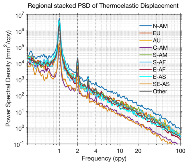
Figure 11. Regionally stacked power spectral densities of the TED time series.
