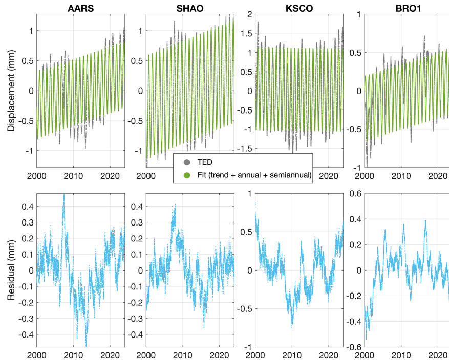
Figure 4. Examples of vertical TED time series at four representative GNSS stations. The upper panels show the daily FEM_{FL} TED series together with the fitted linear, annual, and semiannual components. The lower panels show the residuals after removing these fitted components.
