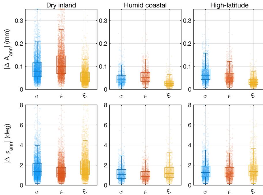
Figure 9. Sensitivity of the annual TED cycle to \pm 10\% perturbations in key parameters. Box-and-scatter summaries are shown for three regional groups: arid interior, humid coastal, and high latitude (defined as stations with absolute latitude \geq 60^\circ ). The tested parameters are \alpha (linear thermal expansion coefficient), \kappa (thermal diffusivity), and E (Young's modulus).
