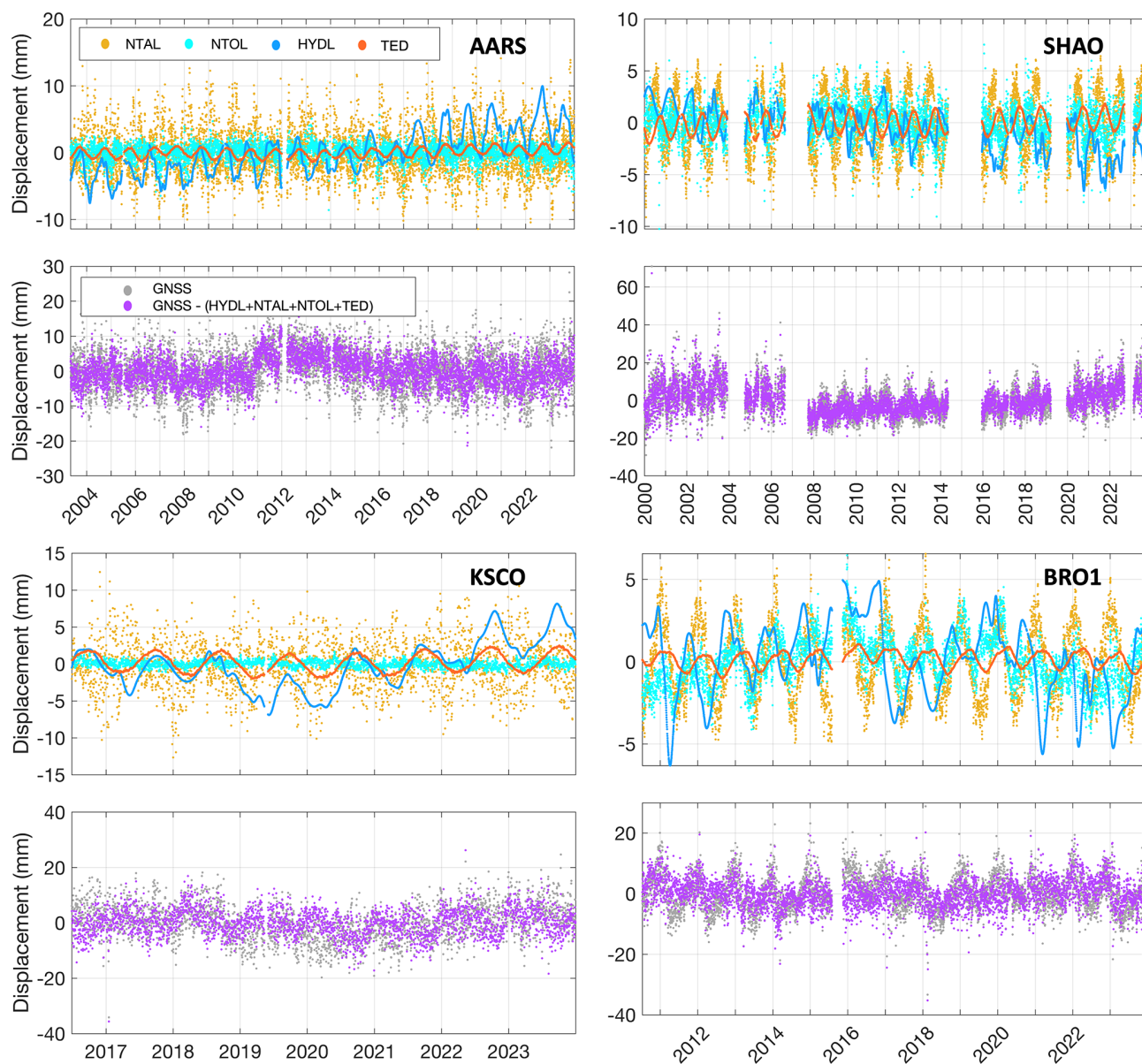
Figure 14. Component comparison at four representative GNSS stations. The upper panels show modelled displacements from NTAL, NTOL, HYDL, and TED. The lower panels compare the raw GNSS height series with the series after removing the combined TED, HYDL, NTAL, and NTOL corrections. These panels are shown only to illustrate the relative timing and amplitude of different environmental displacement components, rather than to evaluate the correction performance of TED alone.
