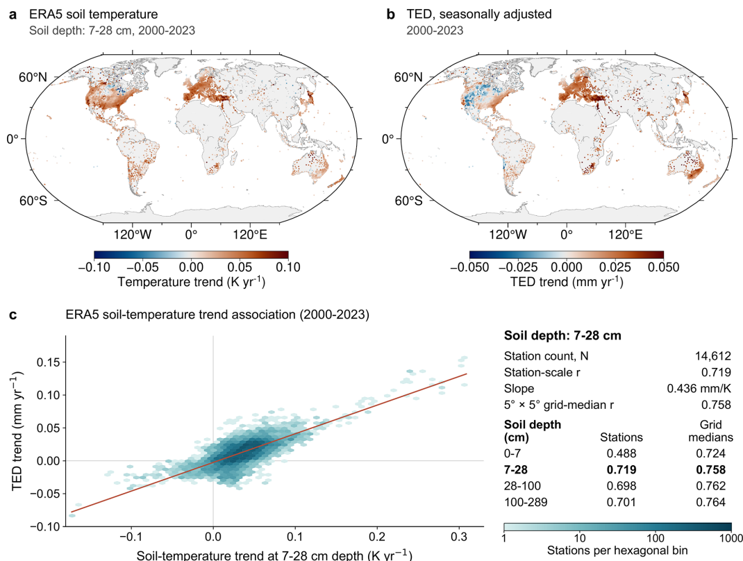
Figure 5. Relationship between low-frequency TED variations and ERA5 soil-temperature trends. (a) Linear trends of ERA5 soil temperature at 7–28 cm depth during 2000–2023. (b) Linear trends of TED after removing the annual and semiannual components. (c) Relationship between soil-temperature trends and TED trends at GNSS stations. The table in panel (c) summarizes Pearson correlation coefficients for the four ERA5 soil-temperature layers at the station and 5^\circ \times 5^\circ grid-cell scales.
