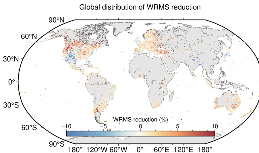
Figure 12. Global distribution of WRMS changes after applying the TED-only correction to GNSS height time series. Positive values indicate reduced WRMS after removing TED, while negative values indicate increased WRMS.
