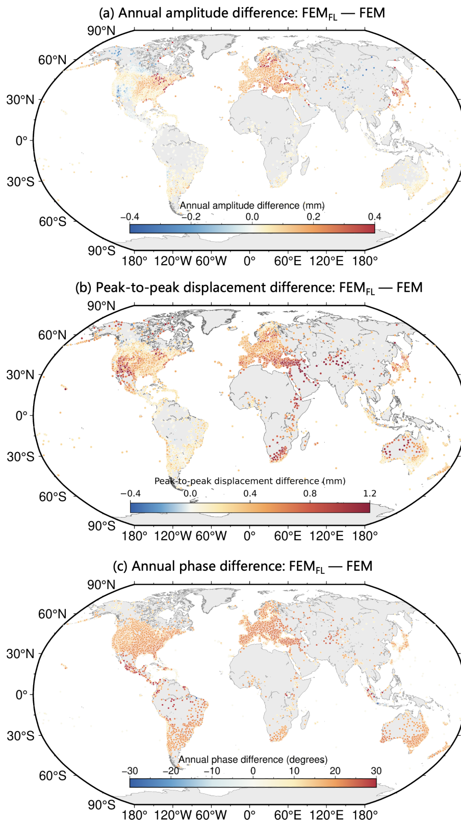
Figure 7. Station-based differences between the FEM_{FL} TED product and the traditional homogeneous FEM solution. Panels (a–c) show the differences in annual amplitude, percentile-based peak-to-peak displacement, and annual phase, respectively.
