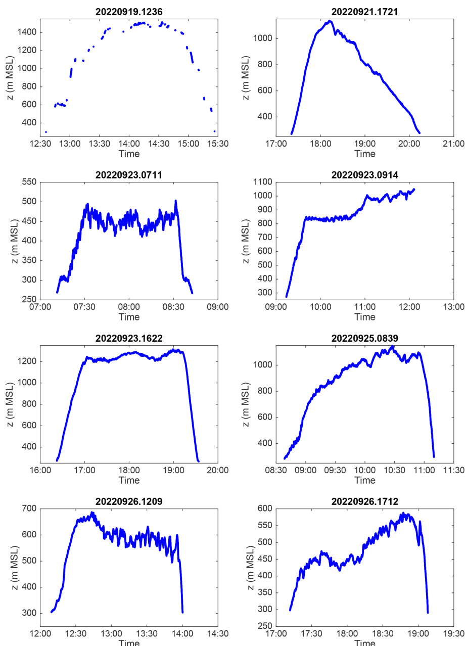
Figure 3. Time series of barometric altitude measured with the pss8 device aboard the MPCK + instrument, the flight numbers are given in each panel title. Flight 20220919.1236 (top row) had issues with the power supply, resulting in visible gaps of the data record.
