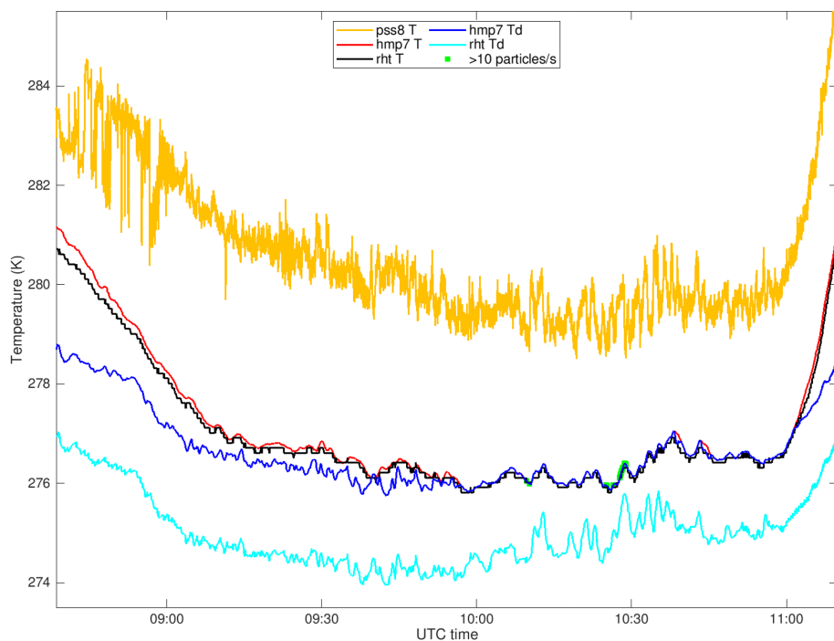
Figure 4. Temperature (orange, red and black lines) and dew point temperature (blue and cyan lines) measured by or calculated from different MPCK + sensors for Flight 20220925.0839 as a function of time. Shown are temperature data from the pss8 system (orange), temperature data from the hmp7 sensor (red), temperature data from the rht sensor (black), dew point data from the hmp7 sensor (blue), and dew point data from the rht sensor (cyan). In addition, the green squares indicate times when the FCDP measured 10 or more particles larger than 10 \mu\text{m} , which indicates the presence of a cloud.
