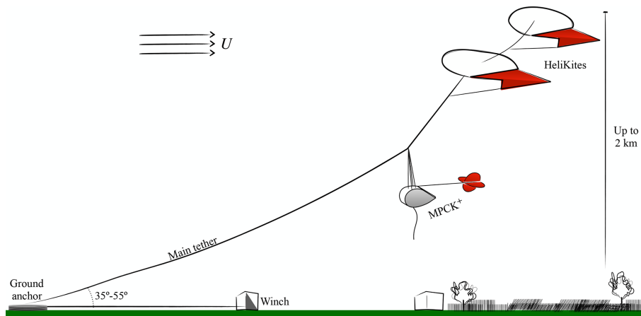
Figure 2. Illustration of the MPCK platform with MPCK + as scientific payload, installed on the main tether, with tandem helikite configuration.
