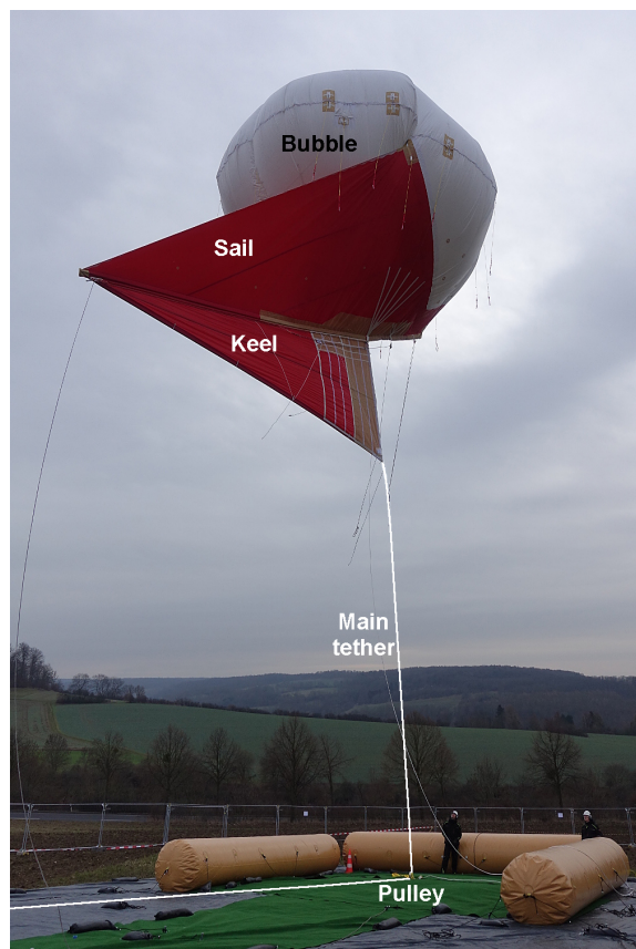
Figure 1. A 250 m 3 Helikite during a test flight next to the institute location of MPI-DS.
