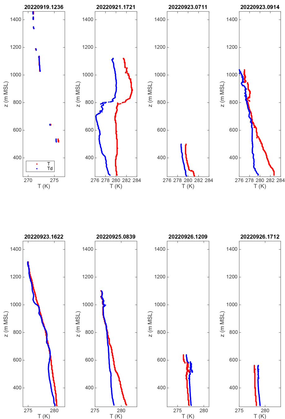
Figure 8. Vertical profiles of temperature and dew point for all eight MPCK + flights. Shown are temperature (red) and dew point (blue) as defined in Sect. 3.3 as a function of GPS altitude above mean sea level. The flight names are given in the title of each panel.
