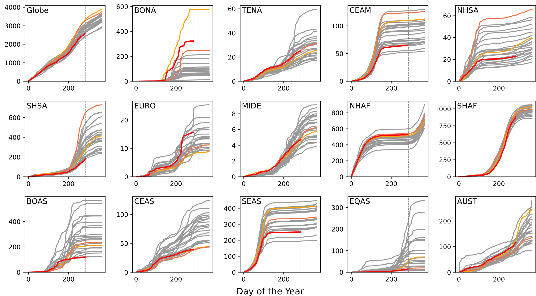
(b) Cumulative global and regional fire emissions (Tg C)
