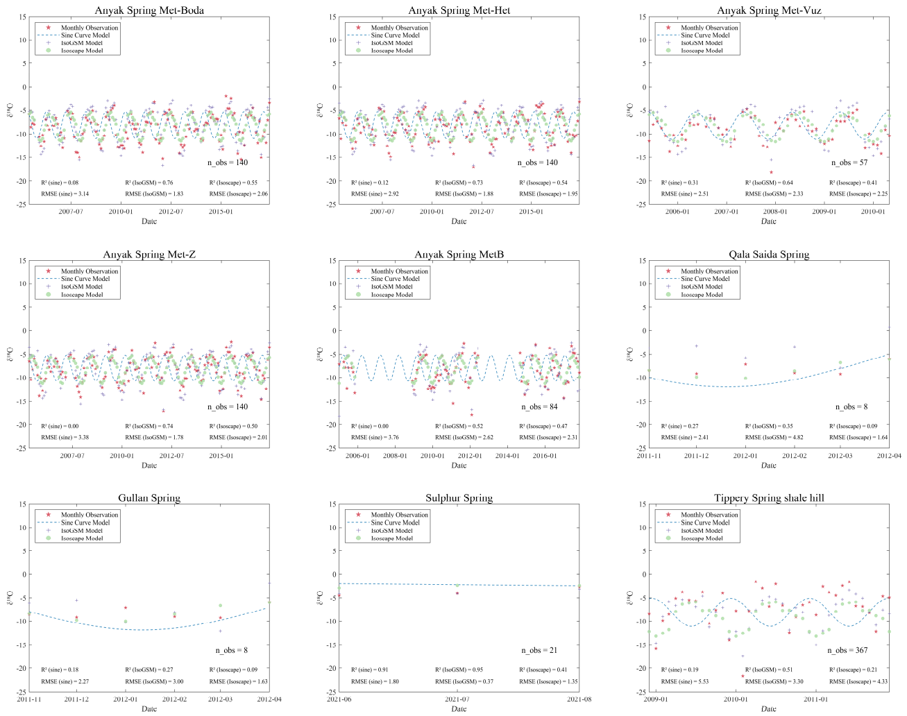
Figure S1: Time series comparison of modelled and observed monthly \delta^{18}\text{O} in precipitation at 51 sites. Observations (red stars) are compared with estimates from the Sine Curve model (dashed blue line), IsoGSM (purple crosses), and the Isoscape model (green circles). Each panel shows the number of monthly observations ( n_{\text{obs}} ) and model performance statistics ( R^2 and RMSE).
