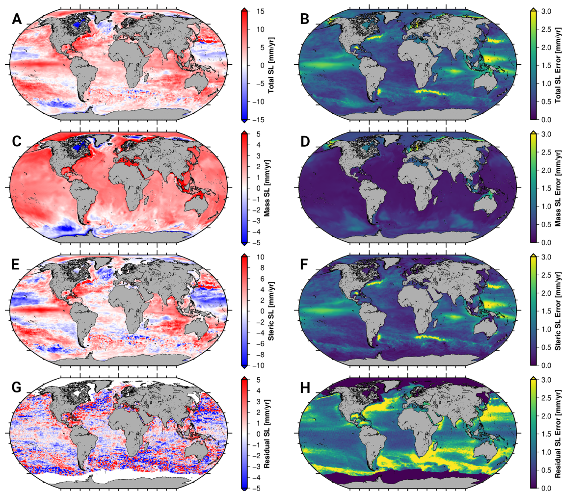
Figure B2. Major regional sea level budget components from the global fingerprint inversion approach. Left column (A, C, E, G) shows the trends from January 2005 till December 2015 and right column (B, D, F, H) shows corresponding trend errors. Note: As the residual component is derived from gridded along-track altimetry residuals, we masked out the area of maximum sea ice extend as seasonally missing along-track altimetry coverage might affect residual trend results in these regions.
