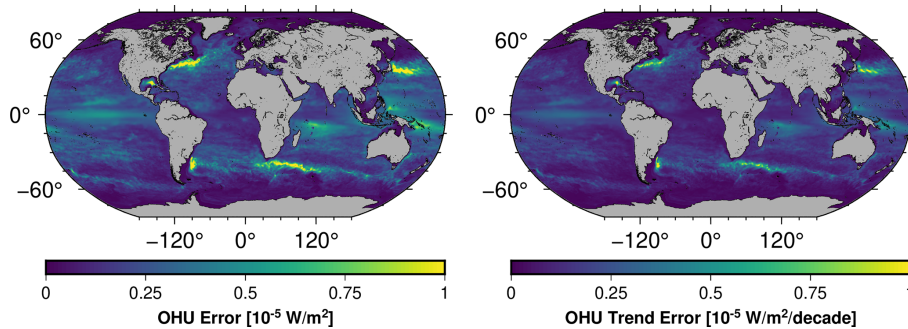
Figure 7. Regional ocean heat uptake (OHU) errors and OHU trend errors as derived from our GAAMR method over January 2005 till December 2024.
