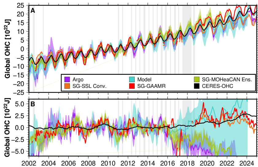
Figure 1. Global mean ocean heat content (OHC) change. (A) Full OHC signal. (B) Residual inter annual signal after removing the fitted signal (mean/trend/acceleration/seasonal) for the period January 2005 till December 2015. Months with missing GRACE/GRACE-FO data are indicated by the light-grey shaded vertical stripes. The groups Argo and Model are comprised by all corresponding data products from Table 1, whereas the space geodetic contributors consists of an ensemble of MOHeaCAN data (Table 1) and from our inversion results by directly converting steric sea level to OHC using a globally constant factor (Sect. 2.4.1) and our proposed GAAMR method (Sect. 2.4.2). The shading of the groups represents the full ensemble spread. Note: The residuals are computed over the aforementioned period and removed from the entire time series, leading to artifacts outside of the 11 yr period that is covered by all datasets. Outside of this analysis period and with fewer ensemble members residuals will become artificially large.
