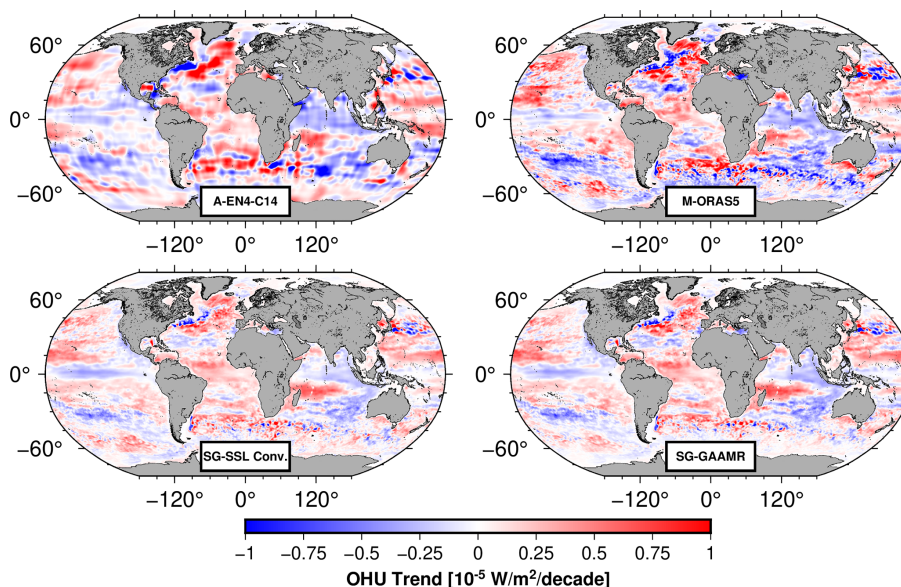
Figure 6. Regional ocean heat uptake (OHU) trend over January 2005 till December 2024.
