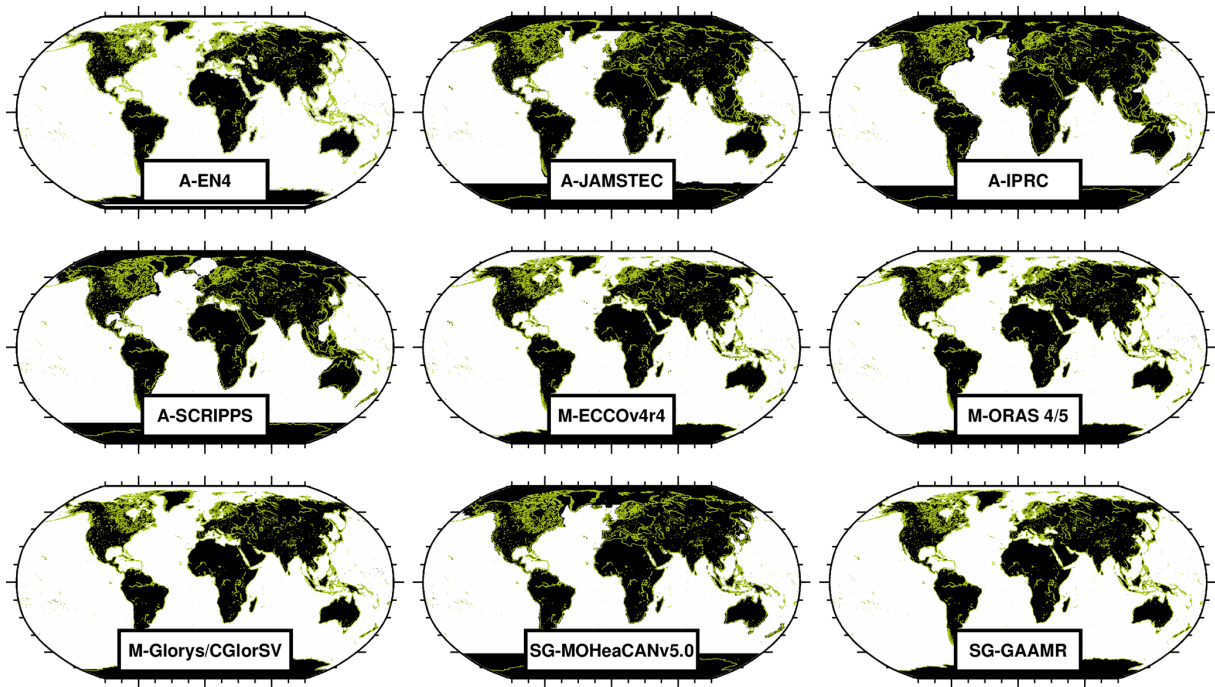
Figure B1. Spatial data coverage for individual data products introduced in Table 1.
