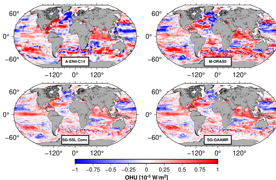
Figure 5. Regional ocean heat uptake (OHU) over January 2005 till December 2024.
