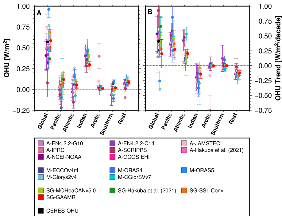
Figure 2. Ocean heat uptake (OHU) estimates (A) and corresponding OHU trends (B) derived from various Argo (A), model (M) and space geodetic (SG) datasets (Table 1) as well as our fingerprint inversion based GAAMR method (Sect. 2.4.2) for the period January 2005 till December 2015. Estimates are provided for the global ocean and individual sub-basins (see Fig. 3). Note that some datasets only provide global averages and can thus not be evaluated for the sub-basins.
