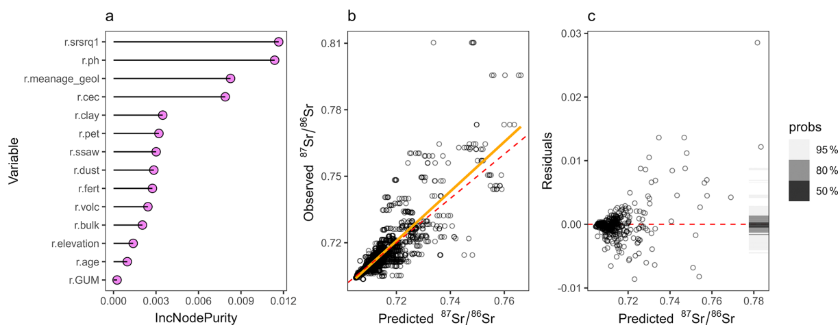
Figure 6. Predictive variables and model accuracy for random forest model based on plant + lichen samples. Increase in Node Purity (IncNodePurity) of the n = 14 external predictors (a); cross-validation scatterplot of observed vs. predicted ^{87}\text{Sr}/^{86}\text{Sr} values for the test-validation sample splits (b); model residuals vs. predicted ^{87}\text{Sr}/^{86}\text{Sr} ratios (c).
