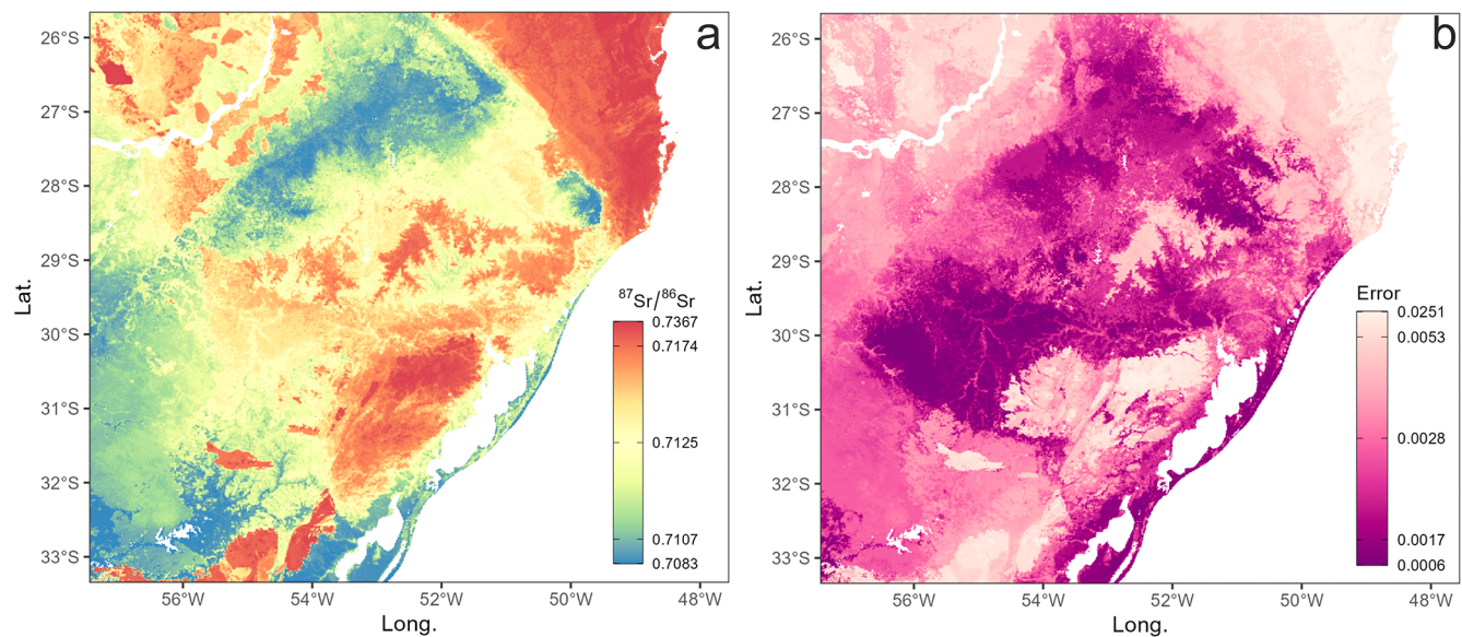
Figure 5. Spatial distribution of strontium isotopes in Santa Catarina and Rio Grande do Sul states based on plant + lichen samples ( n = 531 sites). Isoscape random forest model (a) and associated spatial uncertainty map (b).
