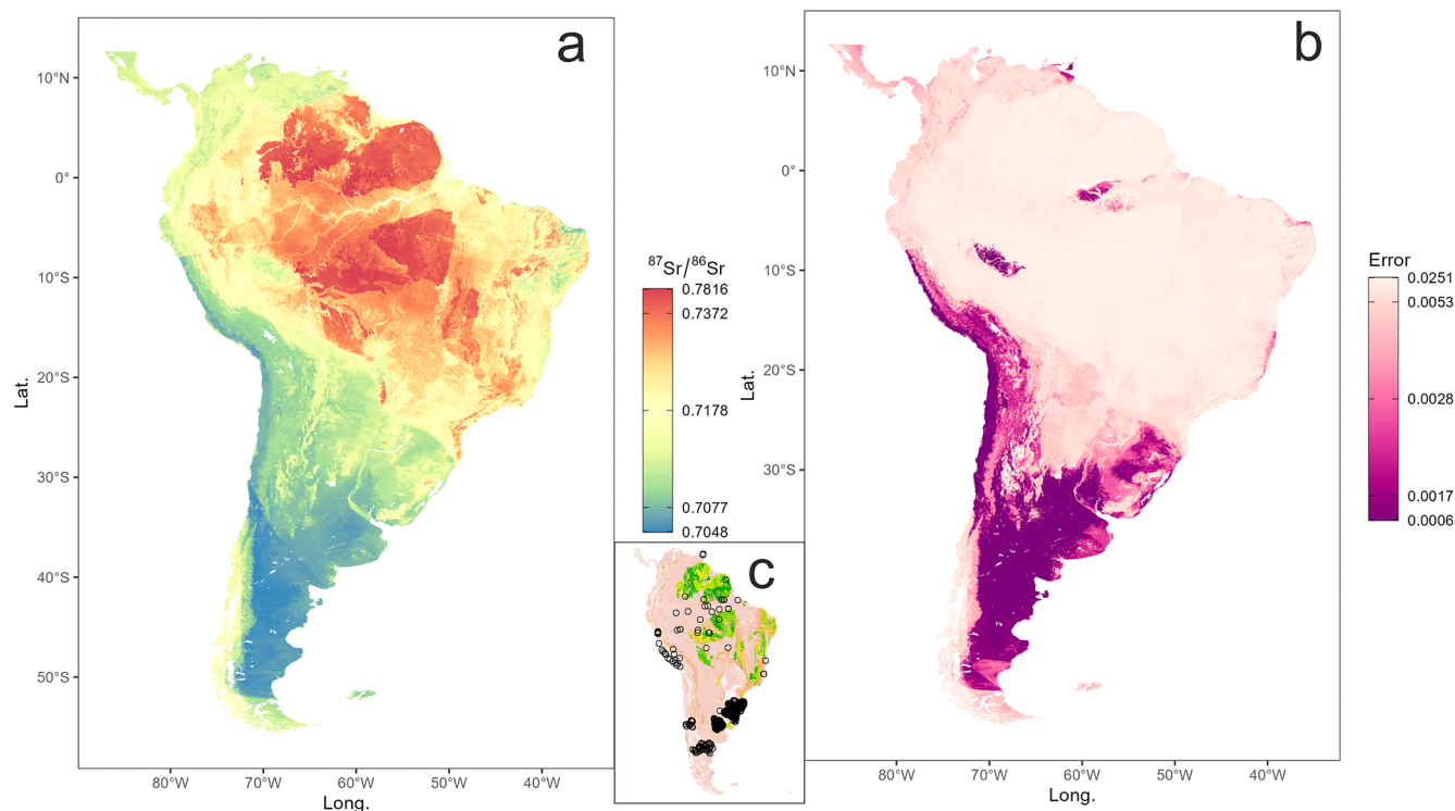
Figure 4. Spatial distribution of strontium isotopes in South America based on plant + lichen samples ( n = 531 sites). Isoscape random forest model (a), associated spatial uncertainty map (b) and sample distribution (c).
