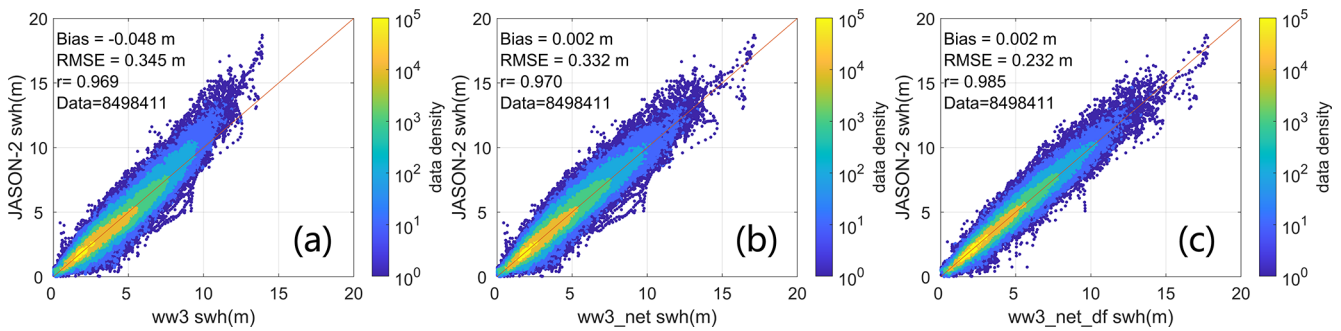
Figure 3. Evaluation of the fused dataset using Jason-2 as an independent reference in 2011. (a) Comparison between the original WW3-ST6 hindcast and Jason-2. (b) Results after applying a one-dimensional look-up table correction to WW3-ST6 SWHs using CCI-Sea State data prior to fusion. (c) Comparison between the fused dataset (WW3-ST6 + remaining altimeters) and Jason-2. The fusion substantially reduces the RMSE and improves the correlation compared to both the original and bias-corrected hindcast.
