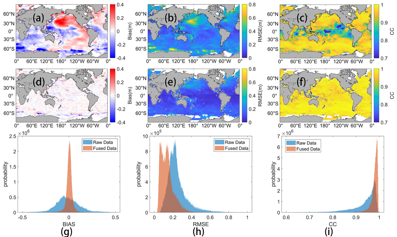
Figure 6. Comparison between WW3-ST6 (forced by ERA5 winds) and WW3-ST4 (forced by CFSR winds) before and after data fusion is applied to both hindcasts using the same altimeter observations in January 2011. (a–c) Maps of bias, RMSE, and CC between the two hindcasts before data fusion. (d–f) Same as (a–c), but after fusion with altimeter observations. (g–i) Probability density functions of grid-point bias, RMSE, and CC, respectively, illustrating the overall improvement in consistency between the two hindcasts after fusion.
