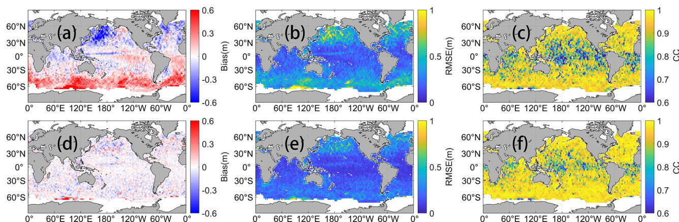
Figure 4. Spatial distributions of SWH error metrics between WW3-ST6 and Jason-2 (a–c) before and (d–f) after fusing SWH data from CCI-Sea State in 2011: (a, d) bias, (b, e) RMSE, and (c, f) CC.
