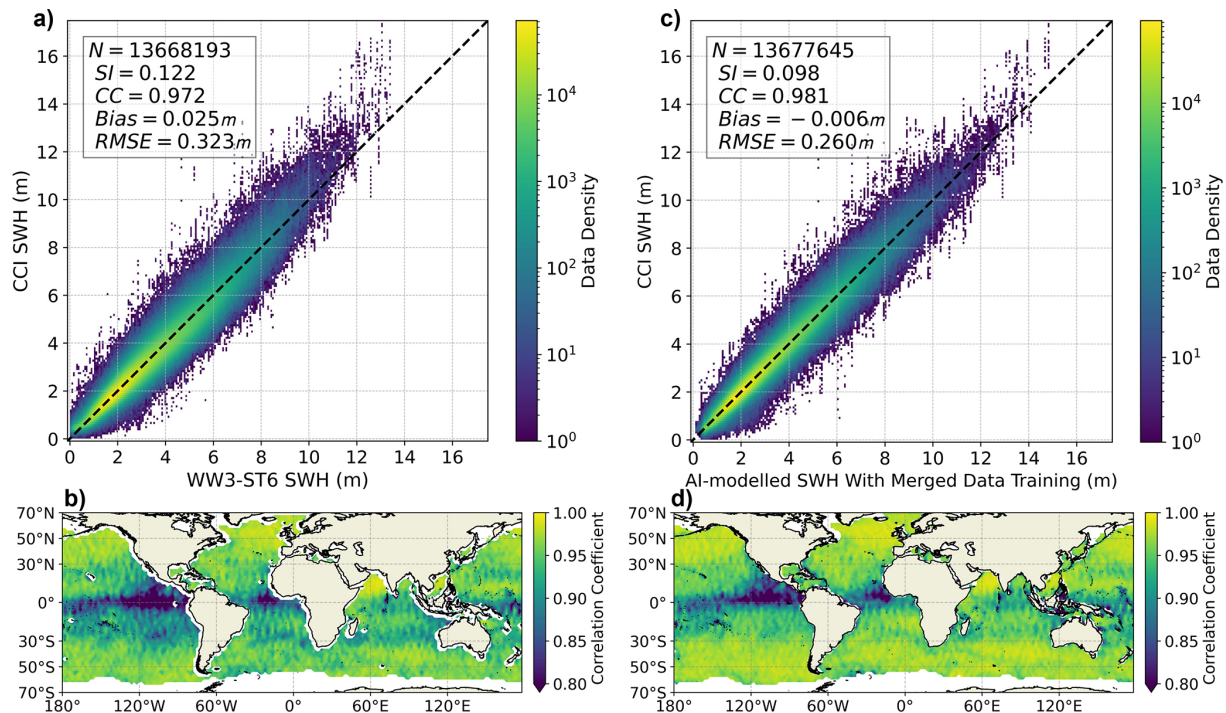
Figure 8. Comparison between SWHs from numerical/AI wave models and CCI-sea state dataset for global ocean in 2020. (a) Scatter plot of SWHs from the NWM versus CCI-sea state. (b) Spatial distributions of CC between SWHs from NWM and CCI-sea state. (c, d) Same as (a) and (b) , respectively, but for the AI wave model trained with ERA5 and subsequently fine-tuned using the 5-year fused dataset. Note that the year 2020 is excluded from the model training.
