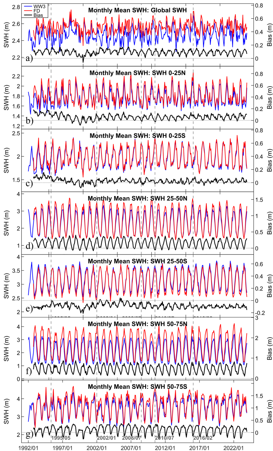
Figure 5. Time series of monthly mean SWH from the WW3-ST6 hindcast background (blue), the “two-sat” fused dataset (red), and the fused-minus-background difference (black) during 1992–2023: (a) the global ocean, (b) 0–25° N, (c) 0–25° S, (d) 25–50° N, (e) 25–50° S, (f) 50–75° N, and (g) 50–75° S. Vertical dashed lines indicate the major satellite-transition times in the two-satellite configuration, as shown in Table 1.
