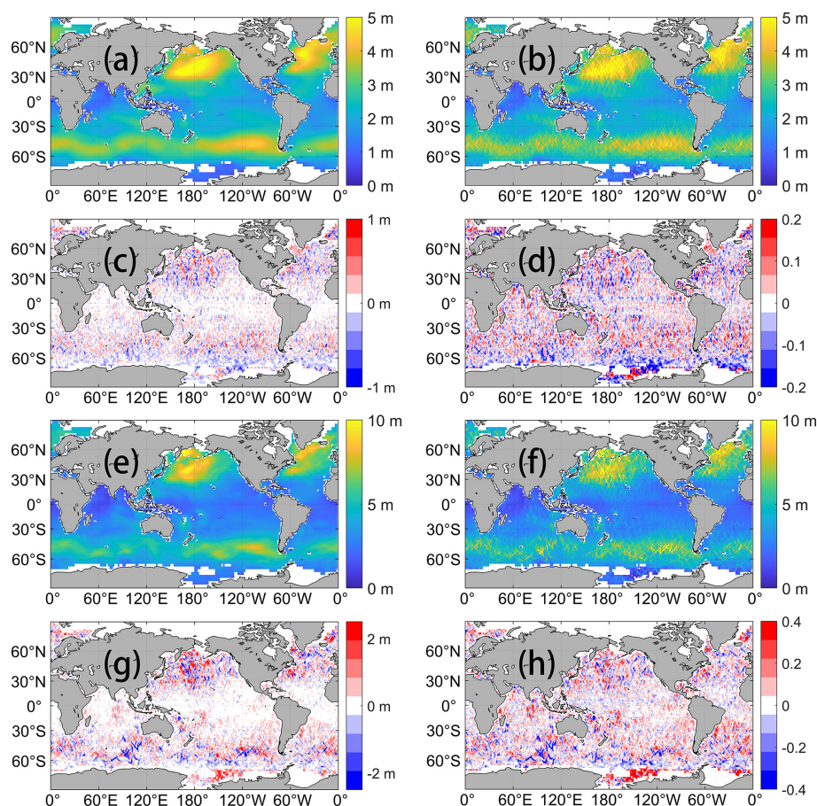
Figure 7. Global distributions of the monthly mean SWH in January 2011 derived from (a) the fused dataset and (b) the original CCI-Sea State L4 dataset, as well as their (c) absolute difference and (d) relative difference. Panels (e) and (f) show the corresponding global distributions of the 95th percentile SWH during the same period derived from (e) the fused dataset and (f) the original CCI-Sea State dataset, as well as their (g) absolute difference and (h) relative difference.
