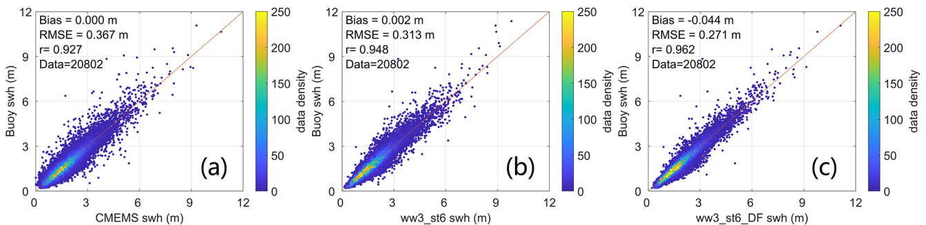
Figure 2. Scatter plots comparing SWHs from buoy observations with those from (a) the CMEMS (Copernicus Marine Environment Monitoring Service) gridded dataset, (b) the WW3-ST6 dataset, and (c) the fused dataset (“two-sat” version) for instantaneous values at 12:00 UTC during the period 2010–2016. All gridded datasets were bilinearly interpolated to the buoy locations.
