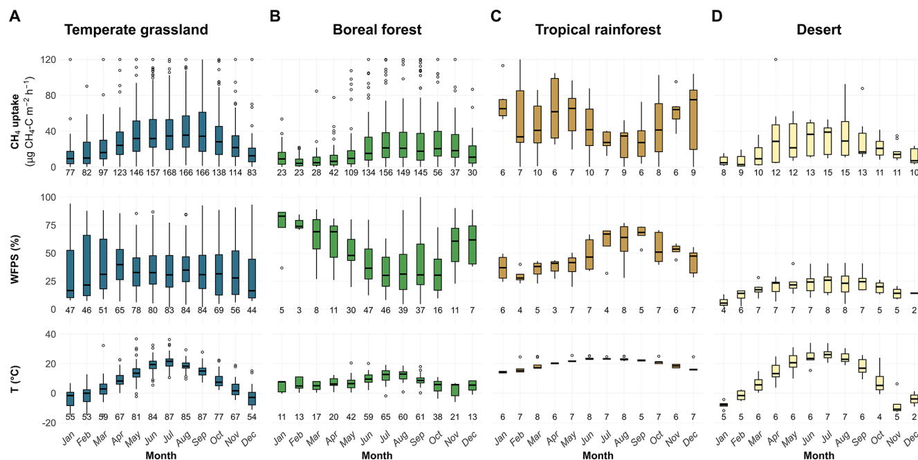
Figure 5. Intra-annual variations of SMU, soil moisture (expressed as WFPS, water-filled pore space), and soil temperature ( T ) across biomes in the Northern Hemisphere. The black lines indicate the median SMU for each biome. The count of flux values in each month is labeled beneath the x -axis ticks. The biomes were grouped into four categories: (A) temperature-dominated, (B) moisture-dominated, (C) jointly controlled, (D) no clear dominant control, based on the covariation of SMU with soil moisture and soil temperature.
