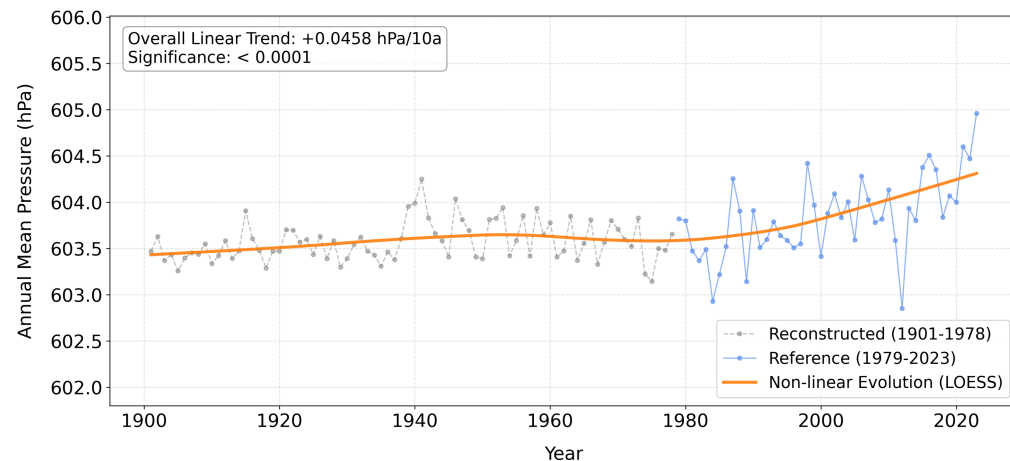
Annual Mean Time Series with Non-linear Trend for Pressure
