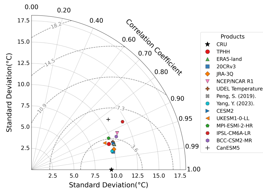
(b) Ref: CRU (Temp)
