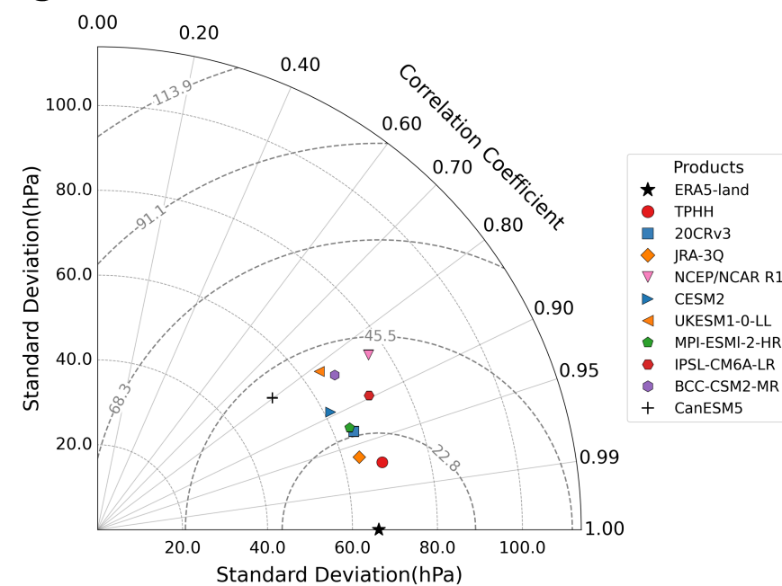
(g) Ref: ERA5 (Pres)
