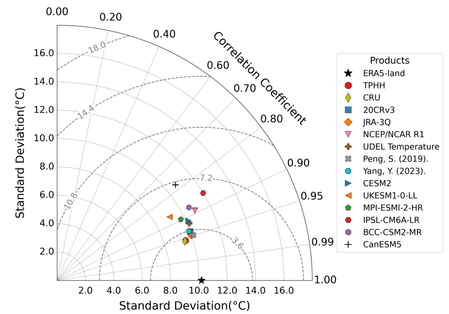
(c) Ref: ERA5 (Temp)
