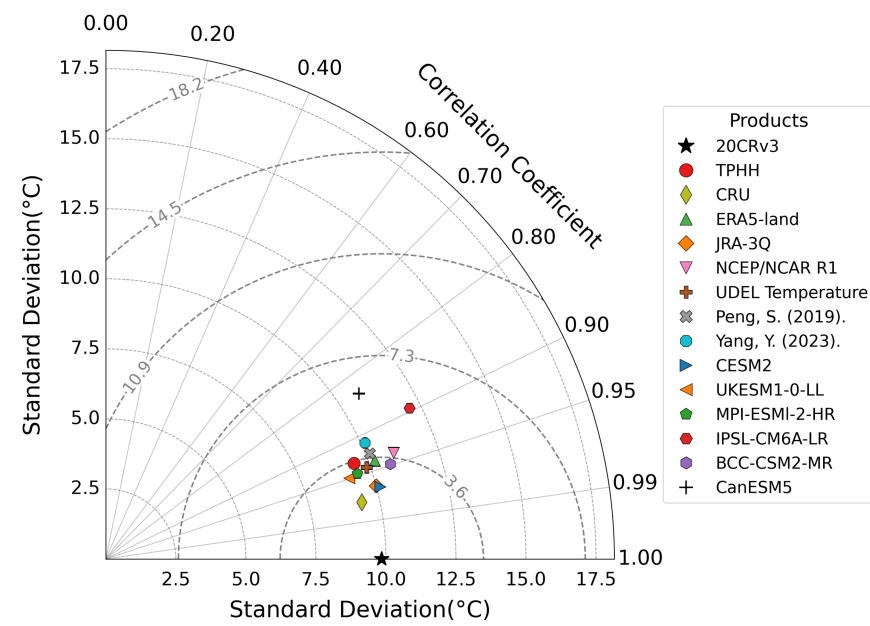
(a) Ref: 20CRv3 (Temp)
