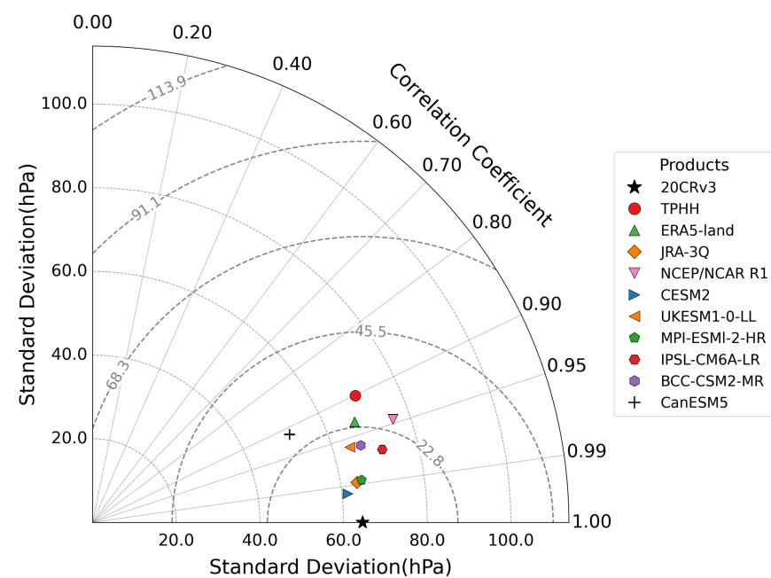
(f) Ref: 20CRv3 (Pres)
