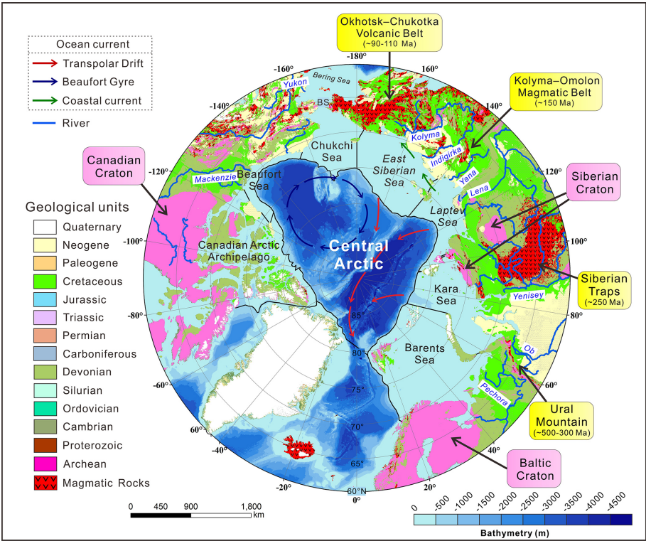
Figure 1. Overview map of the Arctic Ocean illustrating regional subdivisions and circum-Arctic lithological frameworks. The study area is divided into the central Arctic Ocean and the Arctic marginal seas. The geological background is adapted from Harrison et al. (2011). Major magmatic and volcanic belts and cratons (Akinin et al., 2020) are indicated by arrows and annotated with colored boxes. BS denotes the Bering Strait. Major surface ocean circulation pathways are denoted by colored arrows, where red arrows indicate the Transpolar Drift, dark blue arrows indicate the Beaufort Gyre, and green arrows denote regional coastal currents (Timmermans and Marshall, 2020).
