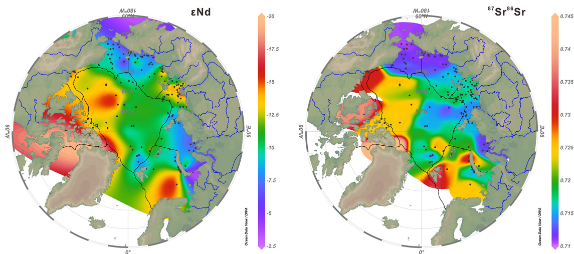
Figure 2. Spatial distribution of \epsilon\text{Nd} and ^{87}\text{Sr}/^{86}\text{Sr} in surface sediments of the Arctic Ocean. Note that some marginal parts of the distribution maps do not contain data points but are the result of extrapolation by the Ocean Data View software.
