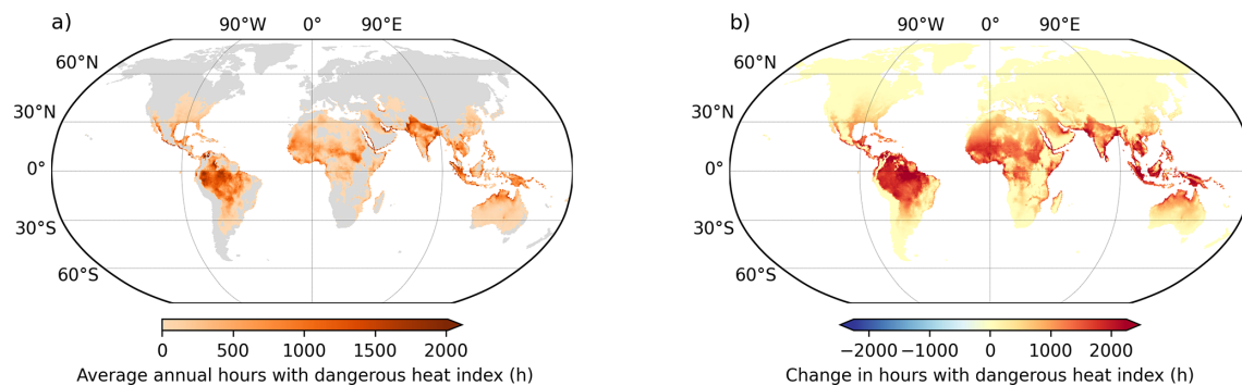
Figure 2. (a) Average annual number of hours with a “dangerous” heat index above 103 °F (39.4 °C) in 1981–2010 based on the MPI-ESM. (b) Change of the number of hours until 2071–2100 under SSP370. This analysis is available for the full set of ISIMIP3 climate models and scenarios from Posch and Zabel (2025a).
