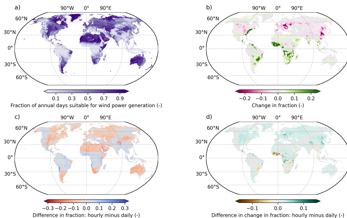
Figure 4. Comparison of the assessment of suitable conditions for wind power generation based on daily and on hourly climate data. (a) Fraction of annual number of days suitable for wind power generation in 1981–2010 based on the daily MPI-ESM data (same color scale as Fig. 3a). (b) Change of the fraction until 2071–2100 under SSP370 based on daily data (same color scale as Fig. 3b). (c) Difference of the fraction in 1981–2010, hourly minus daily. (d) Difference of the projected change, hourly minus daily.
