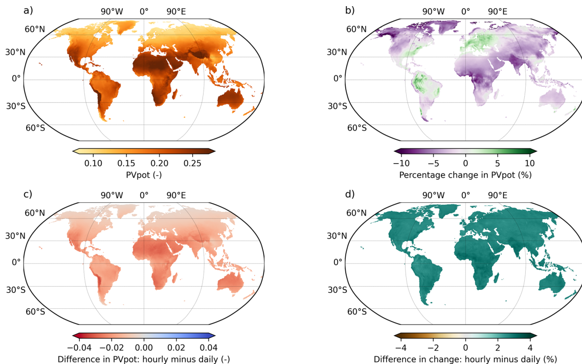
Figure 6. Comparison of the photovoltaic power potential (PV pot ) calculated from daily and from hourly climate data. (a) PV pot in 1981–2010 based on the daily MPI-ESM data (same color scale as Fig. 5a). (b) Percentage change of PV pot until 2071–2100 under SSP370 based on daily data (same color scale as Fig. 5b). (c) Difference of PV pot in 1981–2010, hourly minus daily. (d) Difference of the projected percentage change, hourly minus daily.
