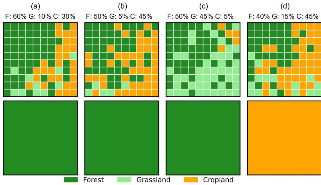
Figure S1. Four hypothetical scenarios (a)–(d) of vegetation composition within a single 0.05° grid cell, comprising varying fractions of 500 m pixels classified as Forest (F), Grassland (G), and Cropland (C).
