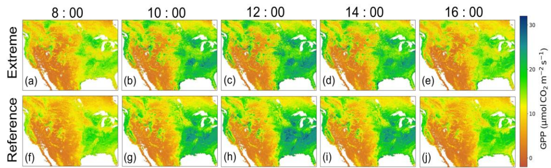
Figure S16. Spatial distribution of GPP in the central North America during June 2021 (a–e), averaged reference year June (f–j).
