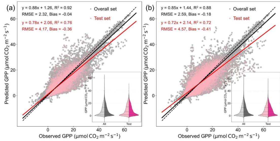
Figure S8. Performance of CKML-GPP of training models (a) with and (b) without aridity index.
