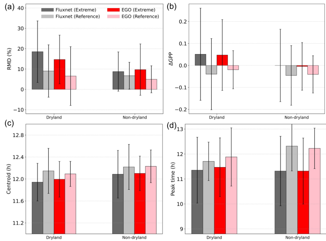
Figure S18. Boxplot of diurnal metrics of site GPP and EGO GPP in dryland and non-dryland in U.S. (a) for RMD, (b) for \Delta GPP , (c) for Centroid and (d) for Peak time.
