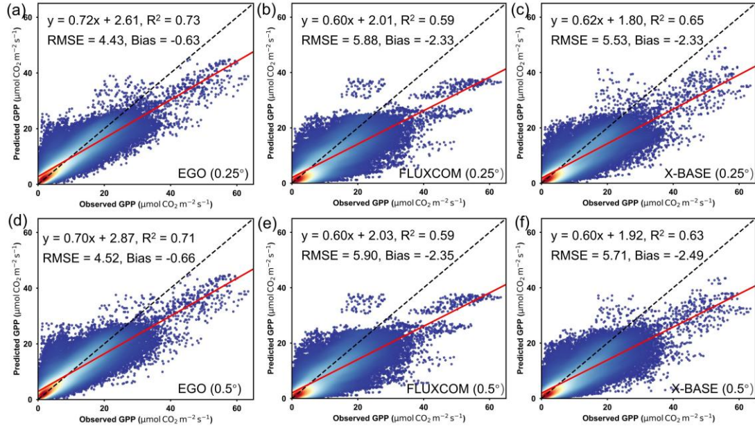
Figure S6. Performance comparison of EGO, FLUXCOM, and X-BASE GPP products against site observations at harmonized spatial resolutions. To ensure a fair comparison, all products were spatially resampled to match specific target resolutions using the bilinear interpolation method. Panels (a)–(c) display the accuracy evaluation when all products are unified to a 0.25° spatial resolution, which is consistent with the native resolution of X-BASE. Panels (d)–(f) present the corresponding performance when all datasets are unified to a 0.5° spatial resolution, consistent with the native resolution of FLUXCOM. The red solid lines represent the linear regression fits, and the black dashed lines denote the 1:1 reference line.
