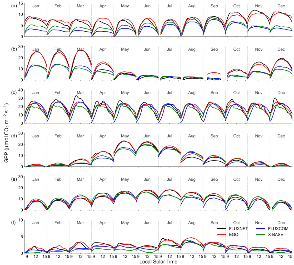
Figure S10. Comparison of diurnal GPP dynamics between site observations and products across diverse biomes for each month of the year. Panels (a)–(f) illustrate the multi-year average diurnal GPP variations across different months at six representative flux sites: (a) savannas (AU-Gin), (b) grassland (AU-DaP), (c) broadleaf forest (BR-Sa3), (d) cropland (DE-Kli), (e) needleleaf forest (US-Blo), and (f) shrubland (US-SRC). The black solid lines represent the in-situ FLUXNET observations. The colored lines denote the estimations from different global hourly GPP products: EGO (red), FLUXCOM (blue), and X-BASE (green).
