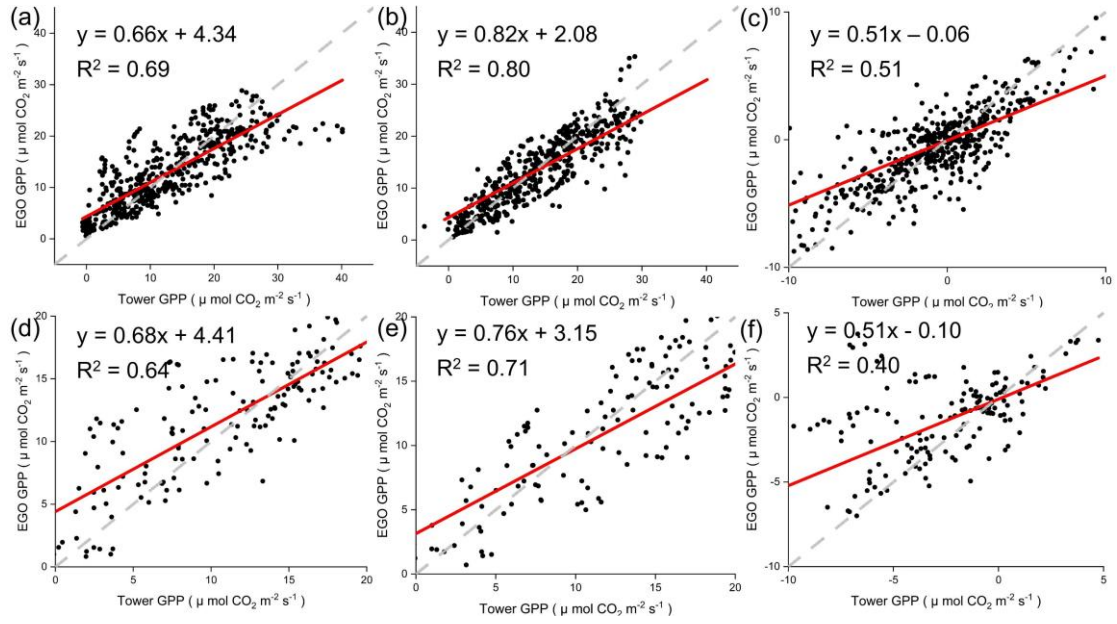
Figure S17. The fitting accuracy of EGO GPP with the corresponding 39 sites GPP in U.S. in (a) June 2021, (b) June of reference year, and (c) anomaly GPP. Similarly, 12 sites GPP in Europe in (d) August 2003, (e) August of reference year, and (f) anomaly GPP.
