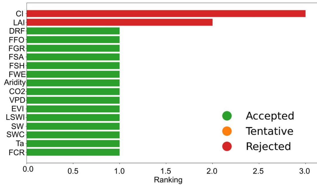
Figure S2. Boruta feature selection. The CI (clumping index) and LAI (leaf area index) were discarded due to their lower importance than shadow feature (Red legend).
