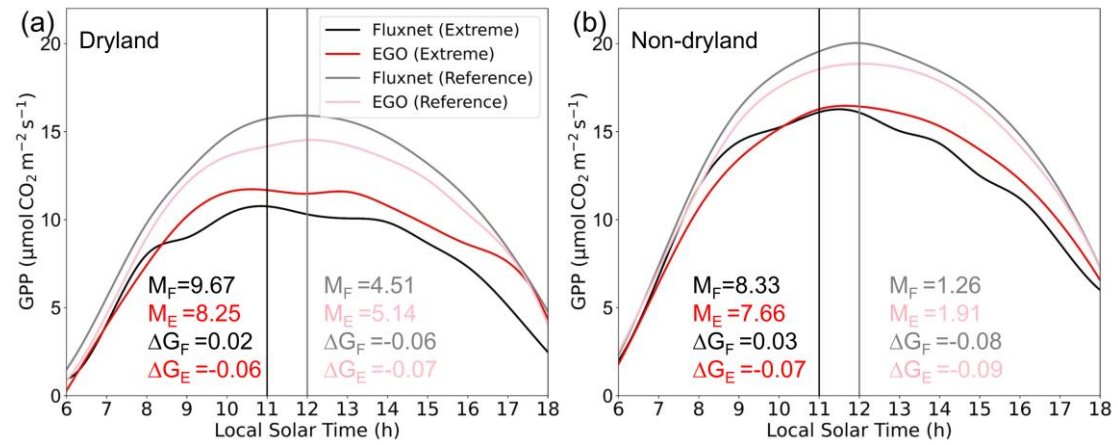
Figure S21. Mean diurnal GPP cycles aggregated for (a) dryland and (b) non-dryland sites in the European. Black and red lines denote average GPP cycles for August 2003, while gray and pink lines represent averaged years for August (Reference). The vertical line represents the peak time. M and \Delta G indicate RMD and \Delta GPP ; F and E denote flux-tower observations and EGO GPP, respectively. Dark and light colors correspond to 2003 and reference-year metrics.
