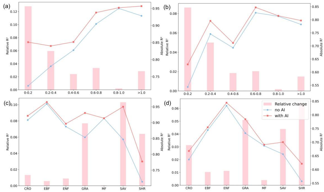
Figure S9. Relative improvement of R^2 across (a,b) aridity gradients and (c,d) vegetation types when incorporated aridity index into predictor. Red and blue line represented the evaluation metrics with and without aridity index. Pink bar was relative change. (a, c) for training set, and (b, d) for test set.
