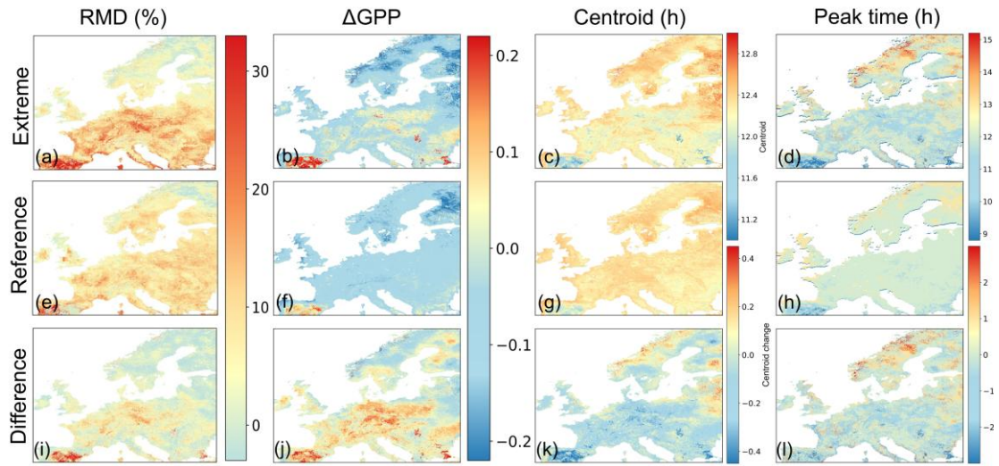
Figure S22. Spatial pattern of the diurnal metrics in the European during August 2003 (a-d) and averaged normal year August (e-h), with (i-l) showing their differences (extreme–normal).
