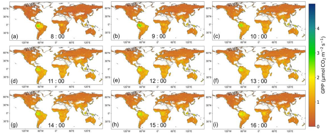
Figure S13. Global diurnal pattern of standard deviation of hourly GPP of EGO at 1-hour intervals of local solar time.
