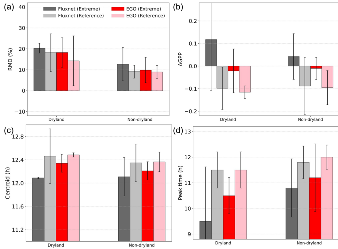
Figure S23. Boxplot of diurnal metrics of site GPP and EGO GPP in dryland and non-dryland in European. (a) for RMD, (b) for \Delta GPP , (c) for Centroid and (d) for Peak time.
