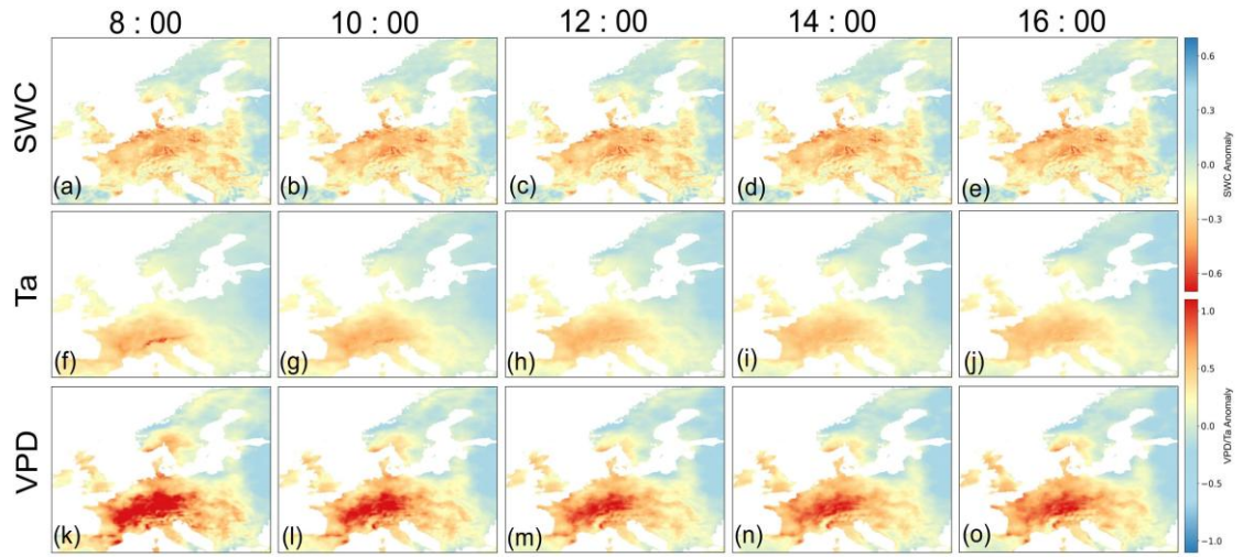
Figure S19. Spatial distribution of anomaly of SWC (a-e), Ta (f-j) and VPD (k-o) in the European during August 2003.
