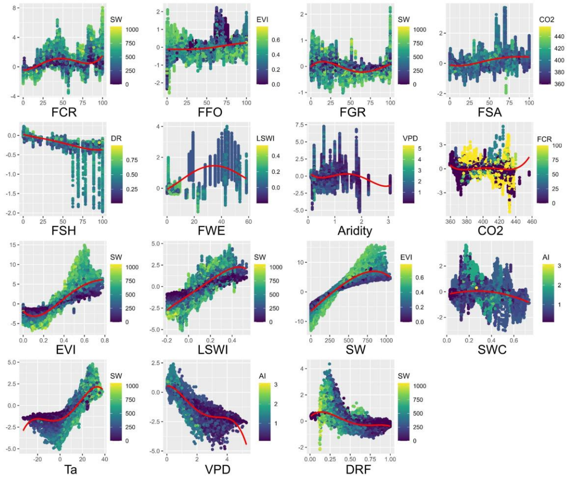
Figure S7. Interaction between each driver and their corresponding SHAP values.
