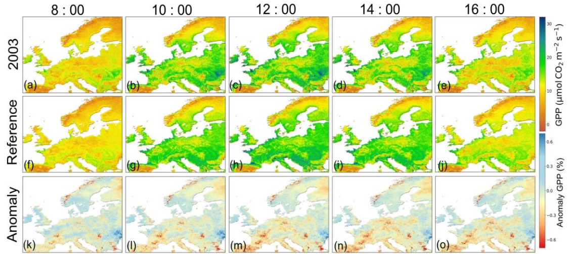
Figure S20. Spatial distribution of GPP in the European during August 2003 (a–e), averaged normal year August (f–j), and their anomalies (k–o). Anomaly = (\text{GPP}_{2003} - \text{GPP}_{\text{normal}}) / \text{GPP}_{\text{normal}} .
