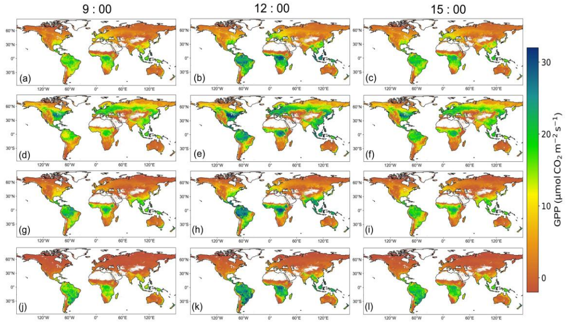
Figure S12. Global diurnal pattern of EGO GPP from 2000 to 2022 in different seasons. (a-c) for March to May, (d-f) for June to August, (g-i) for September to November, and (j-l) for December to February.
