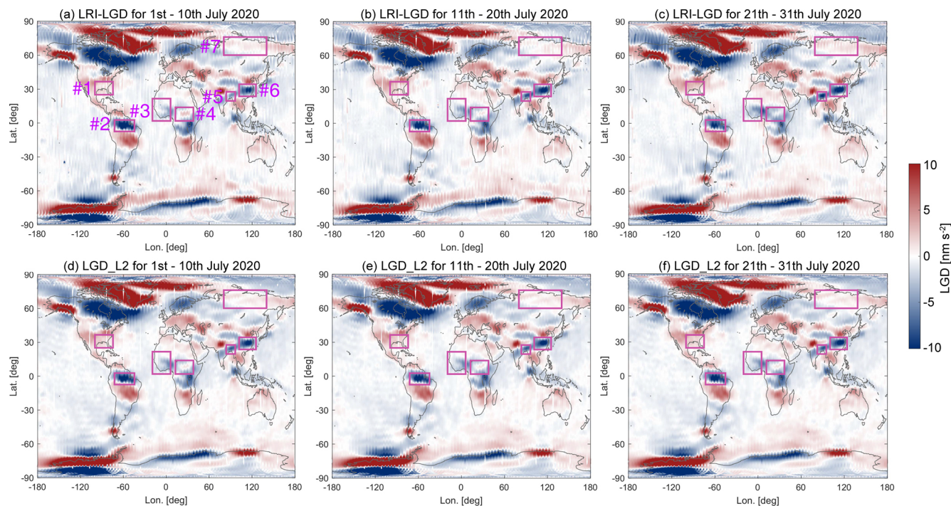
Figure 7. Global LGD maps at a 10 d interval during July 2020. The top row (panels a–c) shows LRI-LGD results, and the bottom row (panels d–f) shows LGD_L2 results. Each column corresponds to early, mid, and late July, respectively. In panel (a), purple rectangles mark regions with evident intra-month variations. Regions #1–#7 correspond the southeastern United States, Amazon basin, western Africa, South Sudan, Bangladesh, Yangtze River basin, and northern Russia.
