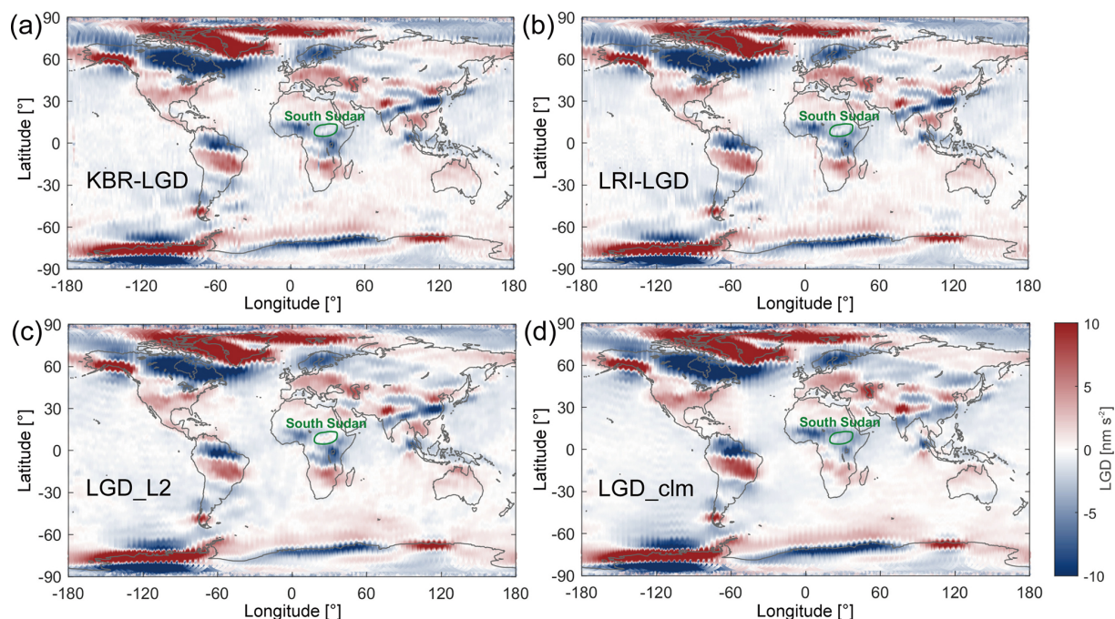
Figure 6. Global maps of LGD and water mass changes for July 2020. Panels (a)–(d) show LGD derived from KBR, LRI, L2 data, and climatology, respectively. Note that KBR-LGD, LRI-LGD, LGD_L2, and LGD_clm contain signals with frequencies below 20, 10, 10, and 10 mHz, respectively.
