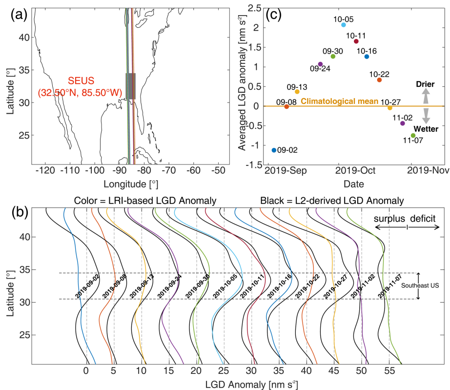
Figure 10. LGD analysis of the flash drought event in the SEUS from September to November 2019. (a) Study region (gray box) centered at 32.5° N, 85.5° W. Colored lines represent GRACE-FO ground tracks intersecting the region during September–early November. (b) Along-track LGD anomalies for each satellite pass, with colored lines denoting LRI-based anomalies (LRI-LGD minus climatological LGD) and black lines showing L2-derived anomalies (LGD_L2 minus climatological LGD) for comparison. Negative LGD anomalies indicate wetter-than-normal conditions, while positive anomalies indicate drier-than-normal conditions. (c) Averaged LGD anomalies over the SEUS through weighted averaging.
