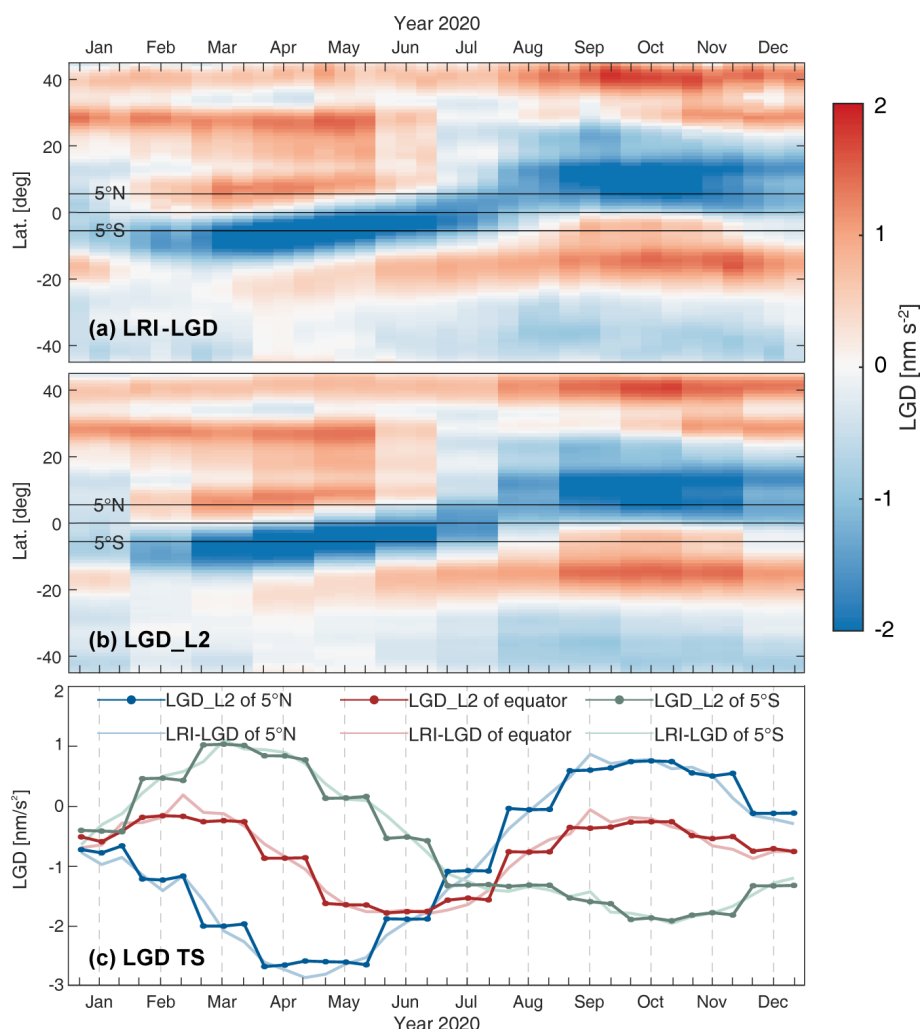
Figure 8. Zonally averaged LGD time series across 45^{\circ}\text{S} – 45^{\circ}\text{N} for 2020, derived from the global LGD maps at a 10 d interval shown in Fig. 7. Panels (a) and (b) present results from LRI-LGD and LGD_L2, respectively. Horizontal lines indicate the selected latitudes for which the LGD time series are presented in panel (c). In panel (c), dark lines represent LGD_L2 time series, and light lines represent LRI-LGD time series.
