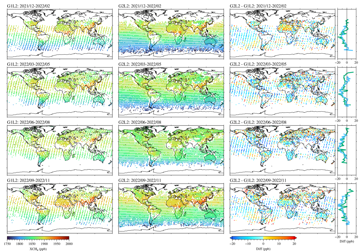
Figure 4. Three-month averaged \text{XCH}_4 distributions for G1L2 (left) and G2L2 (center) from December 2021 to November 2022, and their differences (G2L2–G1L2) (right). Color scales represent \text{XCH}_4 concentrations (ppb) for G1L2 and G2L2, and differences in ppb for the bottom panels. The rightmost panels additionally show latitudinal mean differences (ppb), with blue and green lines indicating ocean and land regions, respectively.
