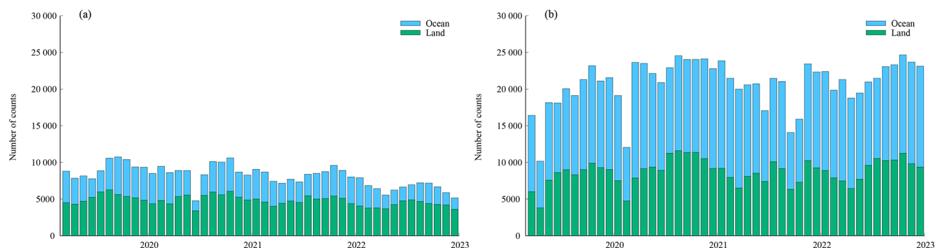
Figure 1. Monthly count of XCH 4 observations meeting the quality criteria for (a) TANSO-FTS and (b) TANSO-FTS-2 in March 2019 and December 2022. Blue and green bars represent observations over ocean and land, respectively.
