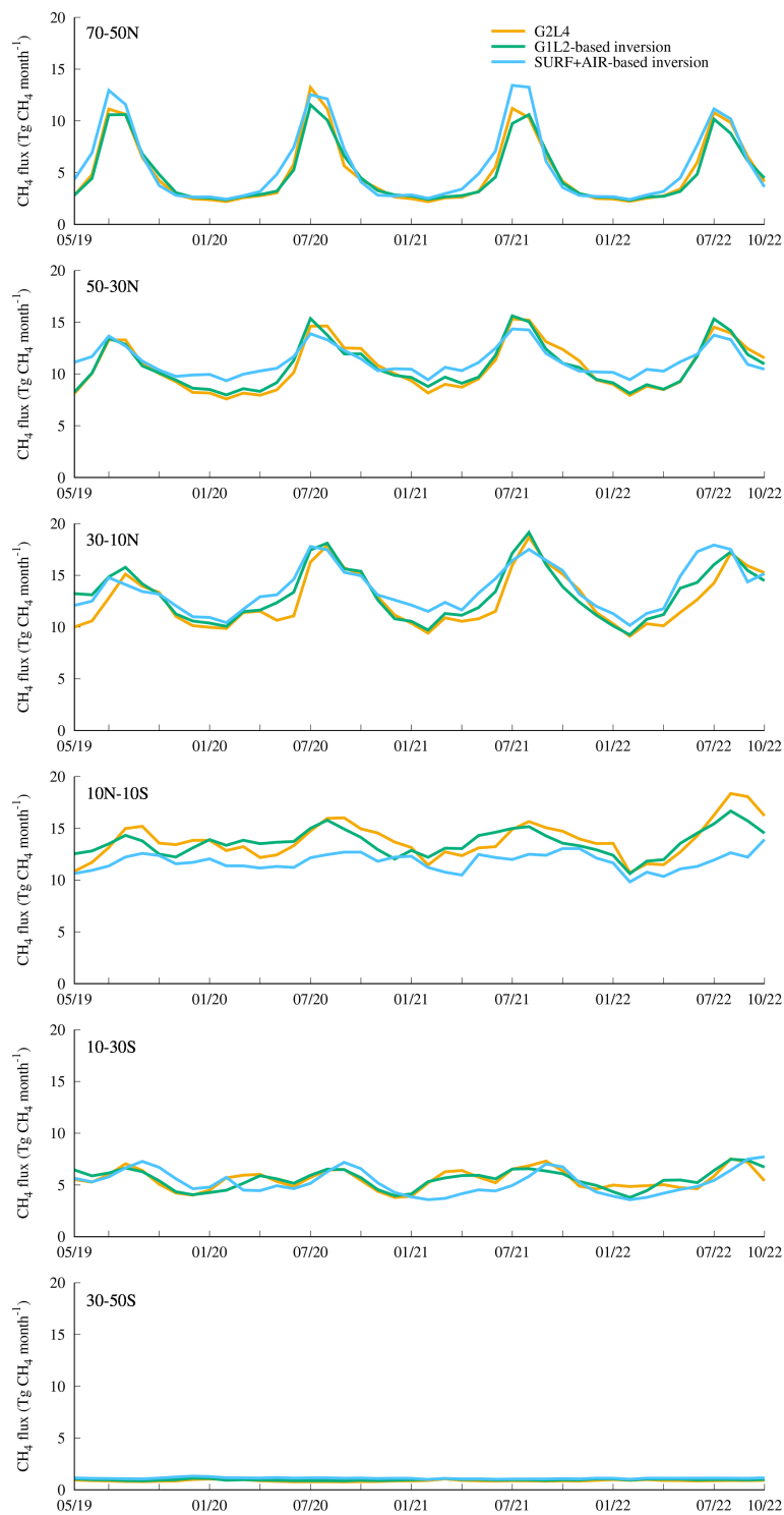
Figure A2. Same as Fig. 6, but showing monthly \text{CH}_4 flux variations ( \text{Tg CH}_4 \text{ month}^{-1} ) estimated from G2L4 (orange), GIL2-based inversions (green), and ground-based inversions (blue).
