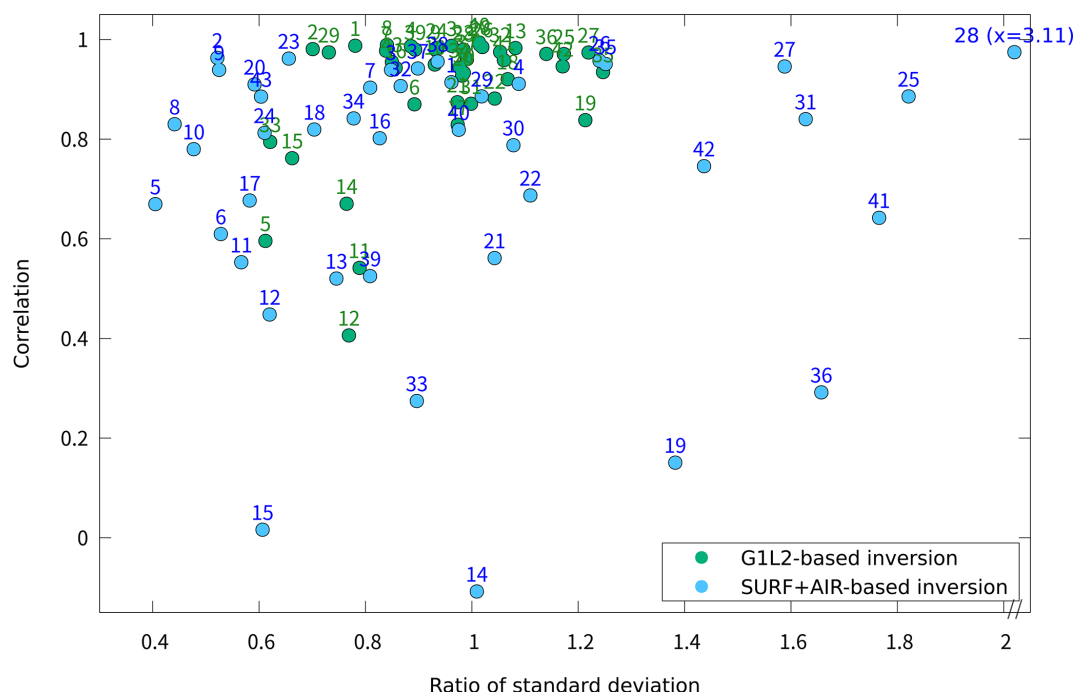
Figure 8. Correlation coefficients versus ratio of standard deviations for seasonal \text{CH}_4 flux variations across 42 land regions. Ratios are computed as the standard deviation of G1L2-based or ground-based (SURF+AIR) inversion divided by that of G2L4, and correlations are calculated between G2L4 and each of other two inversions.
