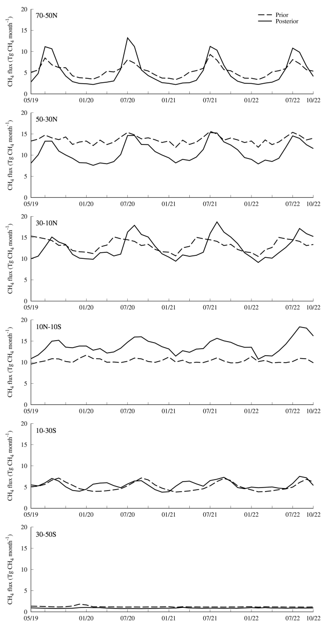
Figure 6. Monthly \text{CH}_4 flux variations ( \text{Tg CH}_4 \text{ month}^{-1} ) for six latitude bands between 70^\circ \text{N} and 50^\circ \text{S} , estimated from prior (broken line) and posterior (solid line) fluxes for May 2019–October 2022.
