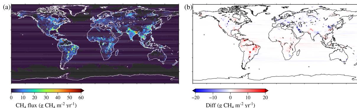
Figure 5. Spatial distribution of (a) annual posterior CH 4 fluxes for 2021 and (b) posterior-minus-prior differences (g CH 4 m -2 yr -1 ).
