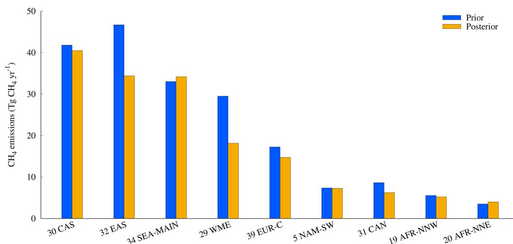
Figure 9. Anthropogenic CH 4 emissions (Tg CH 4 yr -1 ) for nine regions – NAM-SW, AFR-NNW, AFR-NNE, WME, CAS, CAN, EAS, SEA-MAIN, and EUR-C – where anthropogenic sources in the a priori estimates account for more than 80 % of prior fluxes. Bars show prior (blue) and posterior (orange) estimates derived from GOSAT-2 Level 4 product for 2020–2021.
