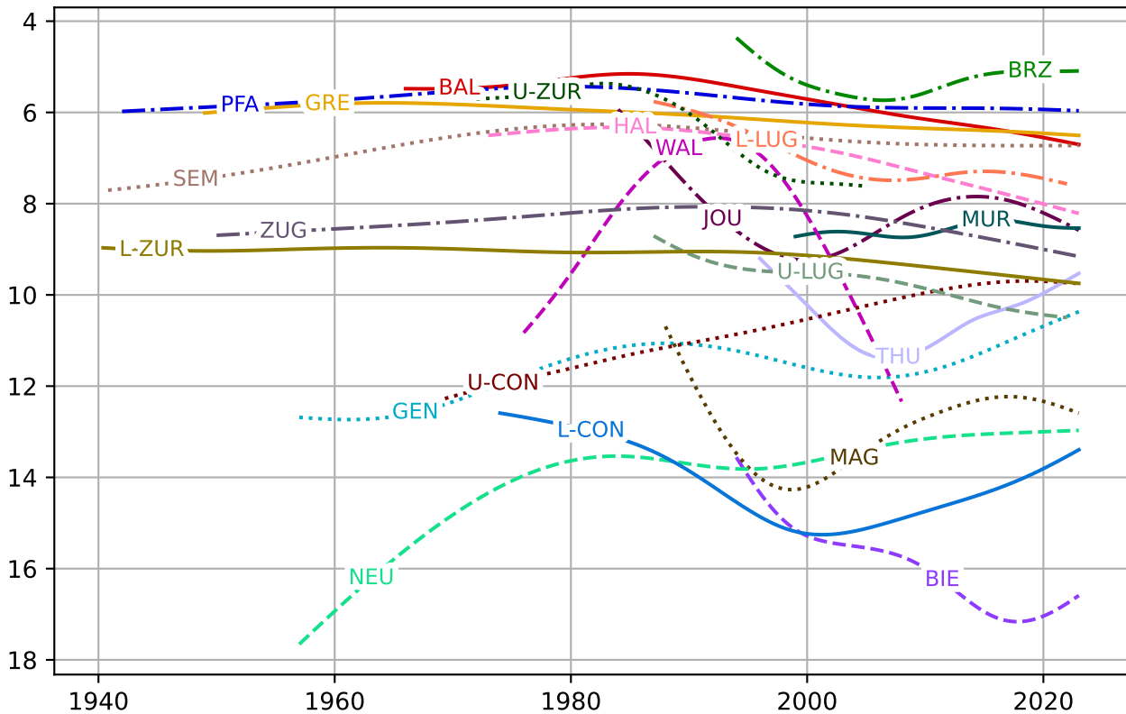
Mean summer thermocline depth (m)
