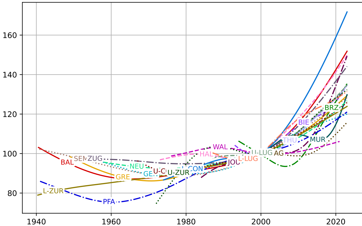
Mean autumn Schmidt stability (%)
