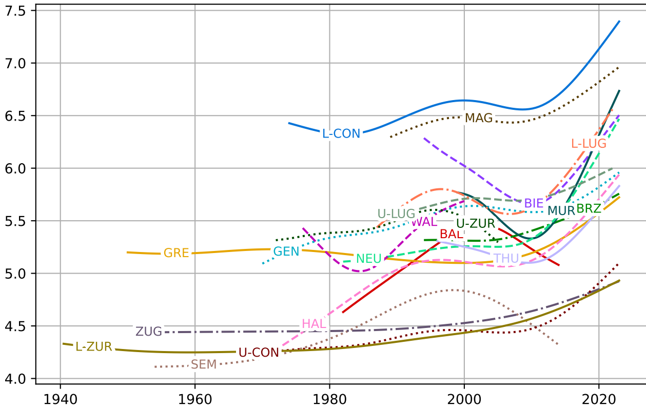
Mean annual bottom temperature (°C)
