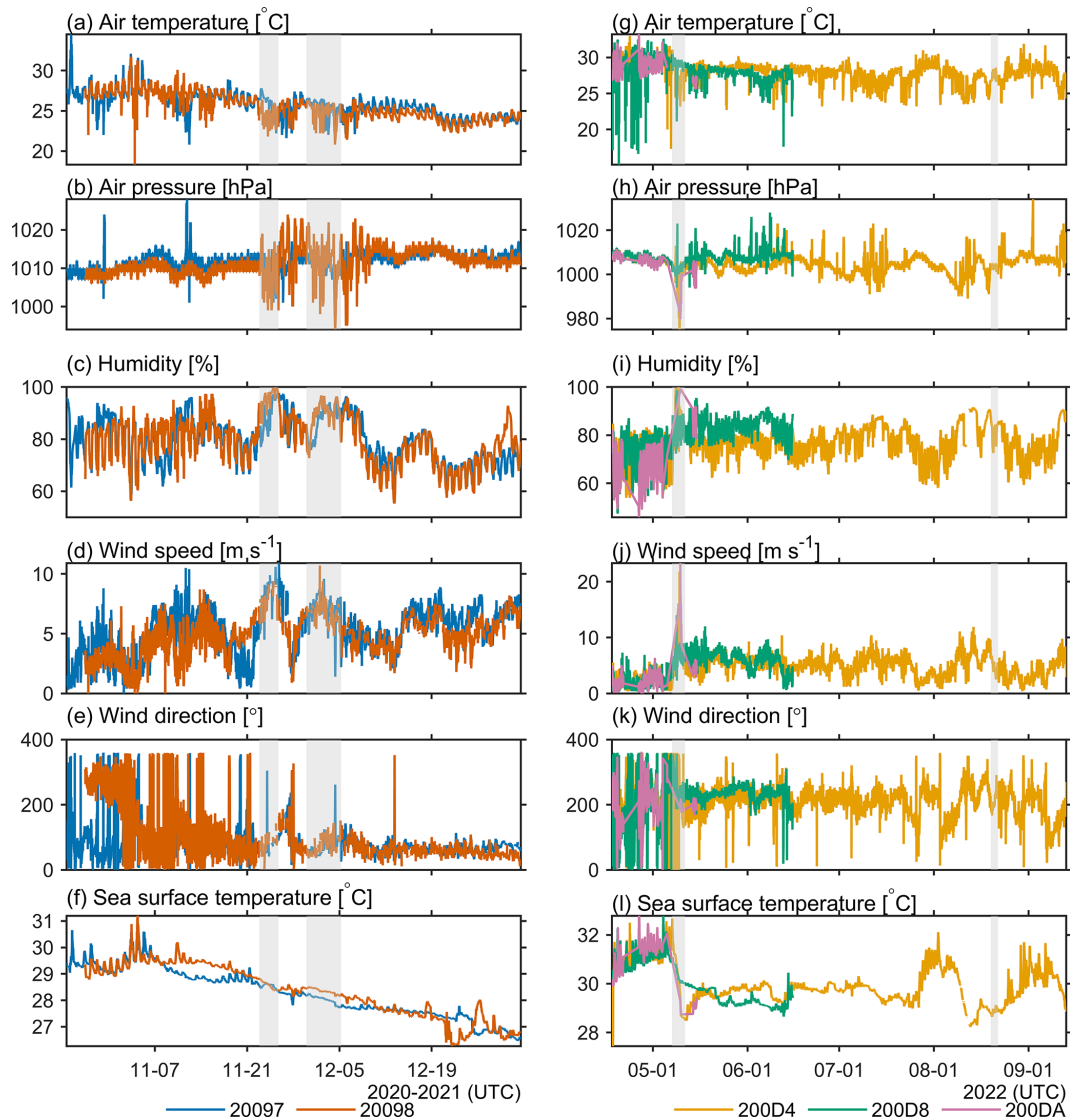
Figure 4. Time series of observed meteorological and oceanic parameters. “Left-column panels show data for buoys 20097 (blue) and 20098 (orange); right-column panels show buoys 200D4 (yellow), 200D8 (green), and 200DA (pink). Gray-shaded areas indicate TC passages: Nivar and Burevi (left), and Cyclonic Storm Asani and Tropical Depression Four (right) in chronological order from left to right. Panels show: (a, g) air temperature, (b, h) sea-level pressure, (c, i) relative humidity, (d, j) wind speed, (e, k) wind direction, and (f, l) SST.
