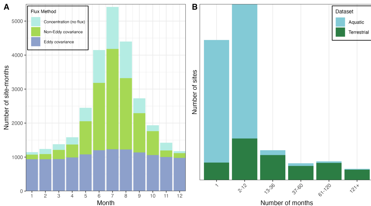
Figure S6. A) The number of observations by measurement method distributed across months. B) The number of sites by the number of total site-month observations for each site separated by aquatic and terrestrial datasets.
