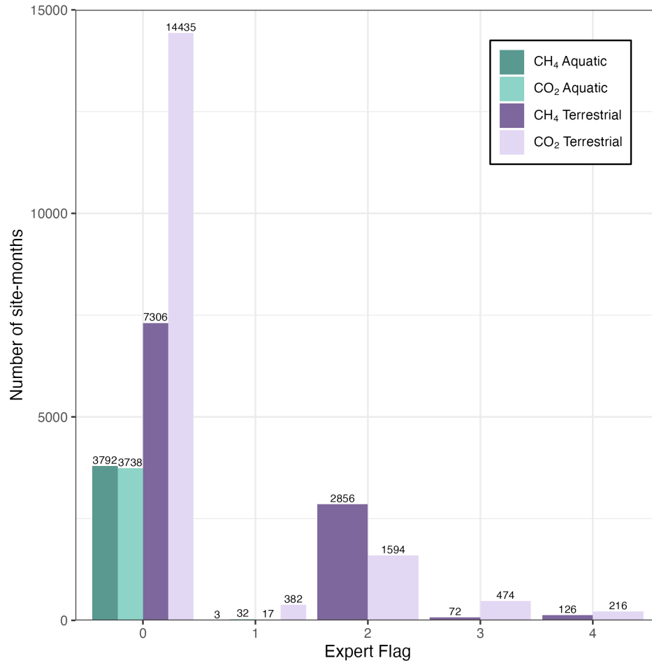
Figure S4. The number of site-months flagged with the 4 different expert flags across CO 2 fluxes (NEE, GPP, Reco) and CH 4 fluxes (flag 0 = data was not flagged). For CO 2 , the flags considered fluxes outside the 1st and 99th percentiles for terrestrial, and outside the 99th percentile for aquatic data (flag 1). For CH 4 , flag 1 points to terrestrial sites with fluxes higher than 30 g C m -2 month -1 , and to lentic sites with higher CH 4 diffusion fluxes. Flags 2 to 4 refer to both gas species and only terrestrial sites. Monthly fluxes based on sporadic non-eddy covariance measurements were marked with flag 2, eddy covariance data with long periods of entirely gap-filled data with flag 3, and sites that do not represent typical conditions across the Arctic-boreal region with flag 4 (Table 4).
