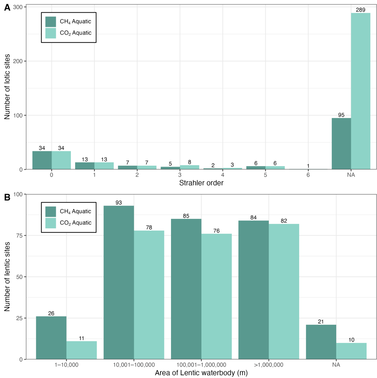
Figure S7. Number of unique lotic sites for each Strahler order for CO 2 and CH 4
