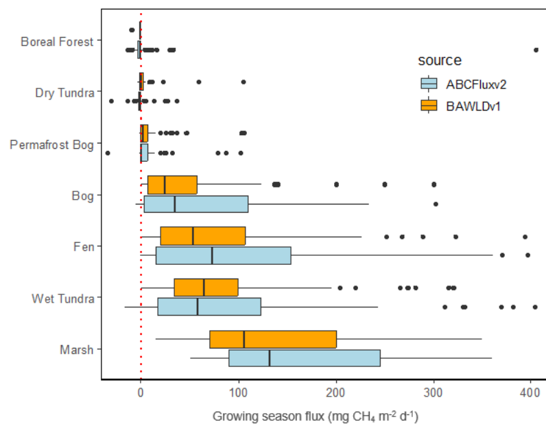
Figure S14. Comparison of terrestrial CH 4 fluxes in ABCFlux v2 vs BAWLD-CH 4 v1. Fluxes from ABCFlux v2 represent the average fluxes between June and August.
