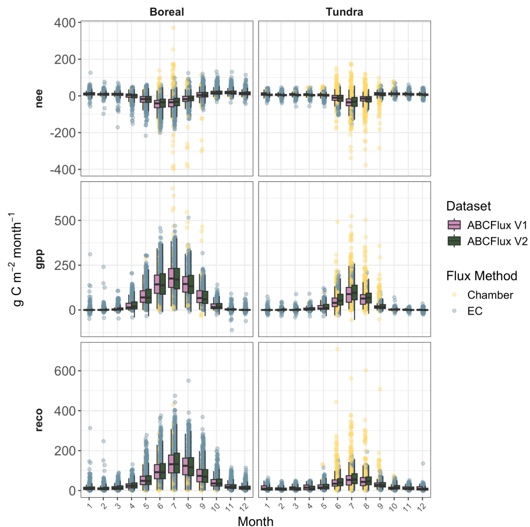
Figure S12. Comparison of monthly terrestrial CO 2 flux magnitudes in ABCFluxv1 vs. v2. GPP was presented as a negative flux in ABCFlux v1 but was converted to positive for the purpose of this comparison.
