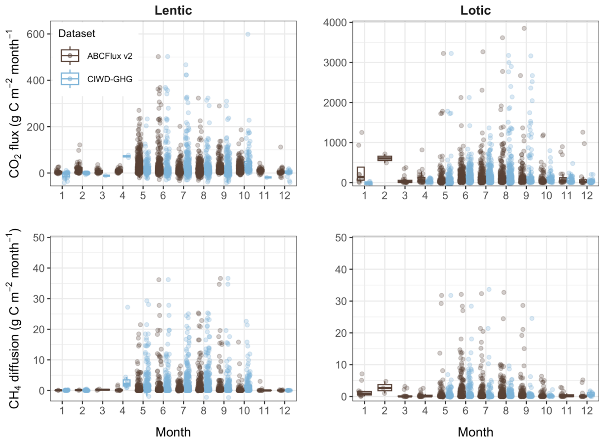
Figure S13. Comparison of monthly cumulative carbon fluxes (CO 2 and diffusive CH 4 flux) for aquatic ecosystems between this study (ABCFlux v2, grey) and Song et al. (2024; CIWD-GHG, blue).
