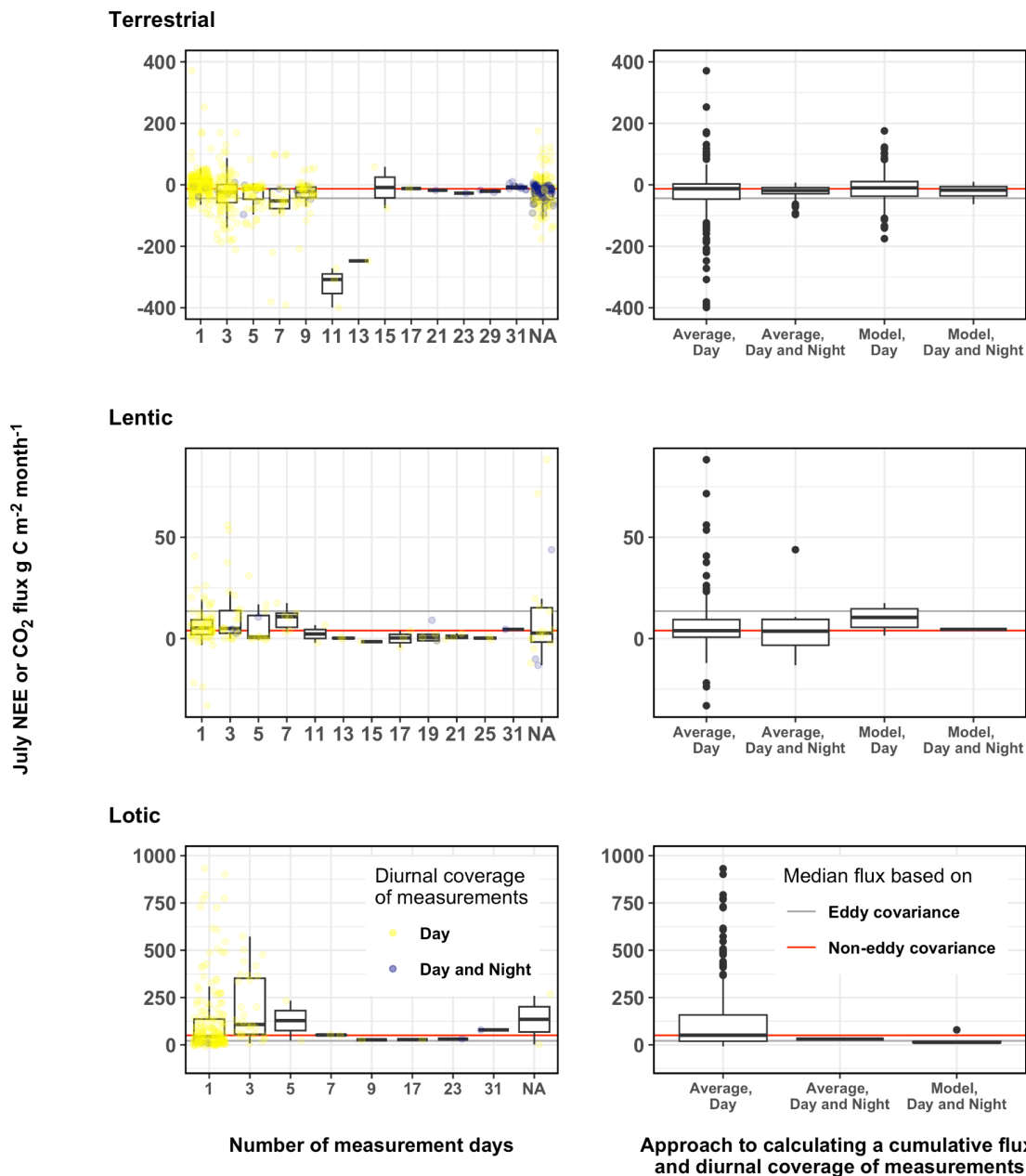
Figure S2. The relationship between chamber-based net CO 2 flux for July and the number of measurement days, diurnal coverage, and the method used to calculate cumulative fluxes across key ecosystems. "Terrestrial" refers only to treeless ecosystems. When information on diurnal coverage was unavailable, we assumed daytime-only measurements for this visualization. Similarly, in the absence of details on the aggregation approach, we assumed a simple average was used—that is, the mean measured flux multiplied by the number of days, rather than modeled using light and temperature response functions.
