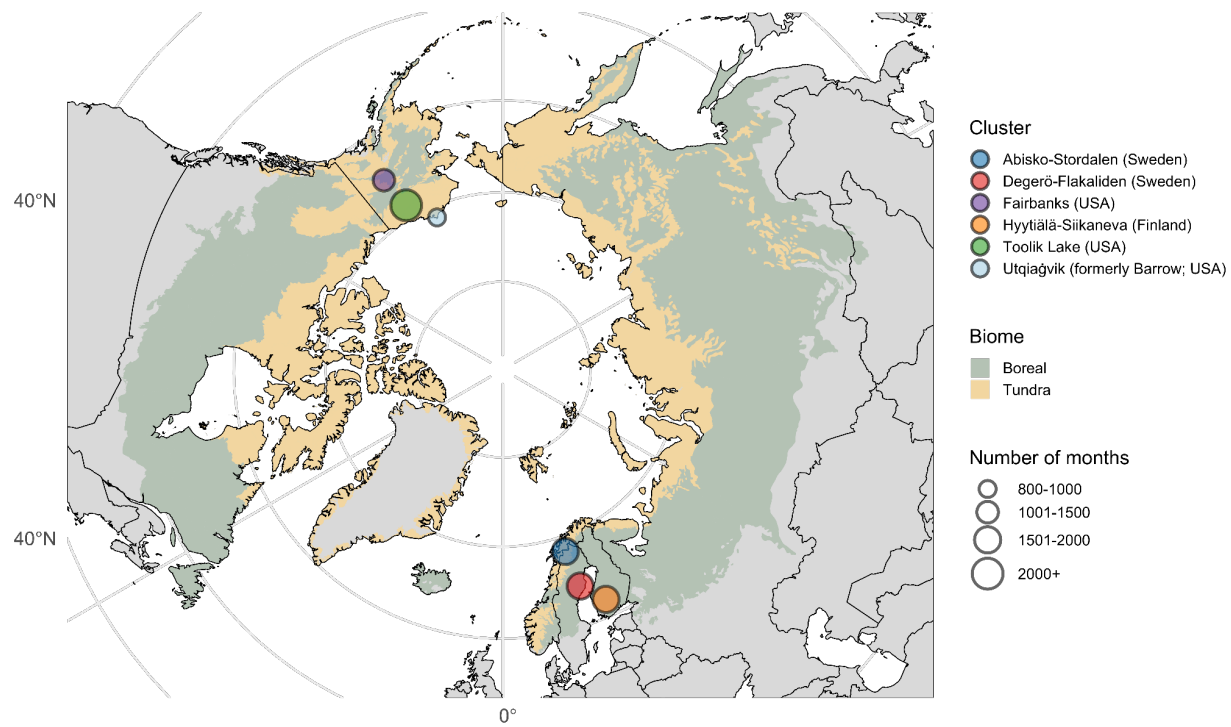
Figure S11. Cluster sites identified by more than 800 site-months within 30km radius.
