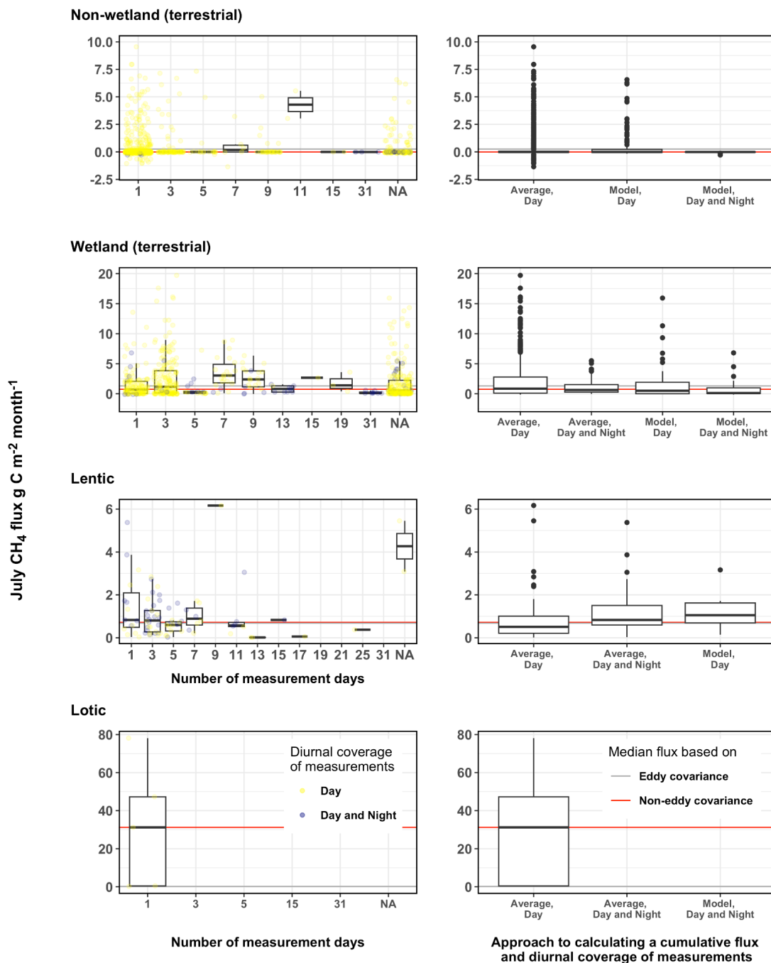
Figure S3. The relationship between chamber-based net CH 4 flux for July and the number of measurement days, diurnal coverage, and the method used to calculate cumulative fluxes across key ecosystems. When information on diurnal coverage was unavailable, we assumed daytime-only measurements for this visualization. Similarly, in the absence of details on the aggregation approach, we assumed a simple average was used—that is, the mean measured flux multiplied by the number of days, rather than modeled using environmental response functions.
