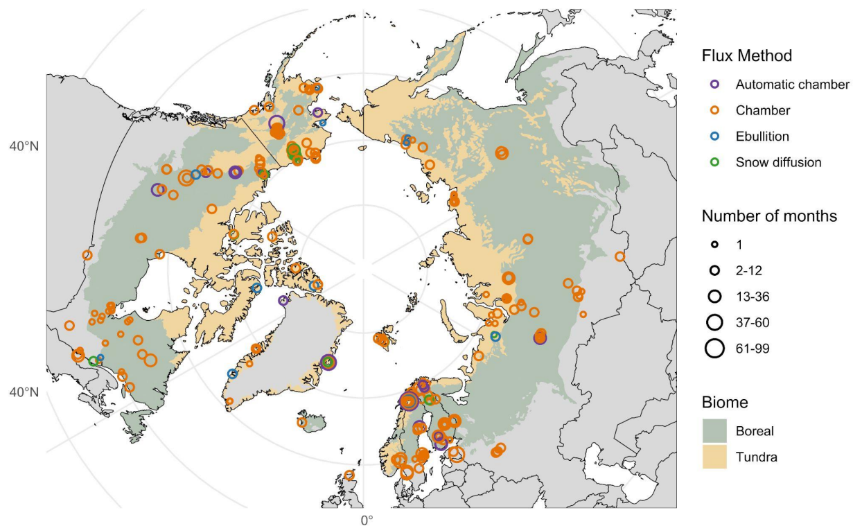
Figure S10. Site-months of non-eddy covariance based measurement sites.
