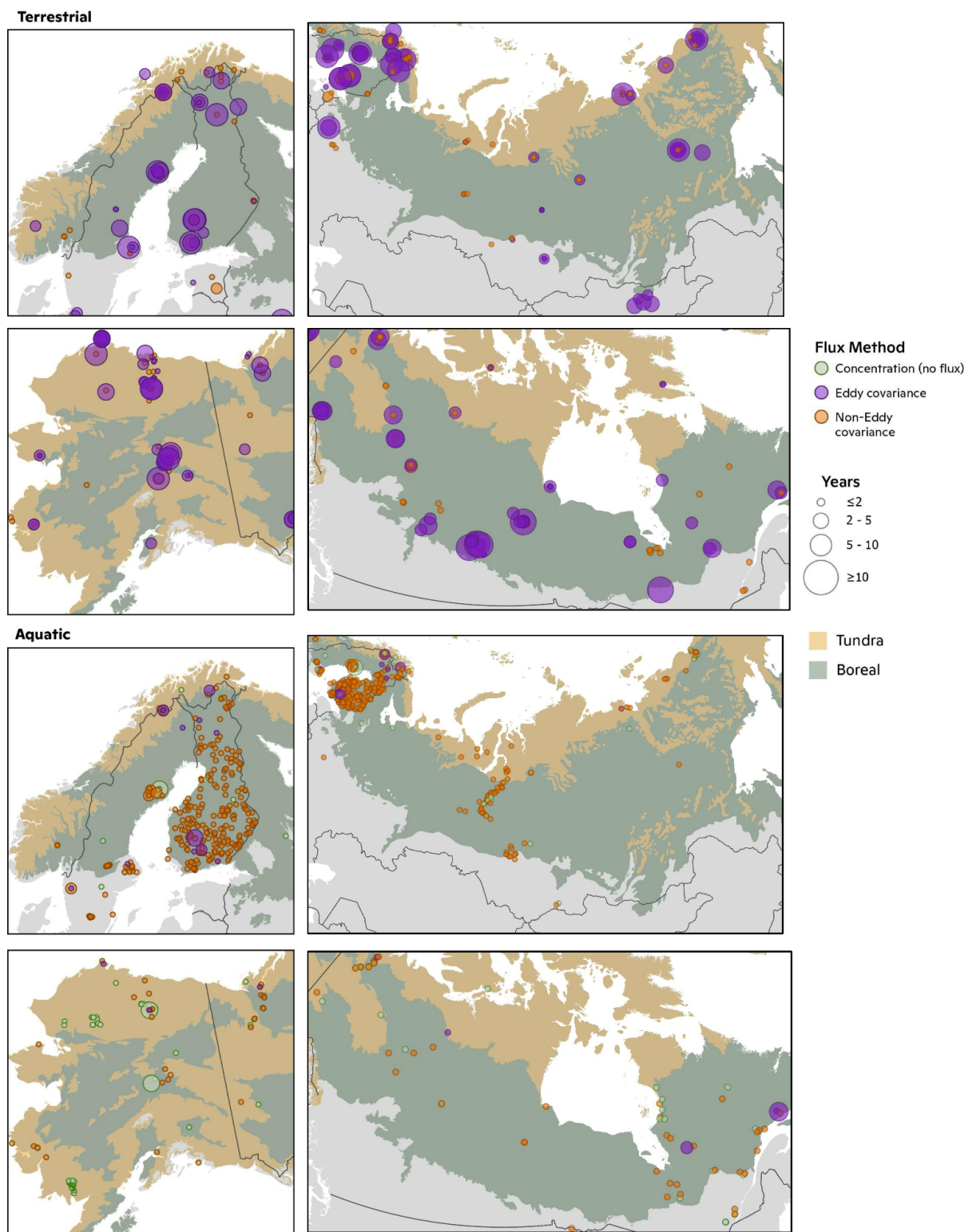
Figure S8. Zoomed-in maps of regional flux sites.
