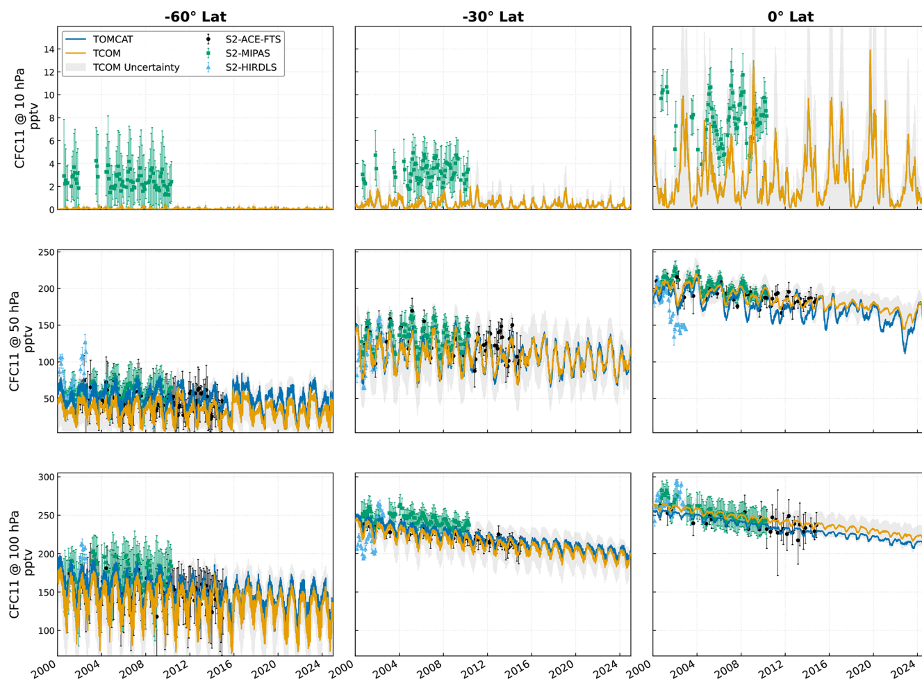
Figure 9. Temporal comparison of daily-mean CFC-11 VMRs (in pptv) from 2000 to 2024 across three distinct latitudes ( 60^{\circ} S, 30^{\circ} S and 0^{\circ} ) at three stratospheric pressure levels: 10 hPa ( \approx 30 km), 50 hPa ( \approx 20 km), and 100 hPa ( \approx 16 km). Data sources shown include: the TOMCAT CTM output (solid blue lines), the XGBoost-predicted TCOM dataset (solid orange lines), and TCOM uncertainty ( \pm 1\sigma derived from quantile regression, light orange shading). Monthly mean data points from observation-based data from the SPARC v2 (Hegglin et al., 2021) are also shown. Data points and related standard deviations from ACE-FTS, MIPAS and HIRDLS are shown with black, green and aqua coloured dots, respectively.
