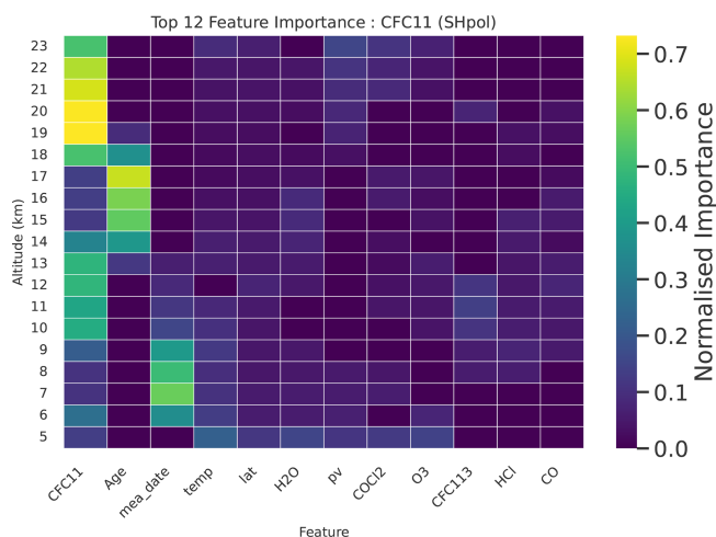
Figure 3. Normalised feature importance heatmap for CFC-11 in the Southern Hemisphere polar (SHpol) latitude bin, derived from the XGBoost regression model. The y-axis represents altitude (in km), and the x-axis lists the 12 most important input features. The colour intensity indicates the normalised relative importance of each feature at a specific altitude level for predicting the ACE-FTS CFC-11 VMR.
