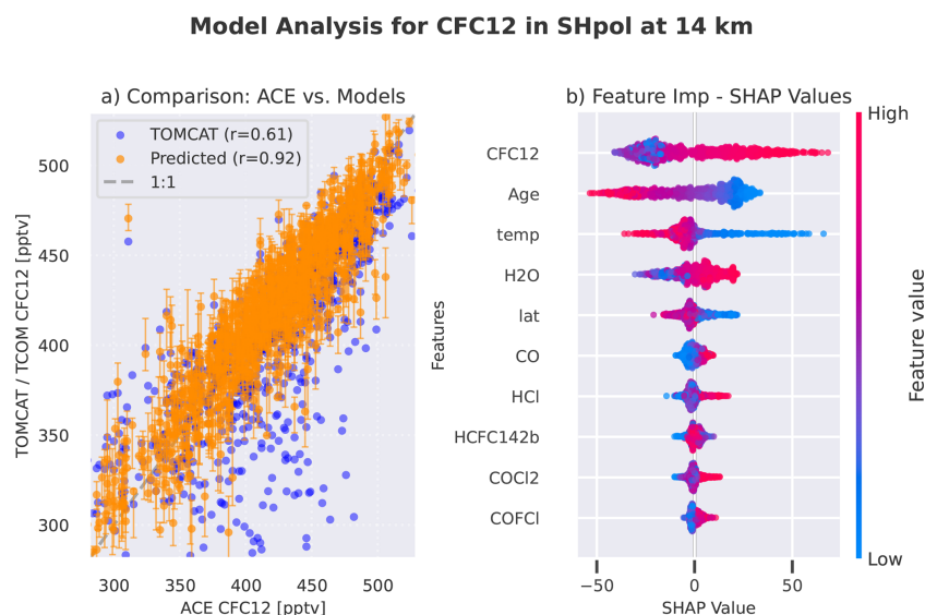
Figure 6. Same as Fig. 5, but for CFC-12.
