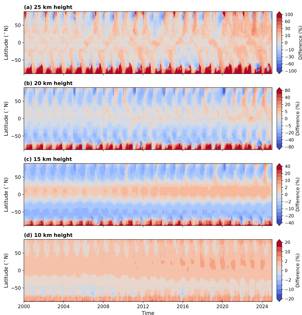
Figure 8. Same as Fig. 7, but for CFC-12, comparing TOMCAT and TCOM data.
