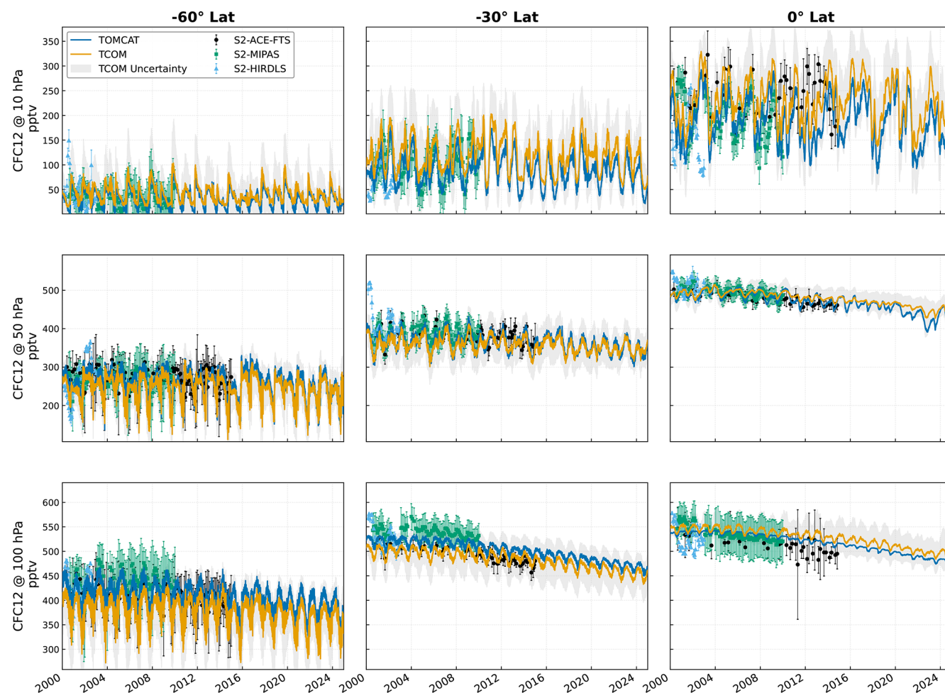
Figure 10. Same as Fig. 9, but for CFC-12.
