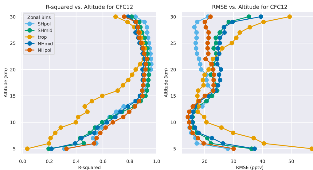
Figure 2. Same as Fig. 1, but for CFC-12.
