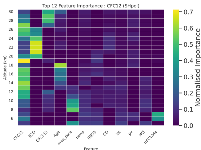
Figure 4. Same as Fig. 3 but for CFC-12 and different y-axis range, showing the altitude-dependent normalised relative importance of 12 most important features for the CFC-12 prediction.
