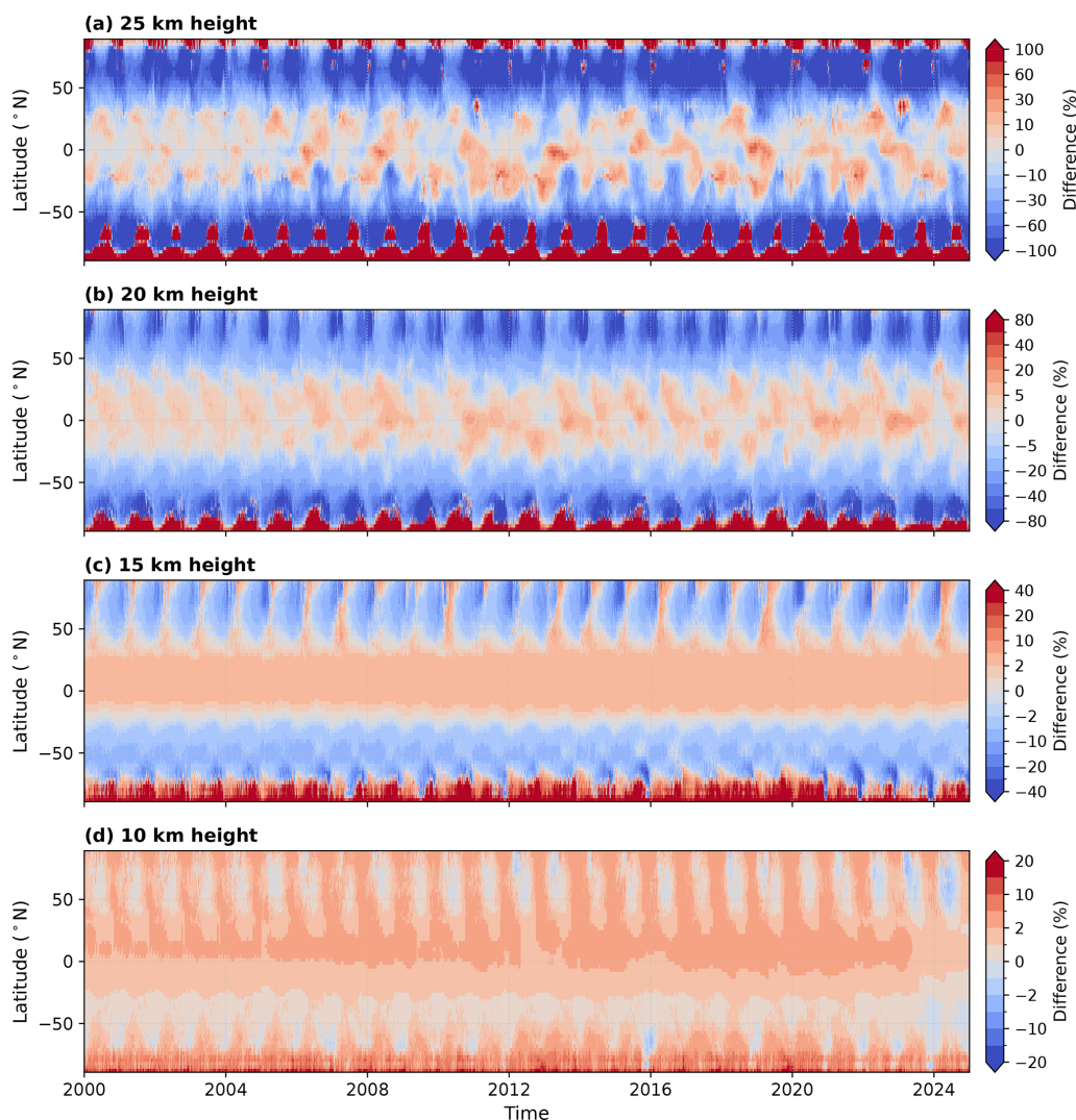
Figure 7. Percentage differences between the TCOM and TOMCAT VMRs of CFC-11 as a function of time (2000–2024) and latitude (85°S to 85°N). Differences are presented for four altitude levels: 25 km (top panel), 20, 15, and 10 km (bottom panel). The differences are calculated as 100 \times (\text{TCOM} - \text{TOMCAT}) / \text{TOMCAT} . The colour-bar scales for the percentage difference are irregular and optimised for each individual altitude panel.
