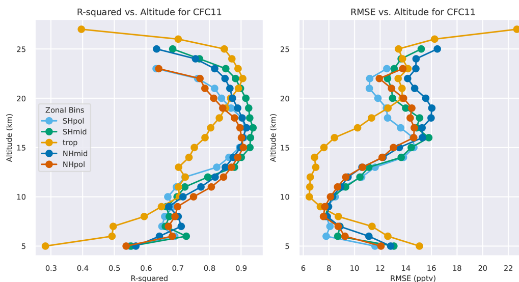
Figure 1. Coefficient of determination ( R^2 , left panel) and root mean squared error values (RMSE, right panel, in parts per trillion by volume (pptv)) for all 5-latitude bands from the XGBoost regression model.
