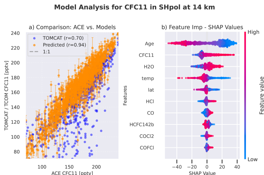
Figure 5. (a) Comparison of CFC-11 VMRs (in parts per trillion by volume or pptv) at 14 km altitude in the Southern Hemisphere polar (SHpol) latitude band. The scatter plot compares ACE-FTS observations (horizontal axis) against the model output: TOMCAT CTM (blue circles) and XGBoost regression model estimated VMRs (TCOM, orange circles). The vertical lines on the TCOM data represent the estimated uncertainties derived using quantile regression (25th and 75th percentiles). The dashed grey line indicates the 1:1 line to illustrate deviations with respect to ACE-FTS data. The legend also includes the Pearson correlation between ACE-FTS and the TOMCAT or TCOM data. (b) SHAP (SHapley Additive exPlanations) values for the XGBoost model at the same level (14 km). The SHAP values indicate the relative importance of each input feature and the direction (positive or negative) of their influence on the XGBoost model's prediction (corrected as TCOM).
