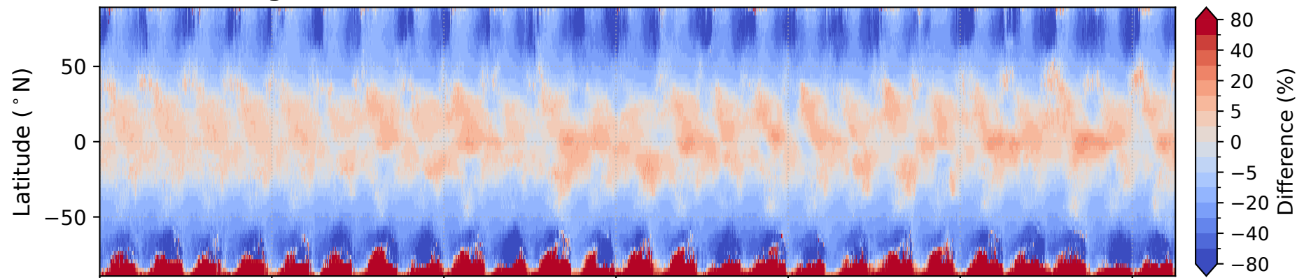
(b) 20 km height
