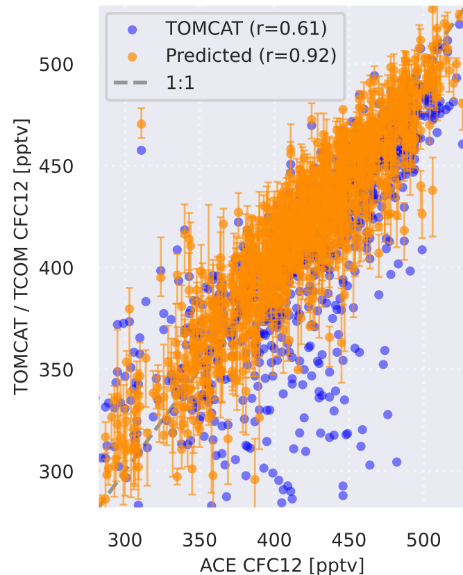
a) Comparison: ACE vs. Models
