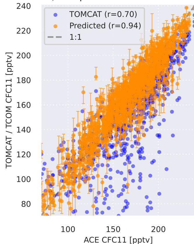
a) Comparison: ACE vs. Models
