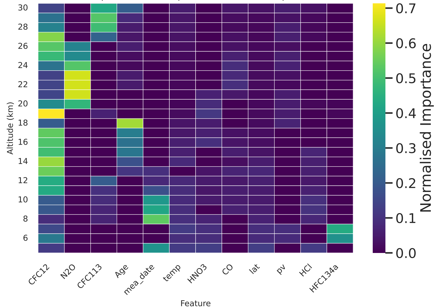
Top 12 Feature Importance : CFC12 (SHpol)
