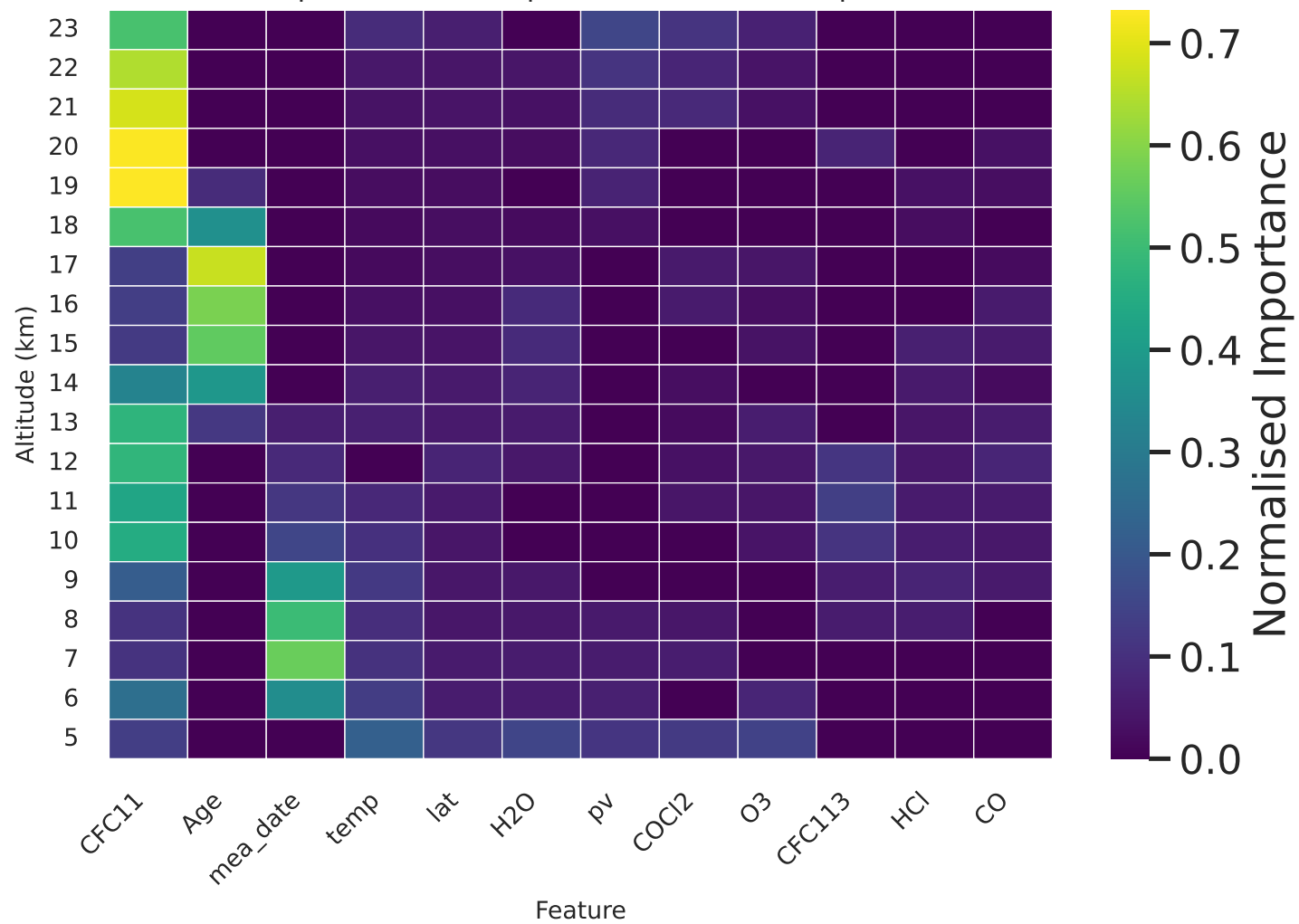
Top 12 Feature Importance : CFC11 (SHpol)
