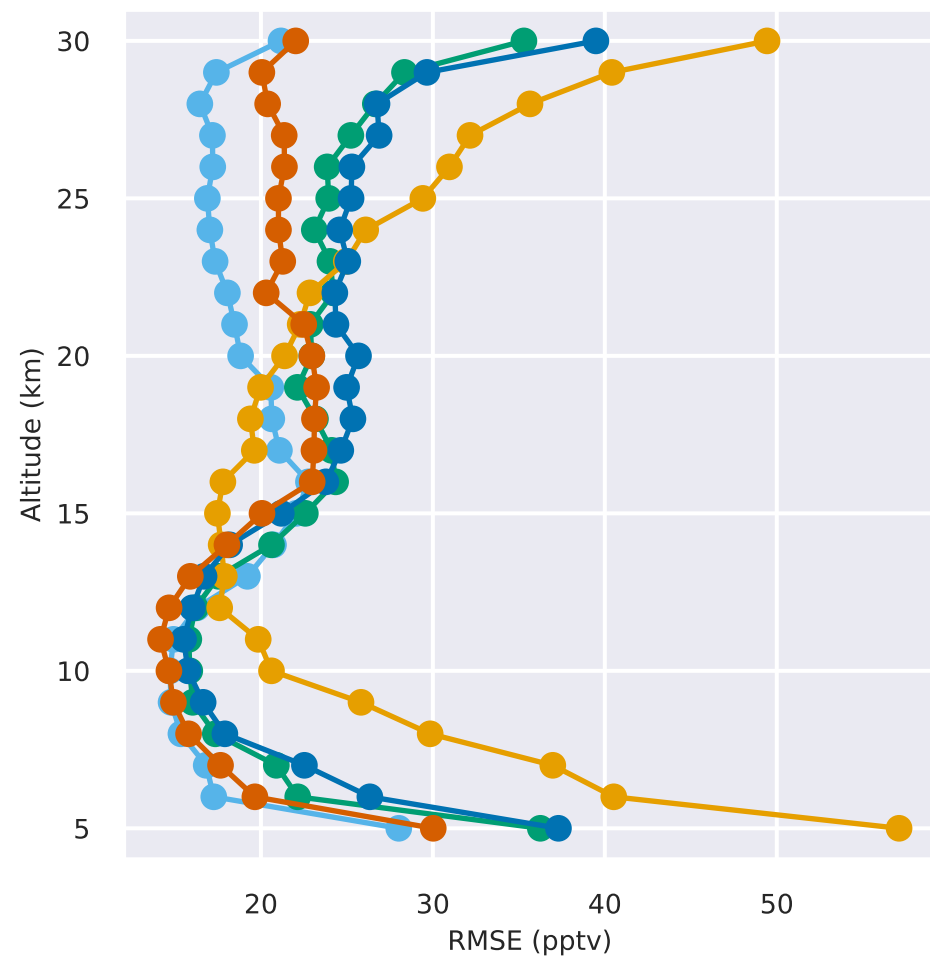
RMSE vs. Altitude for CFC12
