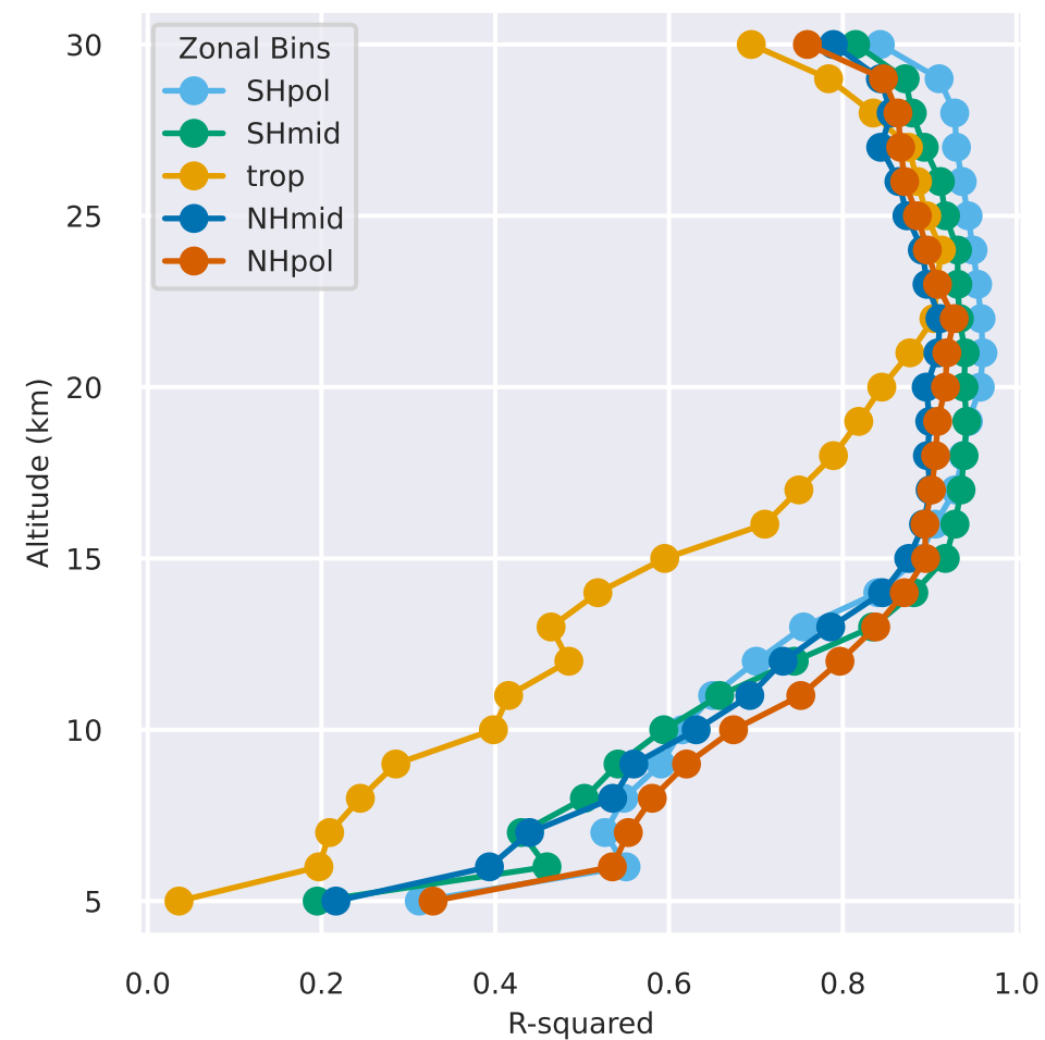
R-squared vs. Altitude for CFC12
