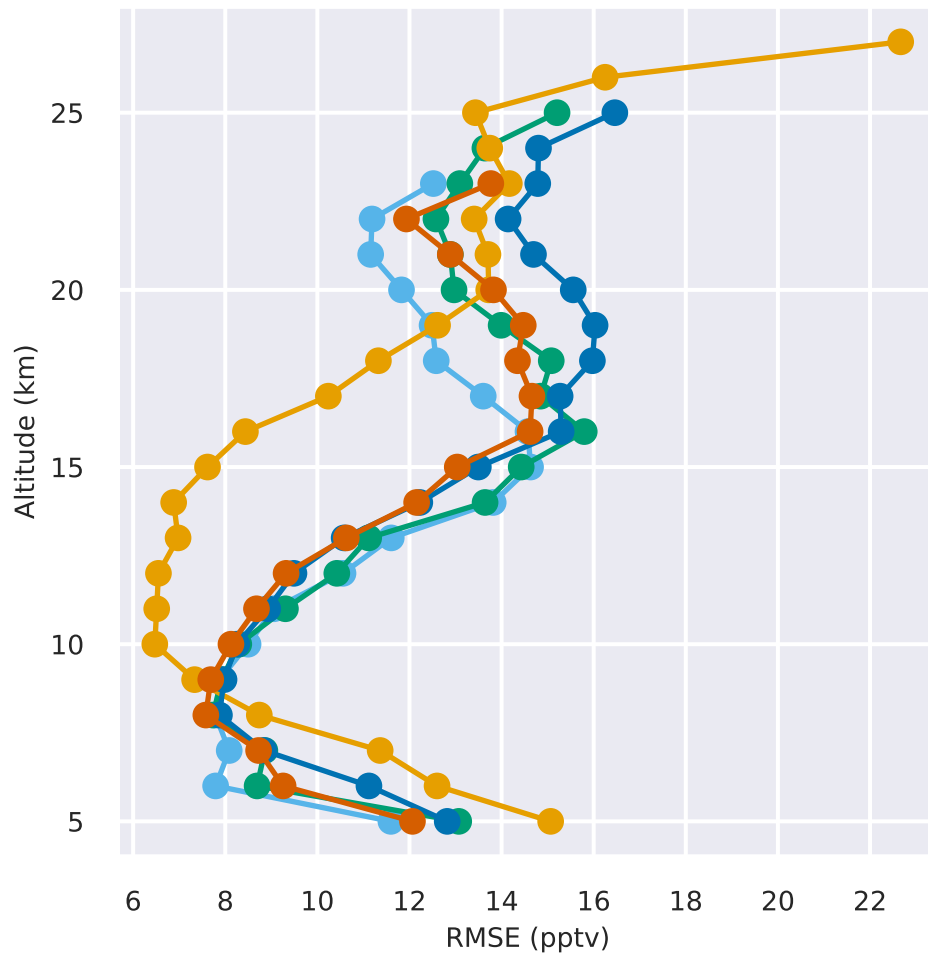
RMSE vs. Altitude for CFC11
