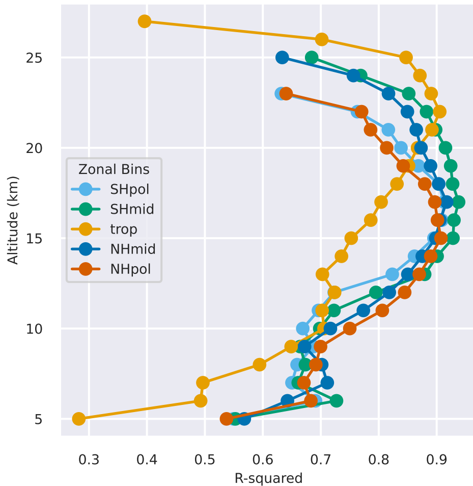
R-squared vs. Altitude for CFC11
