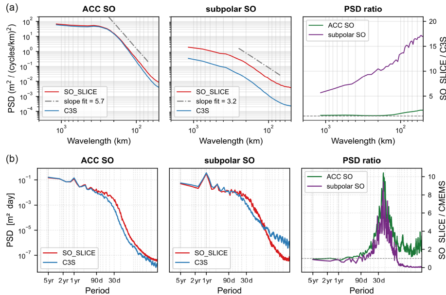
Figure 6. (a) Spatial PSD of SO_SLICE and C3S SLA fields in the ACC region and the subpolar Southern Ocean, as well as the ratio between SO_SLICE and C3S PSD. The linear fit between 250 and 70 km is plotted, and the associated slope is given in the legend. (b) Temporal PSD of SO_SLICE and C3S in the ACC and the subpolar Southern Ocean, with the PSD ratio for each region.
