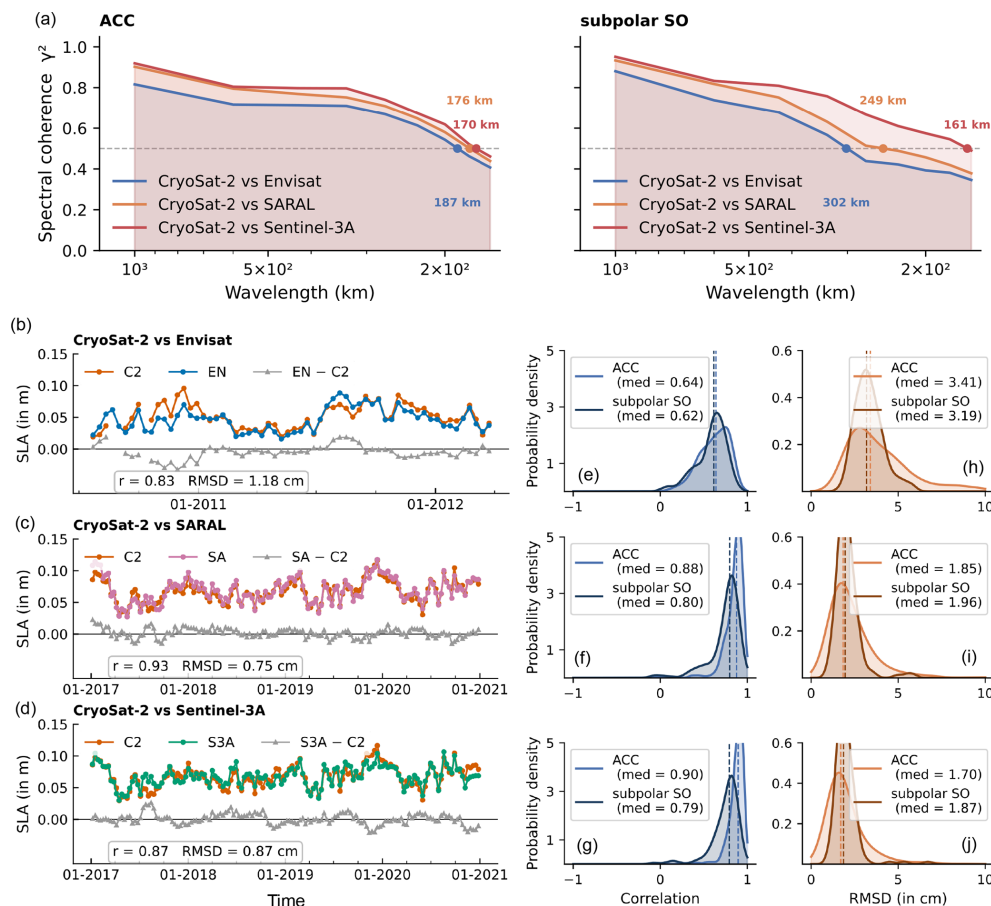
Figure 7. For each satellite mission, observations are binned onto the EASE2 75 km grid, with a 10 d time step. No optimal interpolation is used here. The resulting maps are compared between mission pairs. (a) Spatial spectral coherence for each pair of 75 km maps with a 10 d time step. (b, c, d) SLA spatially averaged over the subpolar Southern Ocean, compared between overlapping mission pairs (b): CryoSat-2 vs. Envisat, c: CryoSat-2 vs. SARAL, d: CryoSat-2 vs. Sentinel-3A). (e, f, g) Probability density of grid-point temporal correlations for each mission pair, on maps coarsened to 300 km per 300 km. The distribution is split between the ACC region and the subpolar Southern Ocean, as in Fig. 6. Median values are indicated by dashed lines. (h, i, j) Same as (e, f, g) but for the RMSD, in centimeters.
