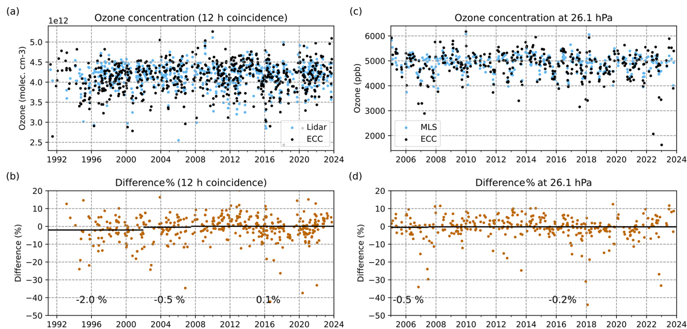
Figure 12. Time series of ozone concentration of the stratospheric lidar and the ECC ozonesonde at 25 km, and MLS and the ECC ozonesonde at 26.1 hPa (a, c). Ozone concentration and (b, d) relative ECC minus lidar ozone concentration differences for the coincident (< 12 h) profiles. Ozone concentrations for (a)–(b) are calculated at altitude 25 km by averaging ozone over a range of \pm 1 km. Ozone concentrations for (c)–(d) are calculated at pressure level 26.1 hPa by averaging ozone over a range of \pm 1 layer (31.6–21.5 hPa). Black lines with values in (b) and (d) indicate average relative differences for the periods same as Figs. 1–2.
