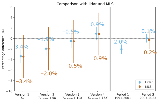
Figure 9. Evaluation of ECC ozone concentration compared with lidar and MLS ozone concentrations. Results are presented as medians and 2 \times standard errors of percentage difference for a corrected and two uncorrected periods. An uncorrected and three corrected ECC ozone concentrations are tested for the period January 2002–June 2007.
