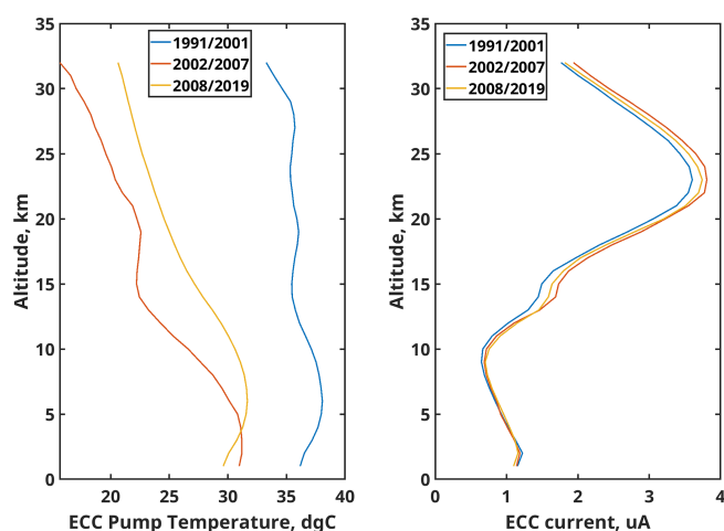
Figure 5. Mean vertical profile of homogenized ECC pump temperature in °C (left panel) and ECC current in μA (right panel) for period 1991/2001, 2002/2007 and 2008/2019.
