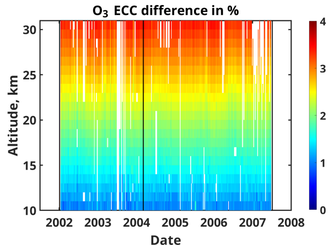
Figure 10. Differences between the ozone concentration calculated without any correction of the homogenized ECC temperature (Version 1 of T_{Pcor} ) and with Version 3 of T_{Pcor} as a function of altitude for the time period 2002–2007.
