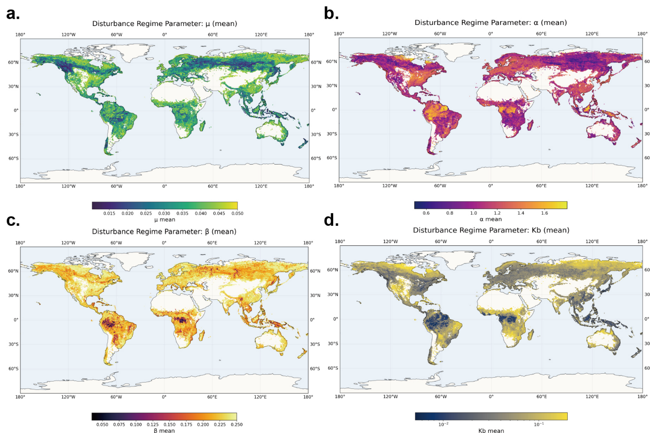
Figure 4. Global patterns of predicted disturbance regime parameters. The four panels show the grided global maps of ensemble means for (a) \mu , (b) \alpha , (c) \beta , and (d) K_b . Each parameter is displayed with a distinct color scale to highlight its unique spatial patterns.
