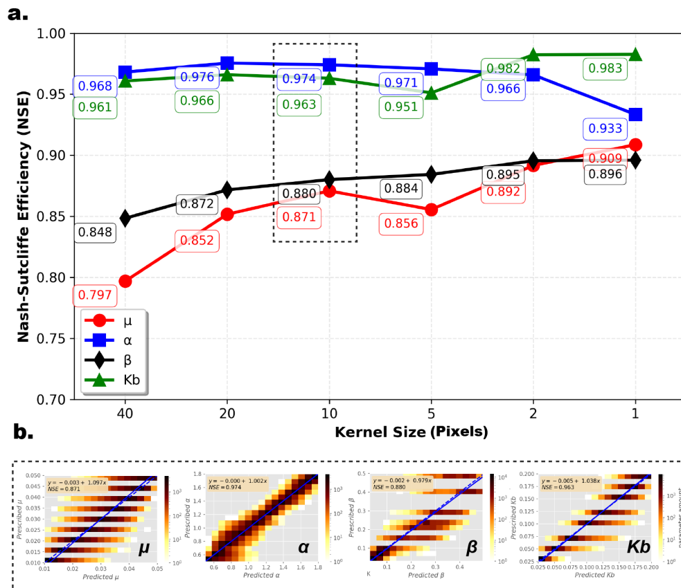
Figure 2. Model predictive performance across spatial aggregation scales. The main panel (a) displays the Nash-Sutcliffe Efficiency (NSE) for predicting disturbance parameters using a 10-fold random cross-validation Random Forest model. The x-axis represents the aggregation of kernel size, where a value of 1 corresponds to the original resolution, and coarser scales are to the left. Panel (b) shows density scatter plots for the optimal aggregation scale (kernel size = 10) at the global level, comparing model predictions (x-axis) to the prescribed parameters (y-axis). The color scale indicates the density of samples, with darker colors representing a higher concentration of points. The consistently high NSE values across scales demonstrate that predictive power is maintained even at coarser resolutions.
