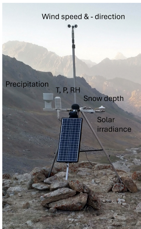
Figure 3. Photograph of AWS with the different sensors indicated ( T = temperature, P = pressure, RH = relative humidity). Photography by Antti Hyvärinen (18 September 2021).
