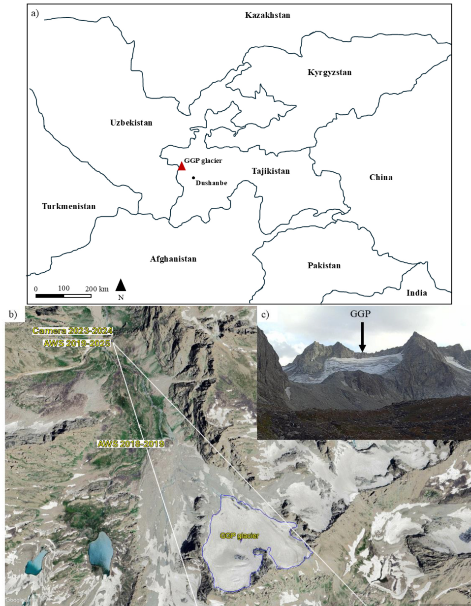
Figure 1. (a) Map of Central Asia and Tajikistan with the location of GGP indicated by red triangle. (b) Satellite imagery of the study area. The outline of GGP is from 2024. AWS stands for automatic weather station. Field of view of the camera installed in 2023 is indicated with white lines. (c) Inserted image of GGP (top right) as seen from the weather station camera on 4 September 2023. Maps data: © Google Earth 2026; images © Airbus 2026.
