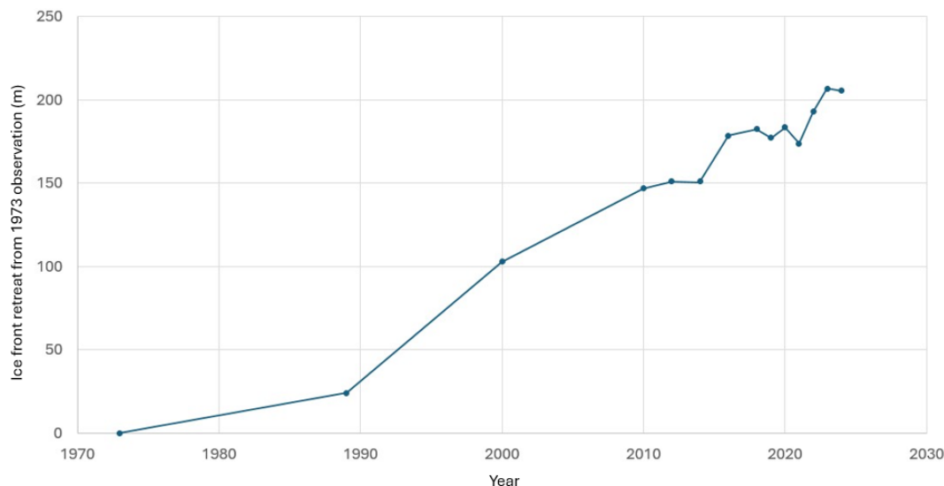
Figure 5. Retreat of GGP terminus from 1973 outline (Vladimirova et al., 1976) to variations determined 1989–2024.
