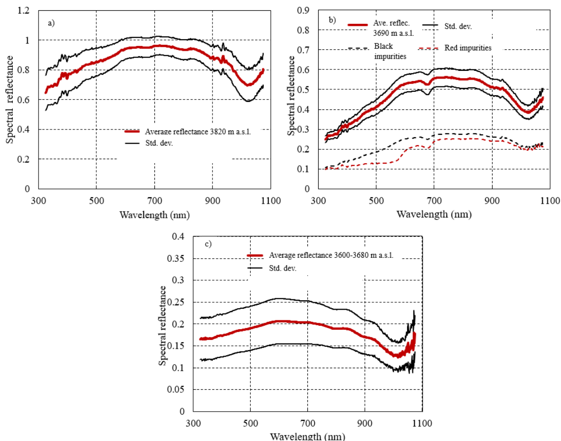
Figure 9. Average reflectance and standard deviation of reflectance measurements of the glacier surface with black, brownish and red impurities. (a) Higher section of GGP 2019. (b) Mid-section of GGP in 2019. (c) Ablation zone in 2023.
