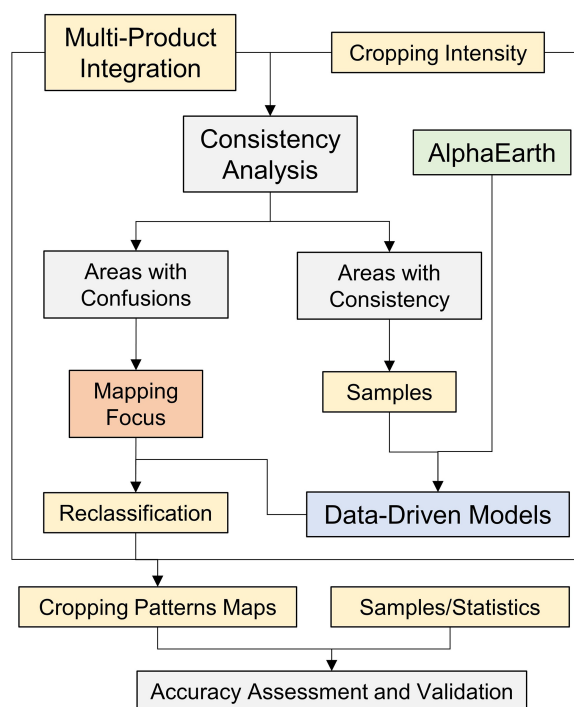
Figure 1. Workflow of this study.
