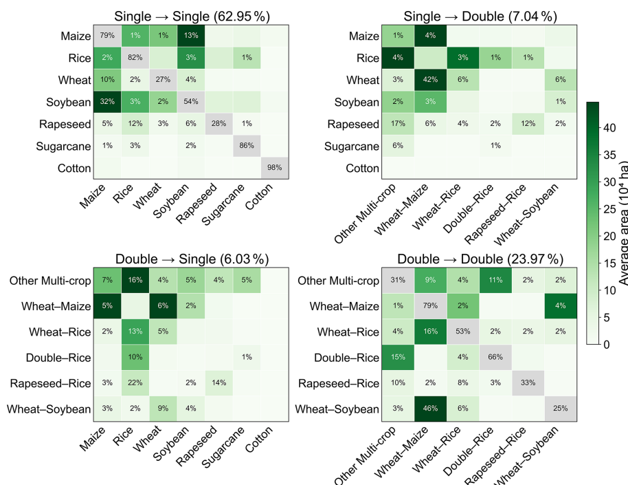
Figure 7. Heatmaps showing the average area of transitions among cropping patterns in China from 2018 to 2021.
