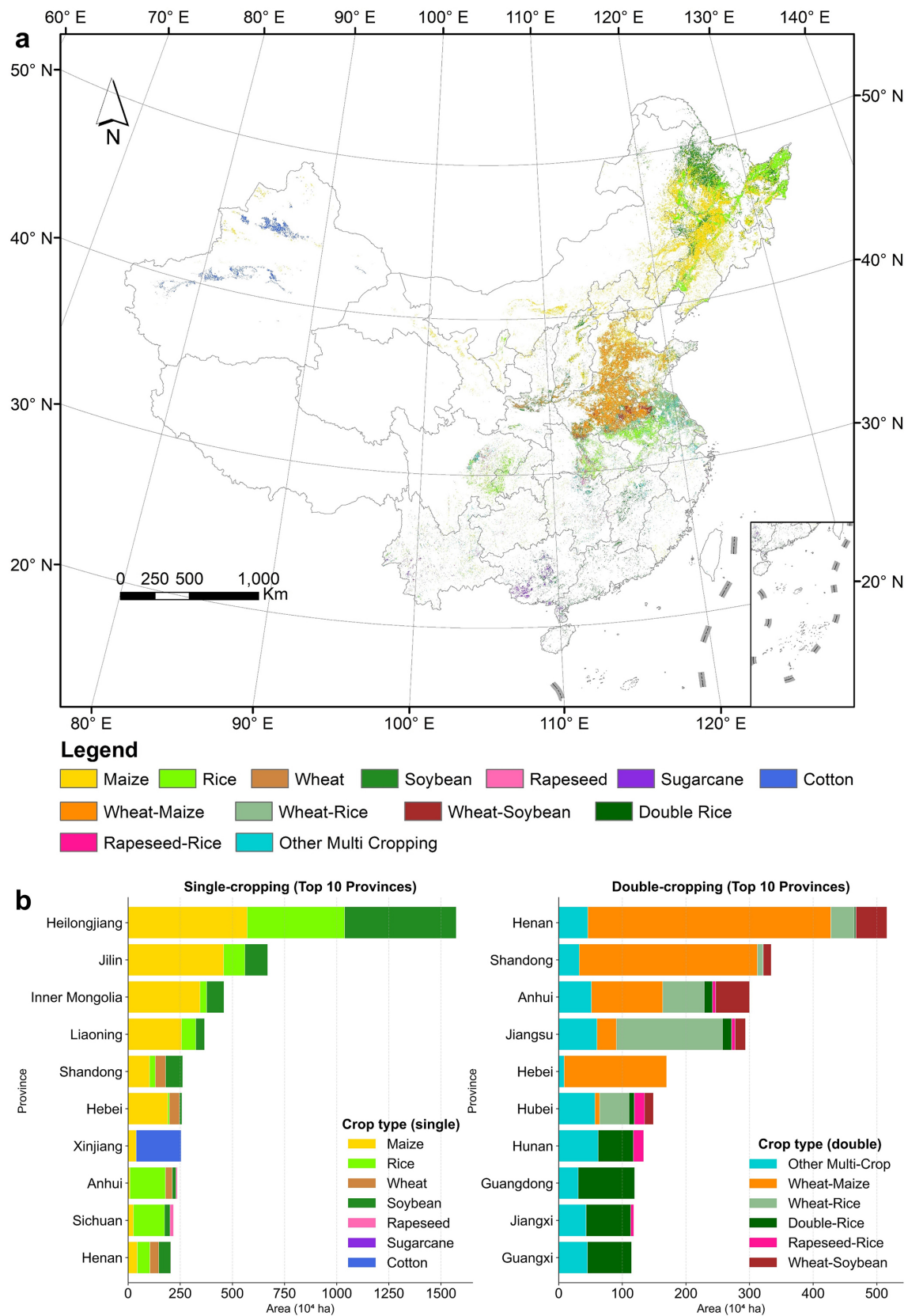
Figure 5. Our maps of Cropping Pattern in China (year 2020 as an example). (a) spatial distribution of cropping patterns; (b) crop area aggregated at the province level.
