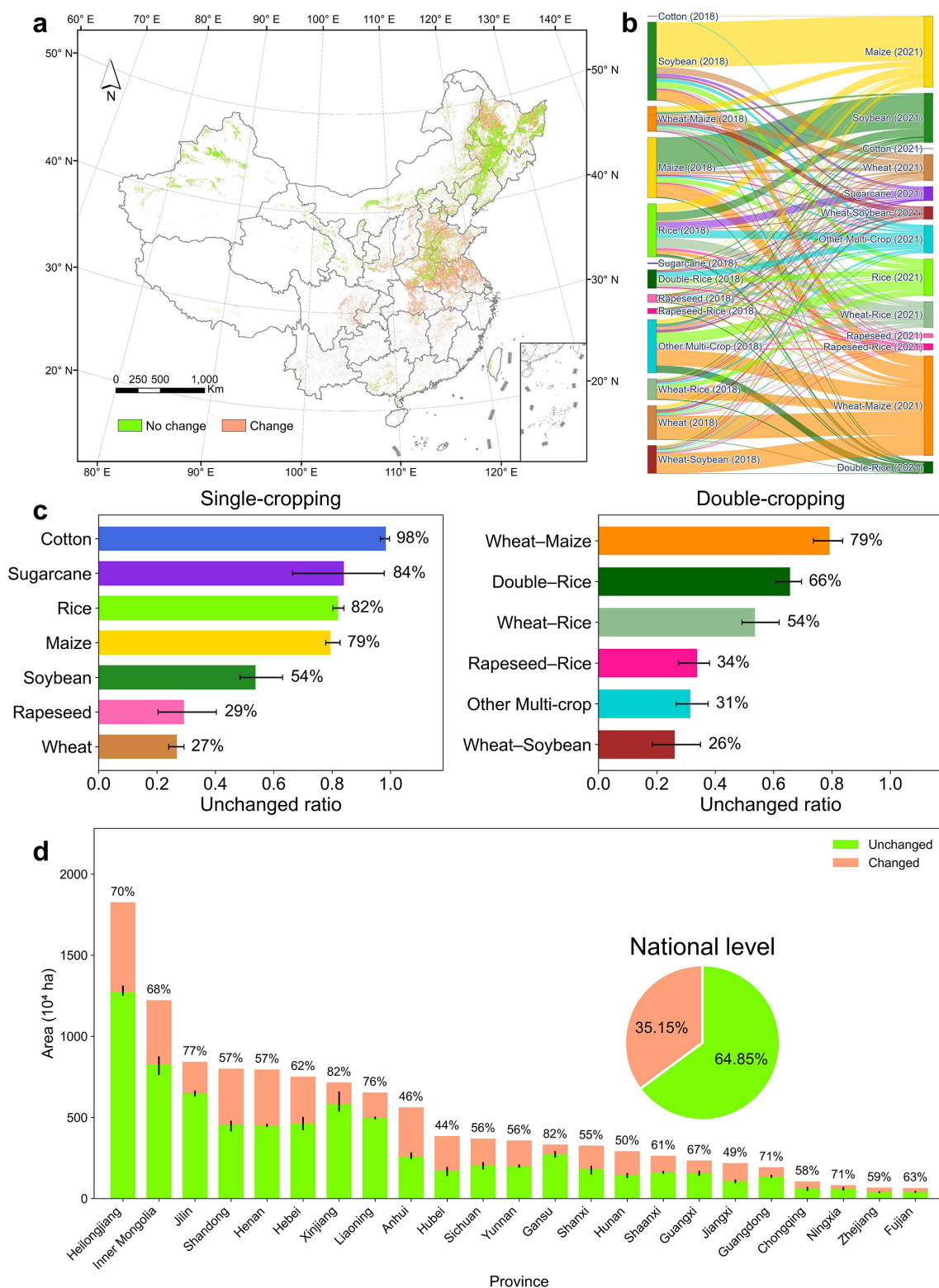
Figure 6. Cropping pattern changes between 2018 and 2021 in China. (a) spatial distribution of changed cropping patterns; (b) Flows of cropland transitions among cropping patterns; (c) unchanged ratio of single- and double-cropping systems; (d) Provincial average unchanged and changed cropland areas.
