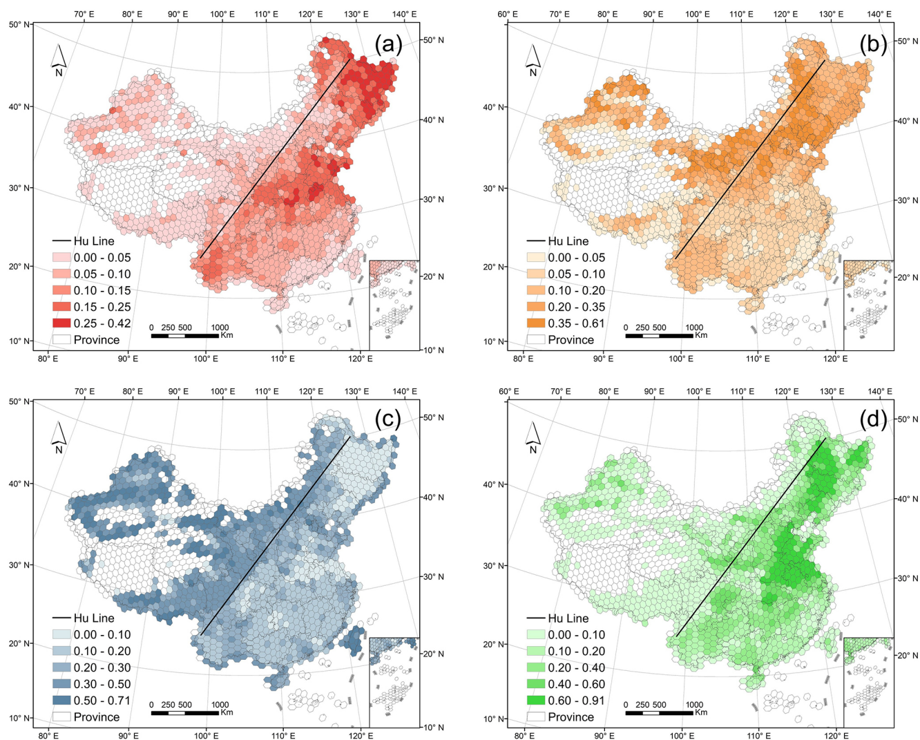
Figure 3. Proportional distribution of cropland and uncertain classes (Confused, Low-consistency, Unlabelled). (a) Proportional distribution of Confused areas. (b) Proportional distribution of Low-consistency areas. (c) Proportional distribution of Unlabelled areas. (d) Proportional distribution of Cropland.
