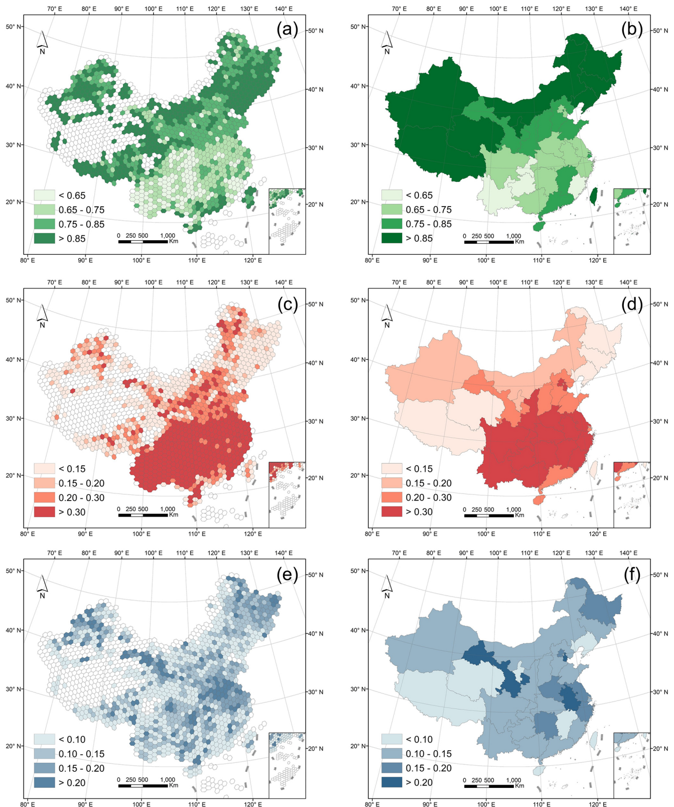
Figure 4. Spatial variation of mean accuracy of classifiers for year periods from 2018 to 2021. (a) F_1 score at hex grid level. (b) F_1 score at ADM-1 level. (c) Omission error at hex grid level. (d) Omission error at ADM-1 level. (e) Commission error at hex grid level. (f) Commission error at ADM-1 level.
