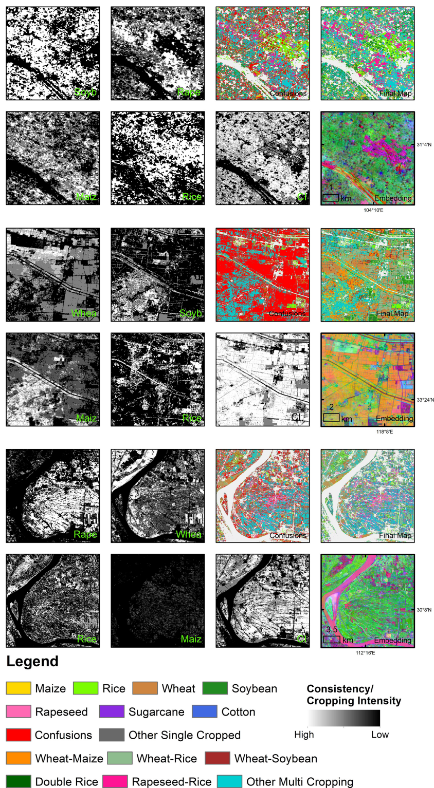
Figure 11. Comparisons of our results and other crop maps (more complex cropping systems) in the year 2020.
