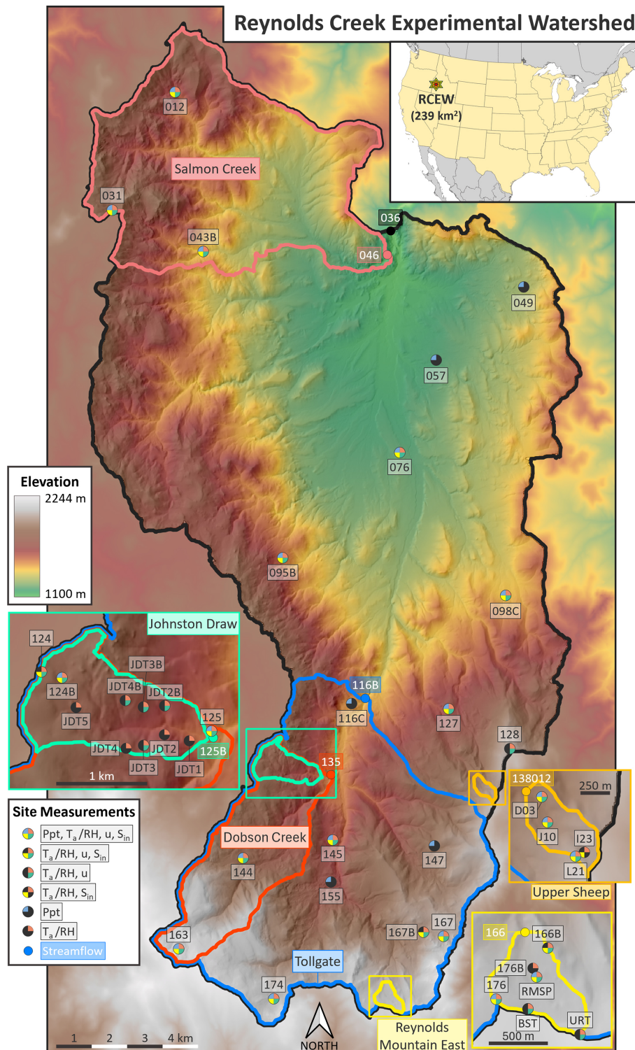
Figure 1. Map of Reynolds Creek Experimental Watershed overlaid on a 10 m digital elevation model with site locations of the meteorological measurements used to produce this dataset. Hourly site measurements include precipitation mass (Ppt), air temperature ( T_a ), relative humidity (RH), wind speed and direction ( u ), and incoming shortwave radiation ( S_{in} ). Also, the six primary sub-watersheds are delineated by their outlet weir locations where streamflow ( Q ) is measured. Weir sites are denoted by the solid single-color circles corresponding to the basin boundary colors.
