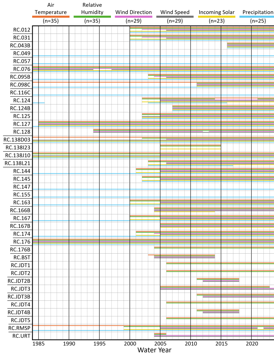
Figure 3. Annual water year measurement record used in SMRF gridded interpolation from the 40 individual sites within RCEW from 1 October 1983 to 30 September 2023. The horizontal bars for each variable indicate station observation data present for over half of a water year, however smaller data gaps are not shown. Some sites measure all six variables required by SMRF to produce the 12 gridded hydrometeorological forcing variables, though many are instrumented to measure fewer variables. For example, five stations solely measure precipitation (RC.049, RC.057, RC.116C, RC.147, and RC.155).
