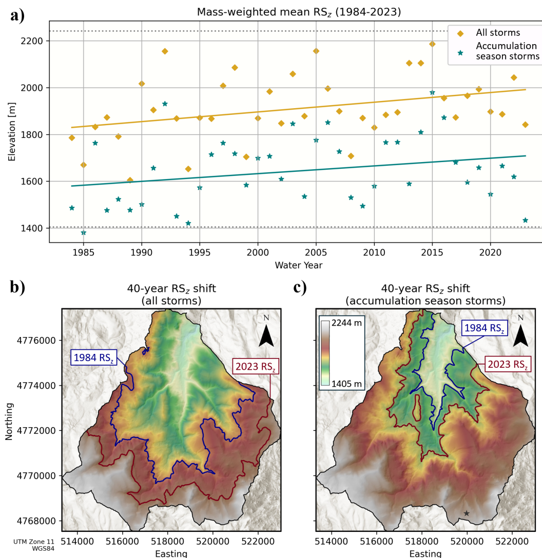
Figure 5. (a) The annual precipitation mass-weighted mean rain/snow transition elevation for water years 1984 to 2023 in the Tollgate sub-watershed for all storms over the course of a full year (orange diamonds and orange line of best fit) and the snow accumulation season from 1 October to peak SWE date (blue stars and blue line of best fit). Horizontal dotted lines represent the upper and lower elevations of the Tollgate sub-watershed. (b) The RS_z in 1984 (blue) and 2023 (red) when considering all storms in each year. (c) Same as (b) but only considering storms occurring from 1 October to the date of peak SWE at the Reynolds Mountain snow pillow (denoted by the black star).
