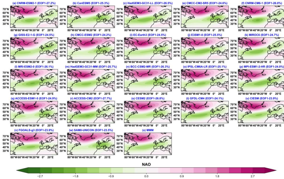
Fig. S1 Normalised spatial pattern of North Atlantic Oscillation (NAO; 1 st leading mode in 500hPa geopotential height over North Atlantic) from (a-w) 22 CMIP6 models (x) MMM. (d) EC-Earth3-CC has been excluded due to substantial gaps in the geopotential height dataset, with many intermediate years missing.
