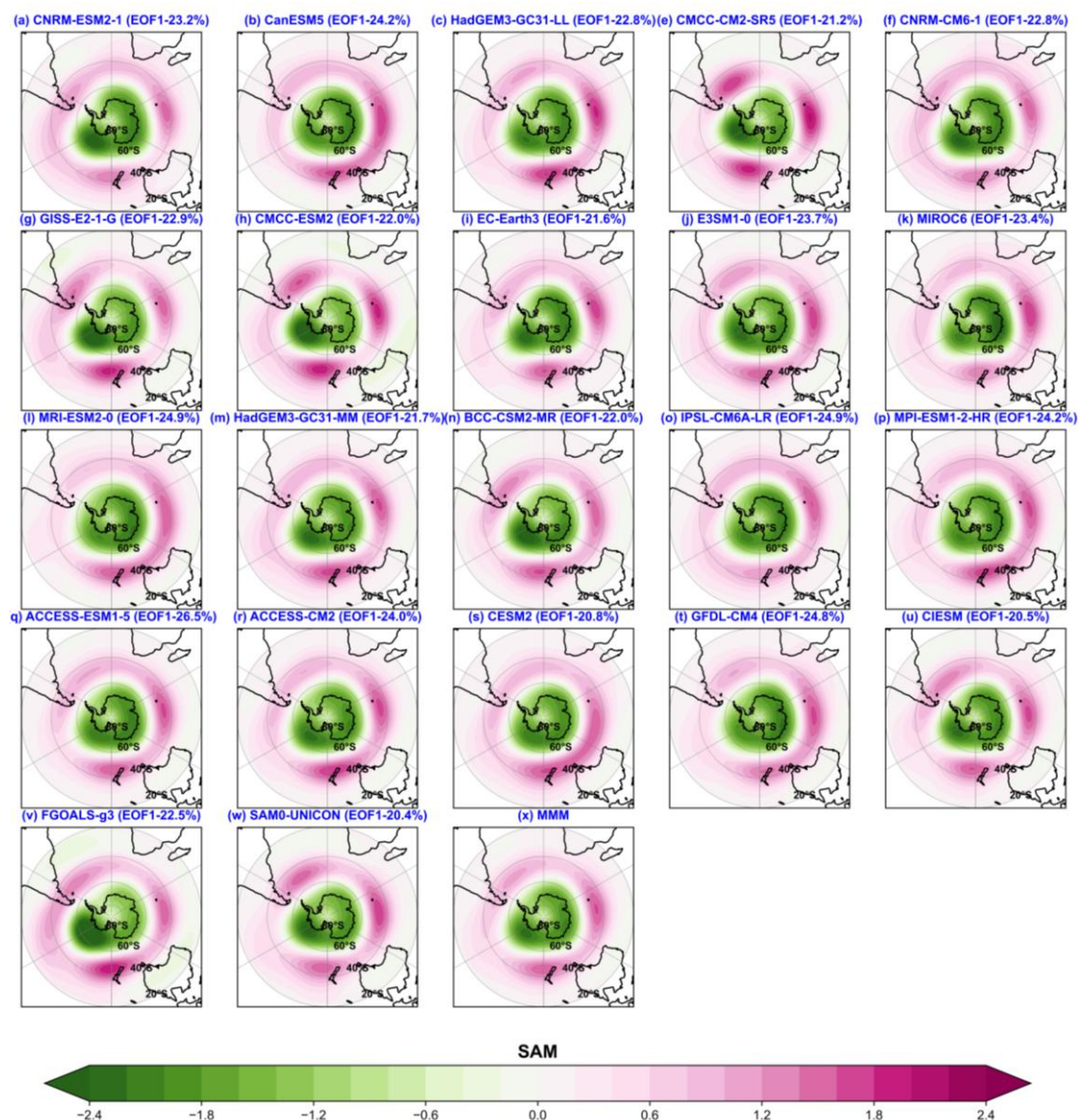
Fig. S2 Normalised spatial pattern of Southern Annular Mode (SAM; based on 1 st leading mode in 500hPa geopotential height over Southern Hemisphere extra tropics) from (a-w) 22 CMIP6 models (x) MMM. (d) EC-Earth3-CC has been excluded due to substantial gaps in the geopotential height dataset, with many intermediate years missing.
