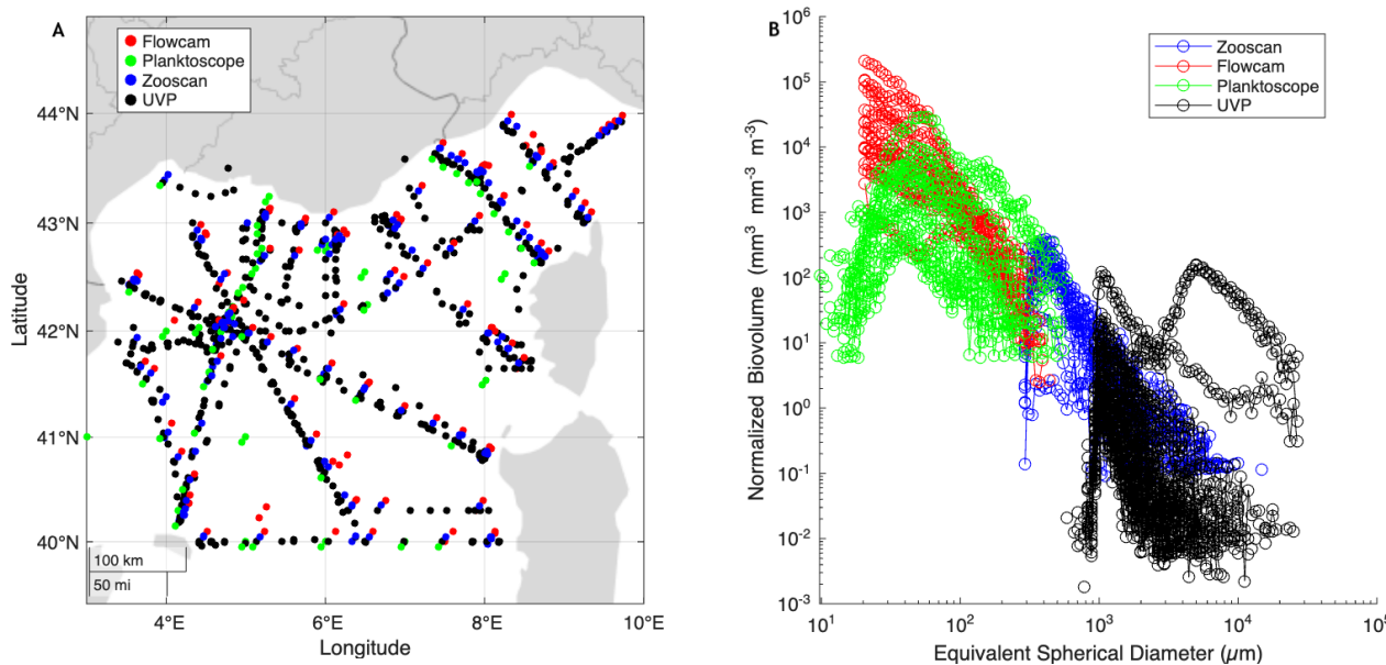
Figure 8. (A) Localisation of the different samples obtained and covering the size spectra of living organisms from microplankton (Flowcam, Planktoscope), mesozooplankton (WP2 nets analysed through Zooscan) and macrozooplankton and marine snow particles observed in-situ through profiling camera (UVP). (B) Comparison of the normalized size spectra of living organisms obtained with the different devices during the MOOSE-GE 2024 cruise, demonstrating the complementarity of instruments in capturing the continuum of life forms.
