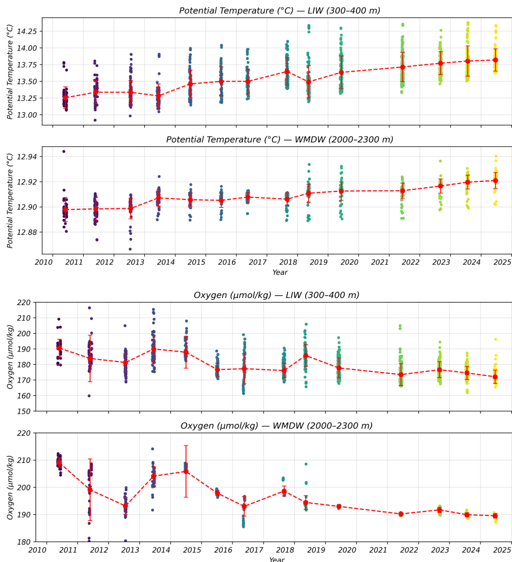
Figure 5. Time series of potential temperature (top panel) and dissolved oxygen (bottom panel) at LIW and WMDW core depth levels (300–400 m and >2000 m, respectively). The color represents the year and the red dots the average value for each year with the standard deviation.
