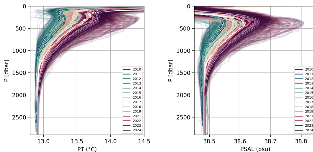
Figure 4. Potential temperature and practical salinity vertical profiles during the MOOSE-GE cruises from 2010 to 2024. The color represents the different years.
