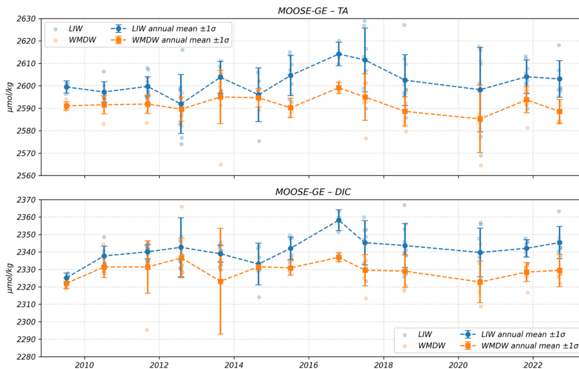
Figure 7. Evolution of TA and DIC concentrations (in \mu\text{mol kg}^{-1} ) in the intermediate waters (400–600 m) in blue and in the deep waters (>2000 m) in orange acquired during the MOOSE-GE cruises. The dots represent the annual mean with the standard deviation (from MOOSE-GE cruise series report, https://doi.org/10.18142/235 ).
