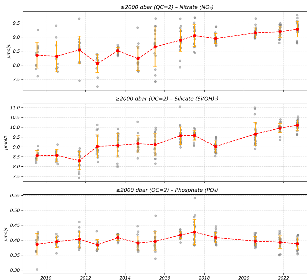
Figure 6. Evolution of nutrients concentrations (in \mu\text{mol L}^{-1} ) in the deep waters ( >2000 m) acquired during the MOOSE-GE cruises. The red dots represent the annual mean with the standard deviation.
