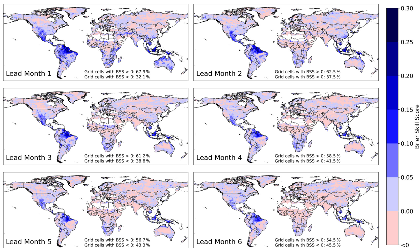
Figure 4. SEAS5-BCSD, Brier Skill Score (BSS) relative to climatology for precipitation, focusing on dry conditions below the 33rd percentile for Lead Months 1–6. Blue colors indicate higher skill than climatology, with darker shades representing better performance. Dry grid cells are excluded.
