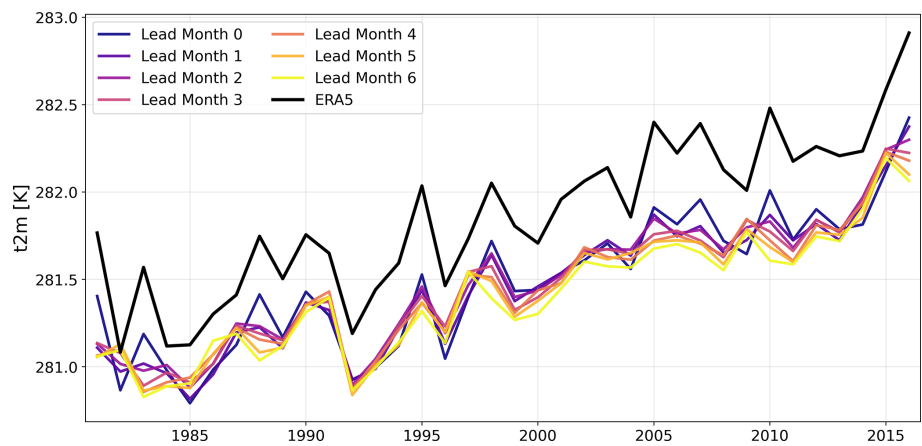
Figure A4. Bias between uncorrected SEAS5 and ERA5 for different lead times. Yearly means across all land masses are shown for the period 1981–2016.
