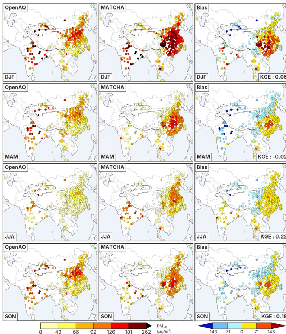
Figure 14. Seasonal averages of adjusted surface \text{PM}_{10} (after removing surface sea salt and dust) (in \mu\text{g m}^{-3} ) across the domain from OpenAQ (left column), MATCHA (middle), and the associated model bias (MATCHA-OpenAQ, right column).
