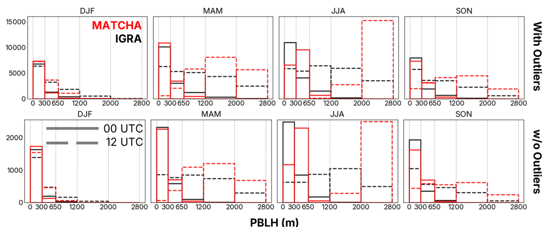
Figure A2. Histograms of both model (red) and observed (black) PBLH values compared across seasons and standard radiosonde launch times (solid for 00:00 UTC and dashed for 12:00 UTC) before and after applying the outlier-detection approach described in Sect. 2.2.4 of the main text.
