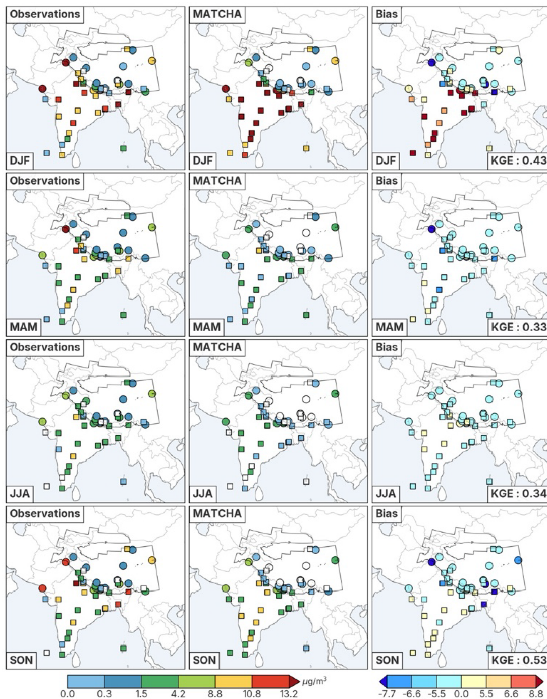
Figure 16. Seasonal mean of surface BC mass concentrations (in \mu\text{g m}^{-3} ) across observation sites in the domain from ground-based observation sites (left column), MATCHA (middle), and the median model bias (MATCHA-sites, right column). Circle markers denote sites from the APCC network with daily observations, and square markers denote sites with monthly or seasonal measurements (see main text for details).
