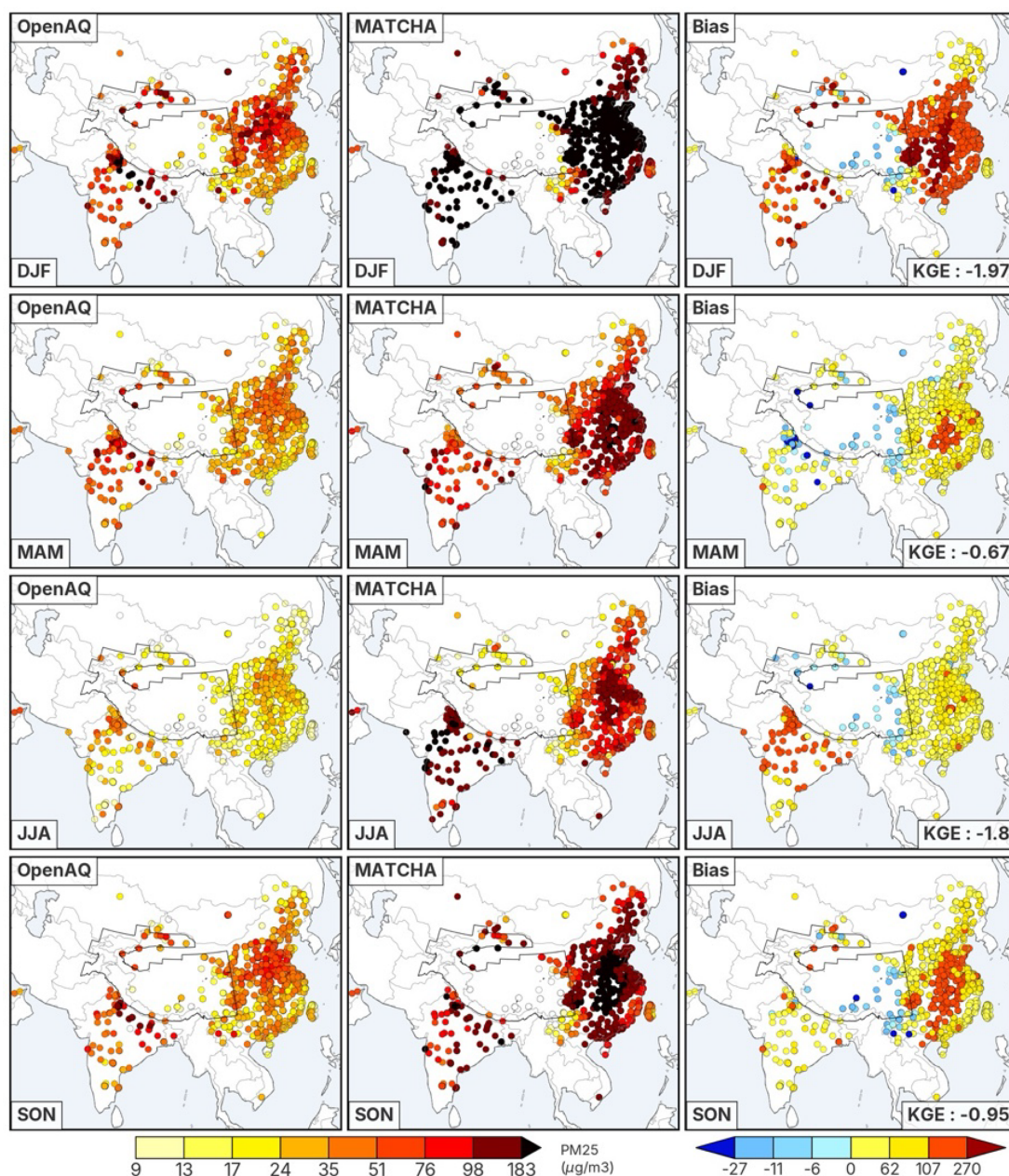
Figure 13. Seasonal averages of surface \text{PM}_{2.5} (in \mu\text{g m}^{-3} ) across the domain from OpenAQ (left column), MATCHA (middle), and the associated model bias (MATCHA-OpenAQ, right column).
