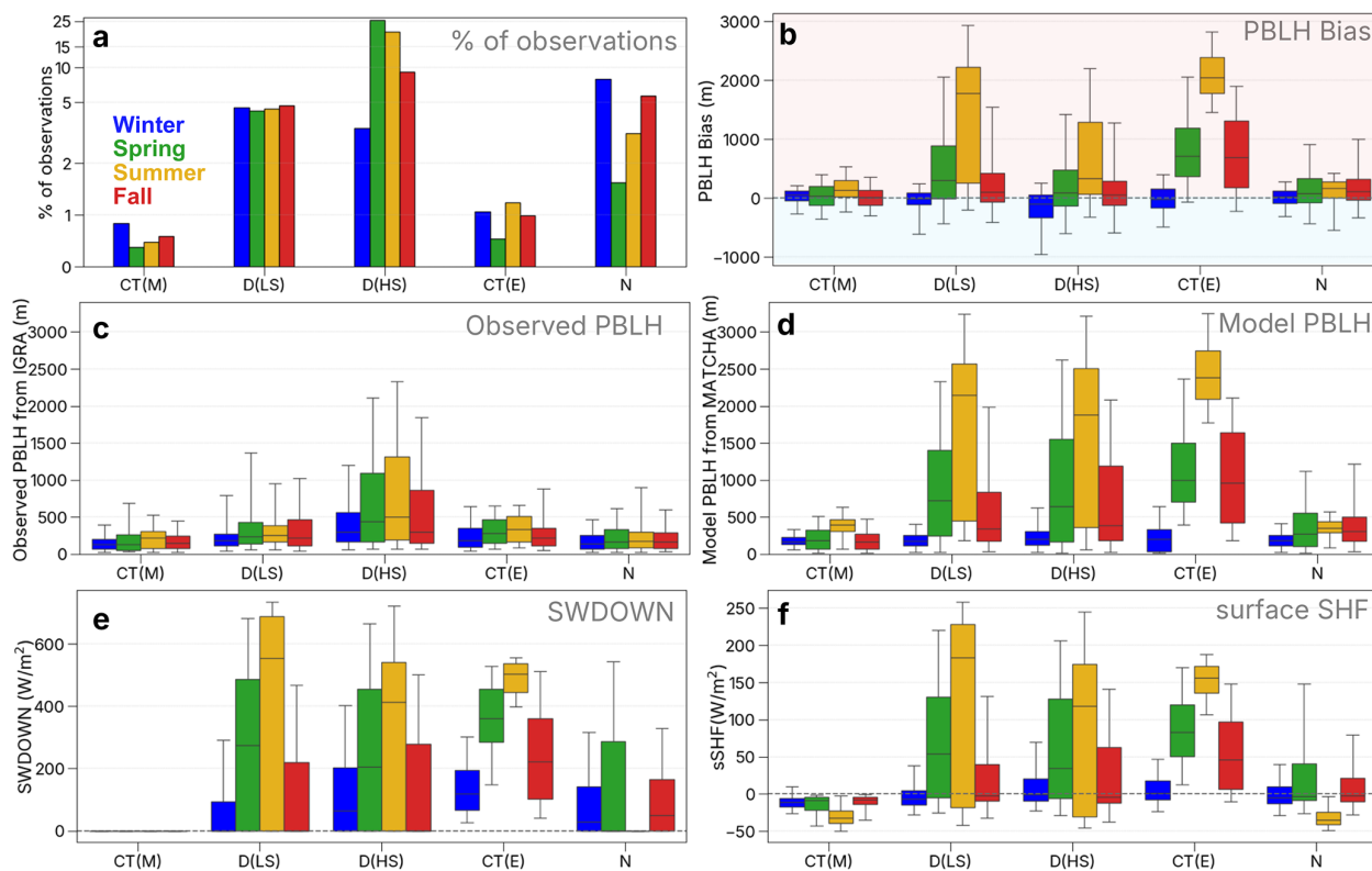
Figure A3. (a) Fraction (in %) of all 00:00 and 12:00 UTC radiosonde launches in the domain across different solar regimes (CT(M) = Morning Civil Twilight; D(LS) = Day – Low Sun; D(HS) = Day – High Sun; CT(E) = Evening Civil Twilight; N = Night) for each season. Solar regimes were defined by computing the solar elevation angle at the exact launch time of each radiosonde observations and classifying them into five exclusive categories: N ( \leq -6^\circ ), CT ( -6 to 0^\circ , split into morning or evening by solar azimuth), D (LS) ( 0 to 10^\circ ), and D(HS) ( > 10^\circ ). (b) PBLH bias (model-observed), (c) observed PBLH, and (d) modeled PBLH from IGRA and MATCHA across the solar regimes and seasons. (e) Downward shortwave radiation flux (SWDOWN) and (f) surface sensible heat flux (sSHF) collocated at IGRA sites from MATCHA across solar regimes and seasons.
