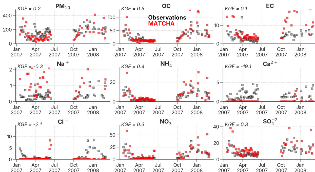
Figure 17. Observed (black) versus MATCHA-simulated (red) daily averaged (between 06:00–18:00 IST) concentrations (in \mu\text{g m}^{-3} ) of total \text{PM}_{10} and eight chemical species at Kanpur (26.5° N, 80.3° E) from January 2007 to March 2008.
