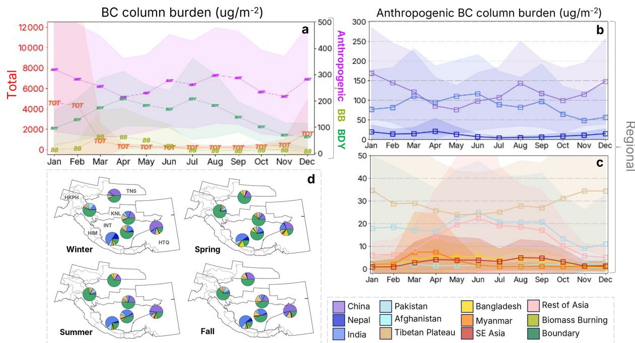
Figure 18. Average total column BC burden in \mu\text{g m}^{-2} across sectors (a), across ten tagged regions of anthropogenic total column BC (b–c), and the seasonal contribution (%) of the 12 tags (d) (ten tagged regions + biomass burning + trans-boundary inflow) at six HMA first-order glacier regions from RGI v6 (INT: Inner Tibet, S and E Tibet; HTQ: Hengduan Shan, Qilian Shan; TNS: W and E Tien Shan; KNL: W and E Kun Lun; HIM: W, C, and E Himalayas, HKPH: Hindu Kush, Karakoram, Pamir, and Hissar Alay). The shaded regions for (a)–(c) refer to the average standard deviation across all six regions. The legend refers to the colors of the regional and the sectoral tags applicable for (b)–(d).
