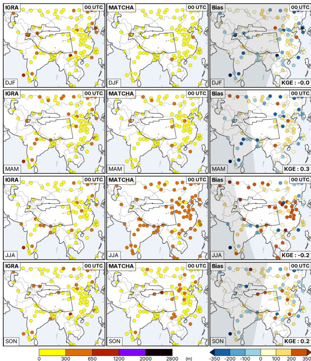
Figure 8. Seasonal averages of planetary boundary layer height at approximately 00:00 UTC from the IGRA archive (left column), MATCHA (middle column), and the associated model bias (MATCHA – IGRA, right column). The shadow zones show parts of the domain with nighttime conditions depending on the solar elevation angle on the 15th of the months; January (for DJF), April (for MAM), July (for JJA), and October (for SON), for the year 2003.
