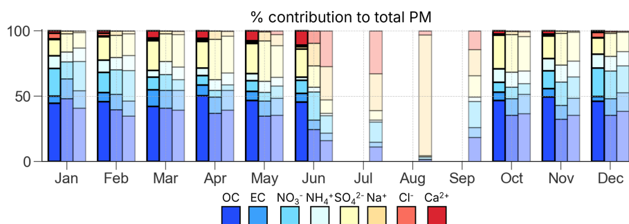
Figure A7. Monthly averaged percentage contribution of eight chemical species to total particulate matter over the Kanpur site based on \sim 1 year of observations from the site (first group of bars), \sim 1 year of model simulation over the site (second group) and 17-year contribution (third group) from the model simulation over the site.
