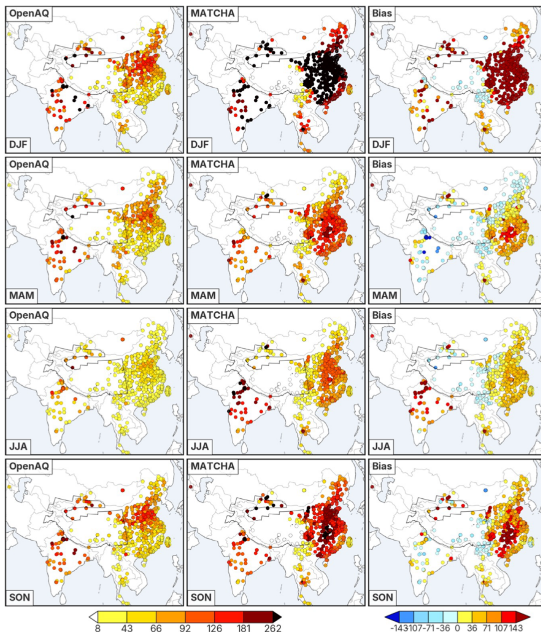
Figure A5. Seasonal averages of total surface \text{PM}_{10} (in \mu\text{g m}^{-3} ) across the domain from OpenAQ (left column), MATCHA (middle), and the associated model bias (MATCHA-OpenAQ, right column).
