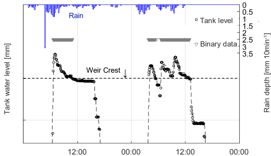
Figure S48. Continuous tank water level ( ^{\circ} ) and binary information (derived from the capacitive sensor signal) reflecting the overflow activity for a period of two days for which two independent overflow events were recorded. Monitoring frequency is 5 minutes, for rainfall it is 1 minute.
