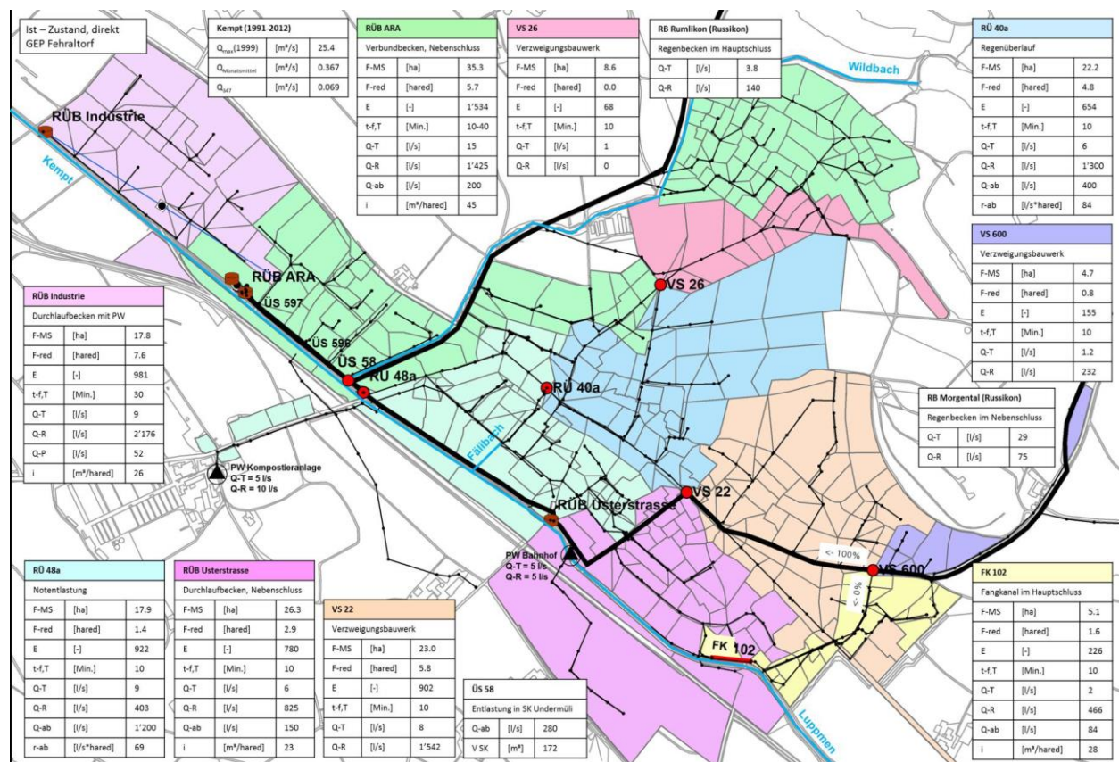
Figure S8. Subcatchment characteristics for hydrological modelling. F-MS [ha]: total area of the combined system; F-red [ha] : Runoff-efficient area (combined sewer system); E_H :Inhabitants [-]; t-f,T [min]: flow time in the subcatchment ; Q-T [Ls -1 ]: dry weather runoff (daily peak = daily mean * 2.4); Q-R [Ls -1 ]: specific stormwater runoff for design storm; Q-ab [Ls -1 ]: flow rate; i [m³ ha -1 ]: specific storage volume; r-ab [Ls -1 *ha -1 ]: specific carry-on flow. (Figure corresponds to “Abbildung 10-4, Einleitschema im Ist-Zustand, Kennzahlen direkt“ in HBT (2016))
