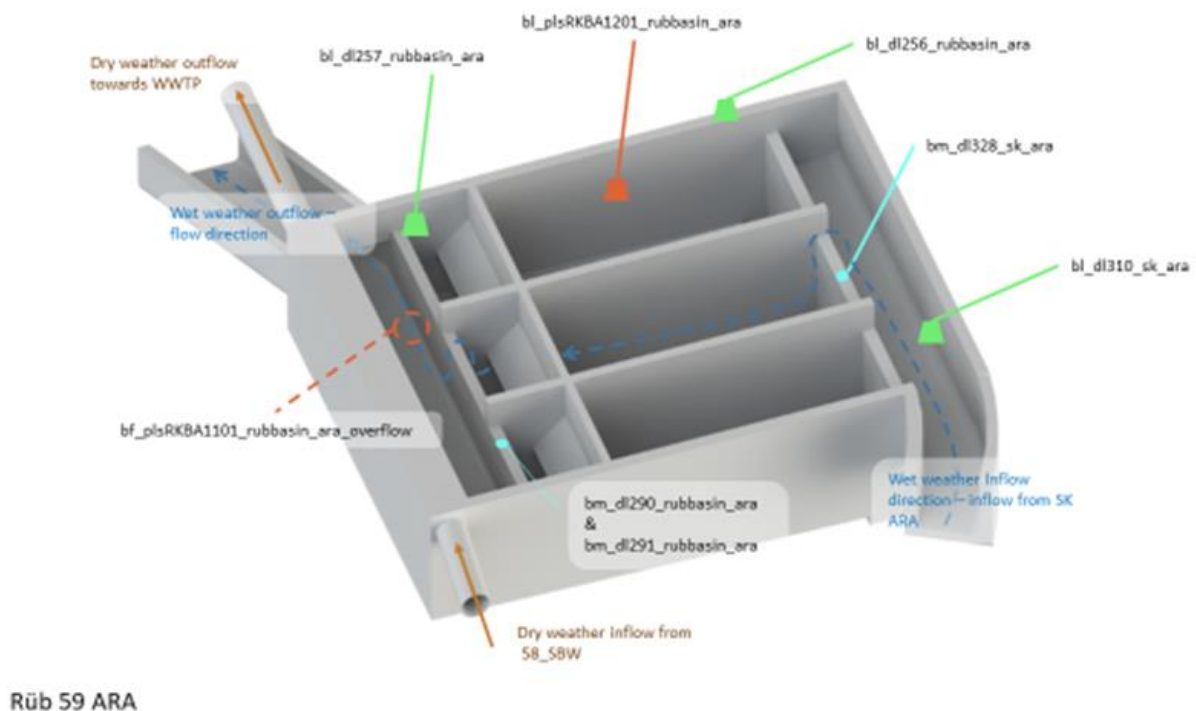
Figure S14. 3-D drawing of RUB 59 , i.e. RUB ARA , including sensor positioning and flow path during wet weather (dotted blue line).
