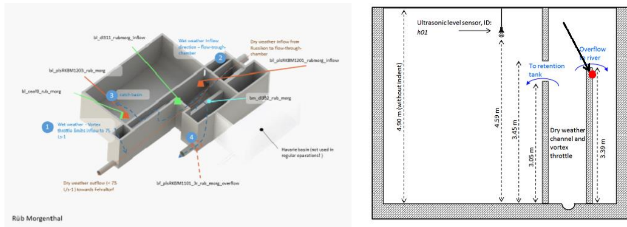
Figure S11. left figure: 3-D drawing of the RUB Morgenthal , including sensor positioning and flow path during wet weather. Right figure: Cross-section through the overflow structure RUB Morgenthal (not drawn to scale) including inflow chamber, retention tank, overflow to receiving water and installed sensors.
