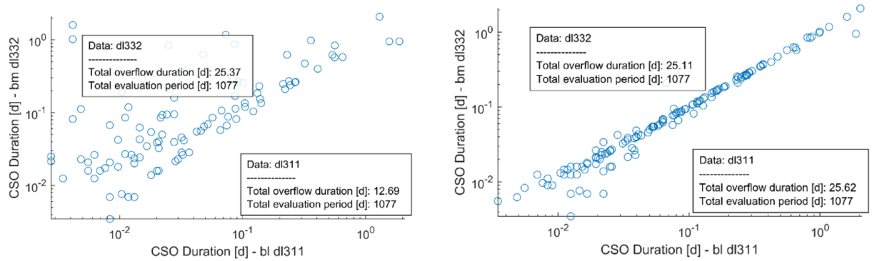
Figure S49. Comparison of event-specific overflow durations derived from one capacitive sensors and one ultrasonic level sensor (dl311), prior (left) and after (right) correctly implementing the sensor settings.
