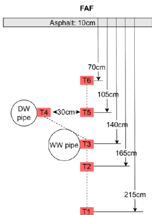
Figure S31. left: principal draft of the temperature measurement positions ; right: photo at installation before they got buried in the soil.
