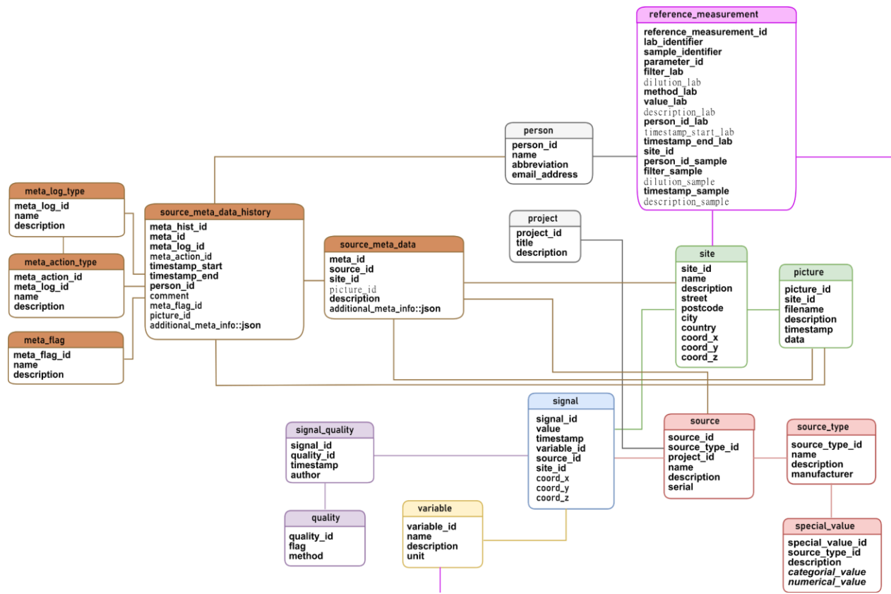
Figure S35. Schematic illustration of the Datapool's data model or database layout. All data is stored in a PostgreSQL database so that arbitrary queries can be performed.
