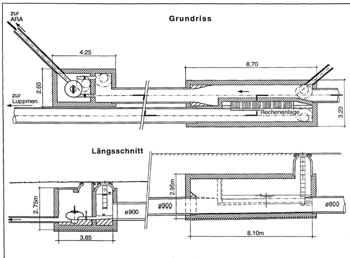
Figure S12. Top: FK 102 - planar view (Grundriss); bottom: FK 102 - longitudinal cross-section ("Längsschnitt") - taken from Krejci (1994).
