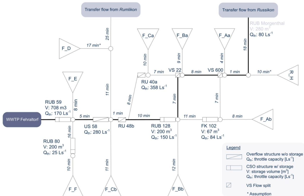
Figure S10. Hydrologic flow scheme of the Fehraltorf (combined) sewer network. The main flow path (bold line) is from top right (RUB Morgenthal) to the left (WWTP Fehraltorf). Triangles represent aggregated sub-catchments. Indicated flow times are estimated assuming an average flow velocity in the sewer of 1 m s -1 and verified through field experiments. Cf. Figure 2, main paper. Version: 15-Jan-2024.
