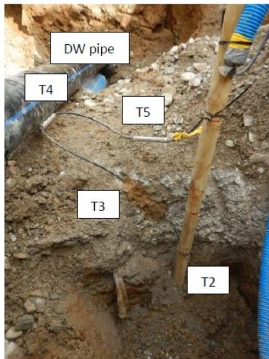
Figure S31. left: principal draft of the temperature measurement positions ; right: photo at installation before they got buried in the soil.
