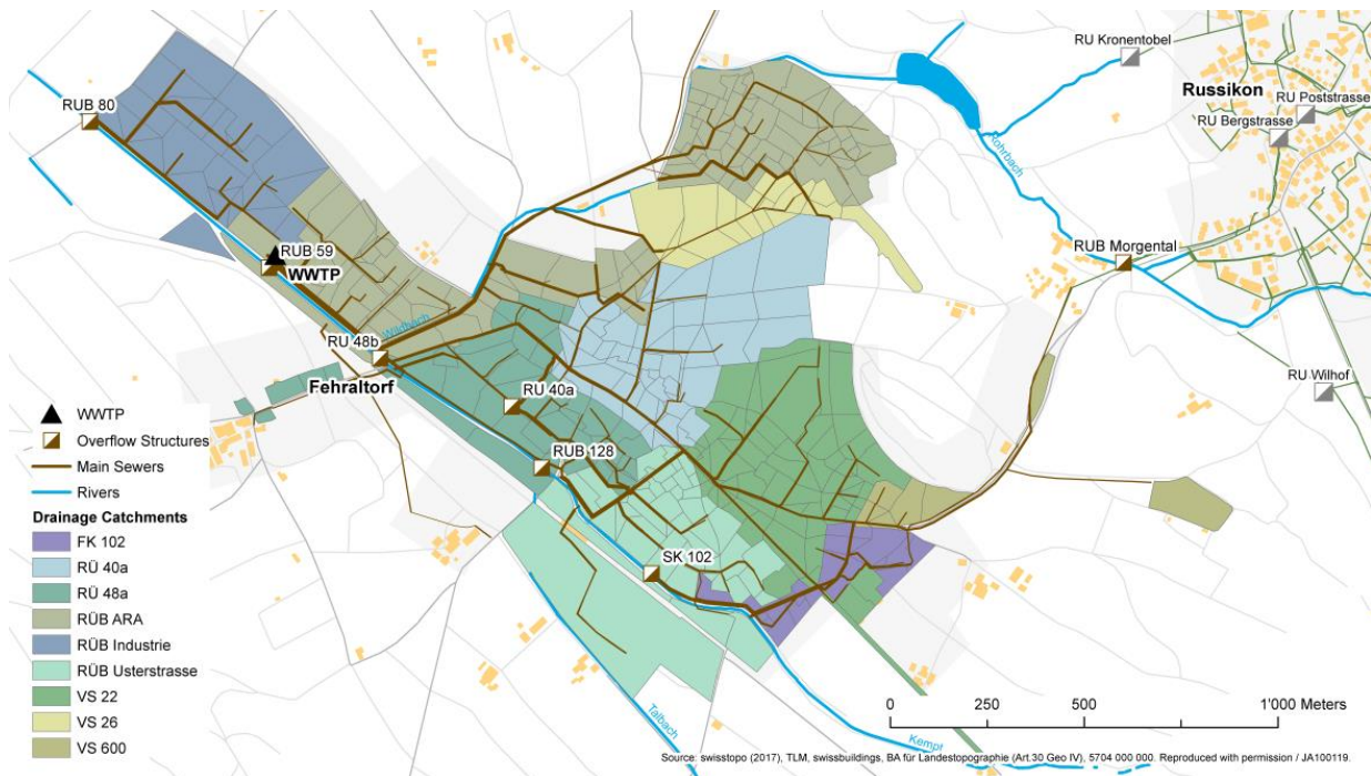
Figure S39. Differentiation of CSO sub-catchments in the Fehraltorf combined sewer system. Source: ©Swisstopo (2017), TLM, swissbuildings, BA für Landestopographie (Art. 30 Geo IV), 5704 000 000 Reproduced with permission / JA 100119
