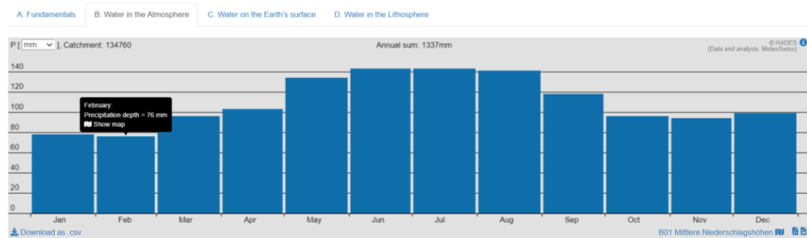
Figure S2. Long-term mean of monthly precipitation depths, in mm
