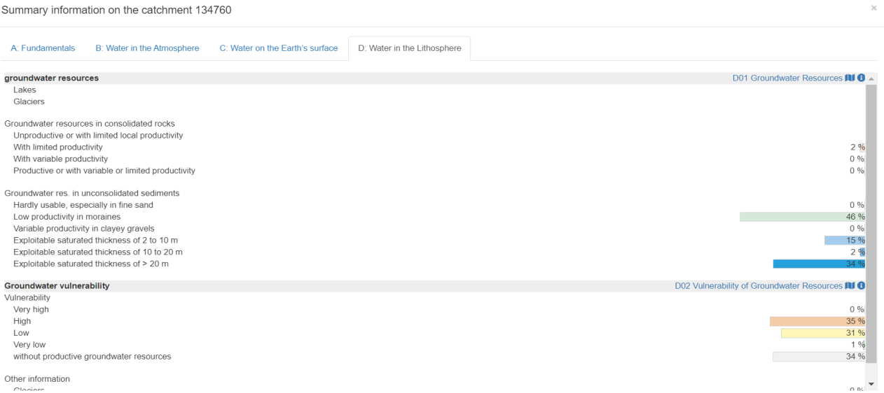
Figure S4. Groundwater resources and vulnerability
