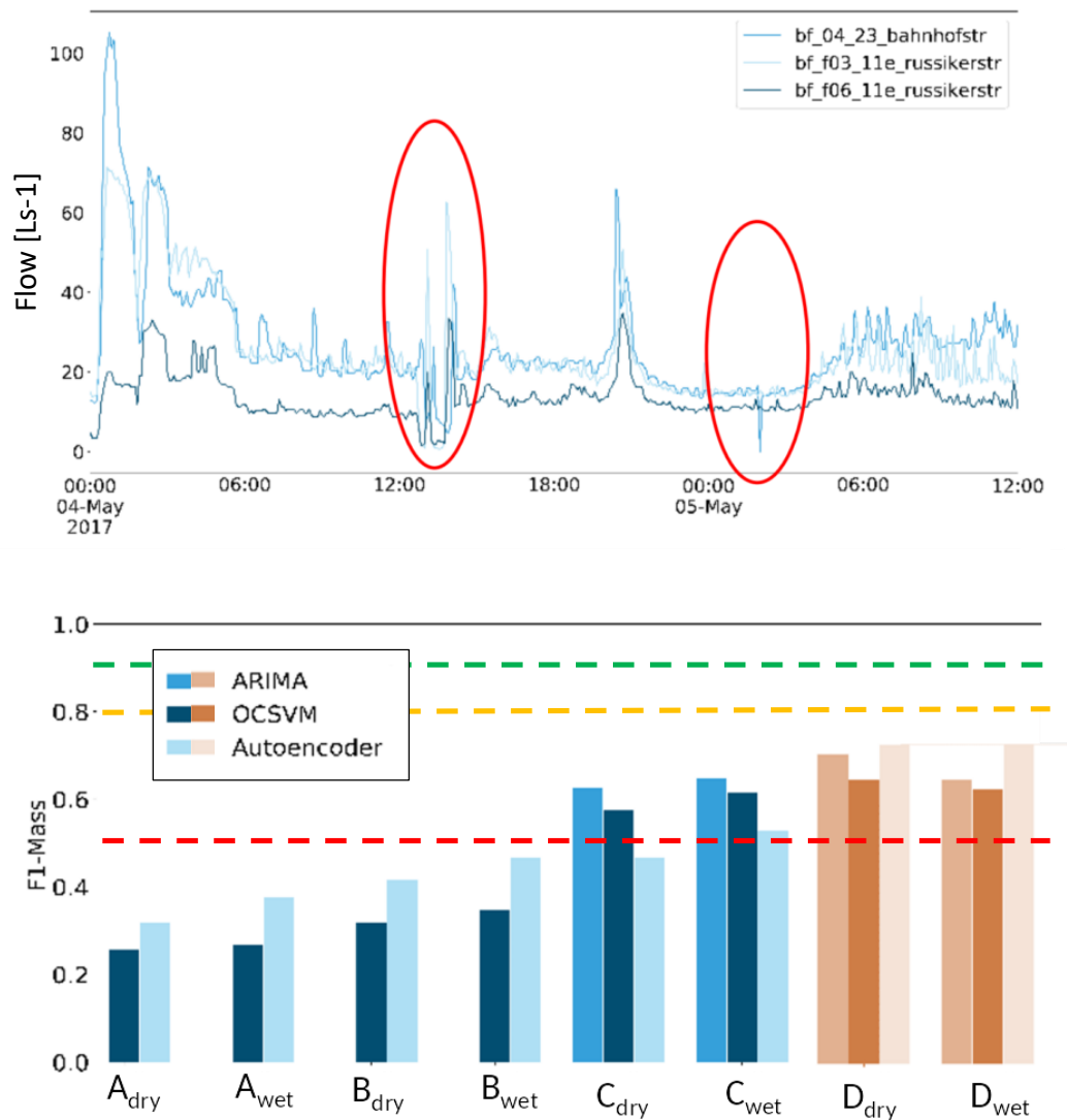
Figure S44. Top: Observations with potential anomalies. The highlighted data show the benefit of multiple sensors in detecting anomalies. While the high variability on the left is reflected in all sensors, the one on the right only appear in a single sensor. Bottom: F1 scores for different methods for pre-processing (A-D). An F1 score of 0.5-0.8 (between the red and yellow dashed lines) is considered medium quality, 0.8-0.9 good and above 0.9 excellent. For real-world data (blue, A-C), the performance increases with increasing levels of pre-processing. For real world data, ARIMA performs best and the Autoencoder never reaches the performance on synthetic data (red, D).
