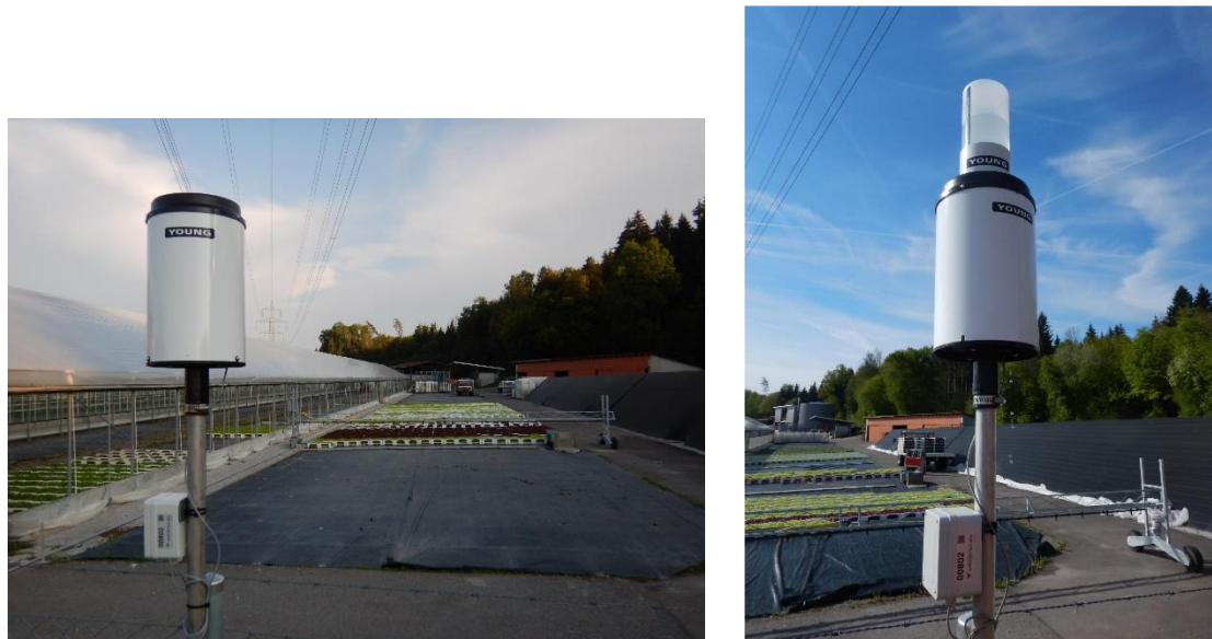
Figure S1. RM young with LoRaWAN-logger attached to the stand pole; right: rain gauge calibrator in action
