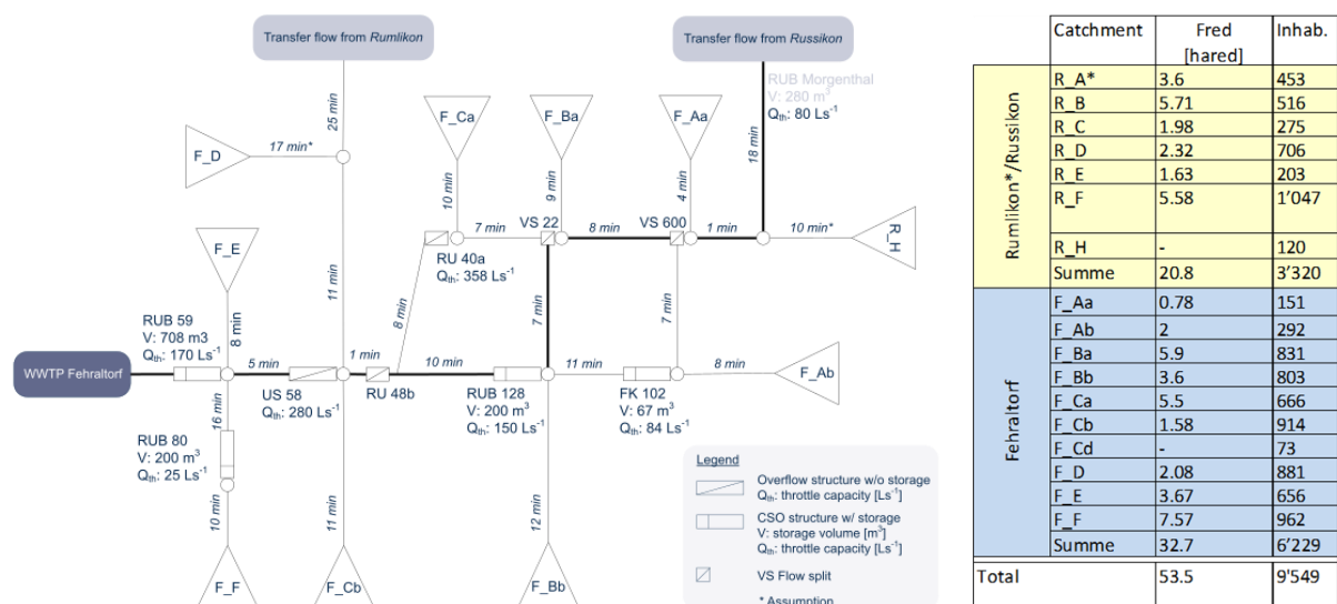
Figure S7. Flow topology (left) and aggregated information on the subcatchments (right).
