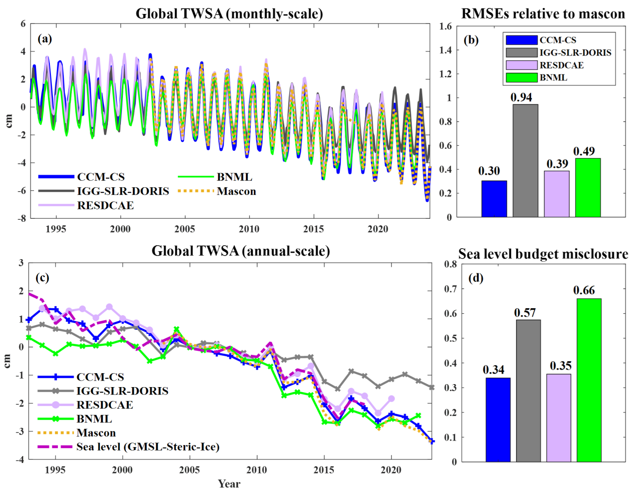
Figure 9. Time series of global TWAs (excluding Greenland and Antarctic) at (a) monthly and (c) annual temporal scale from various solutions (January 1993–December 2024); (b) RMSEs of monthly TWSA series relative to mascon products (April 2002–December 2020), and (d) sea level budget misclosure from annual TWSA series (January 1994–December 2020).
