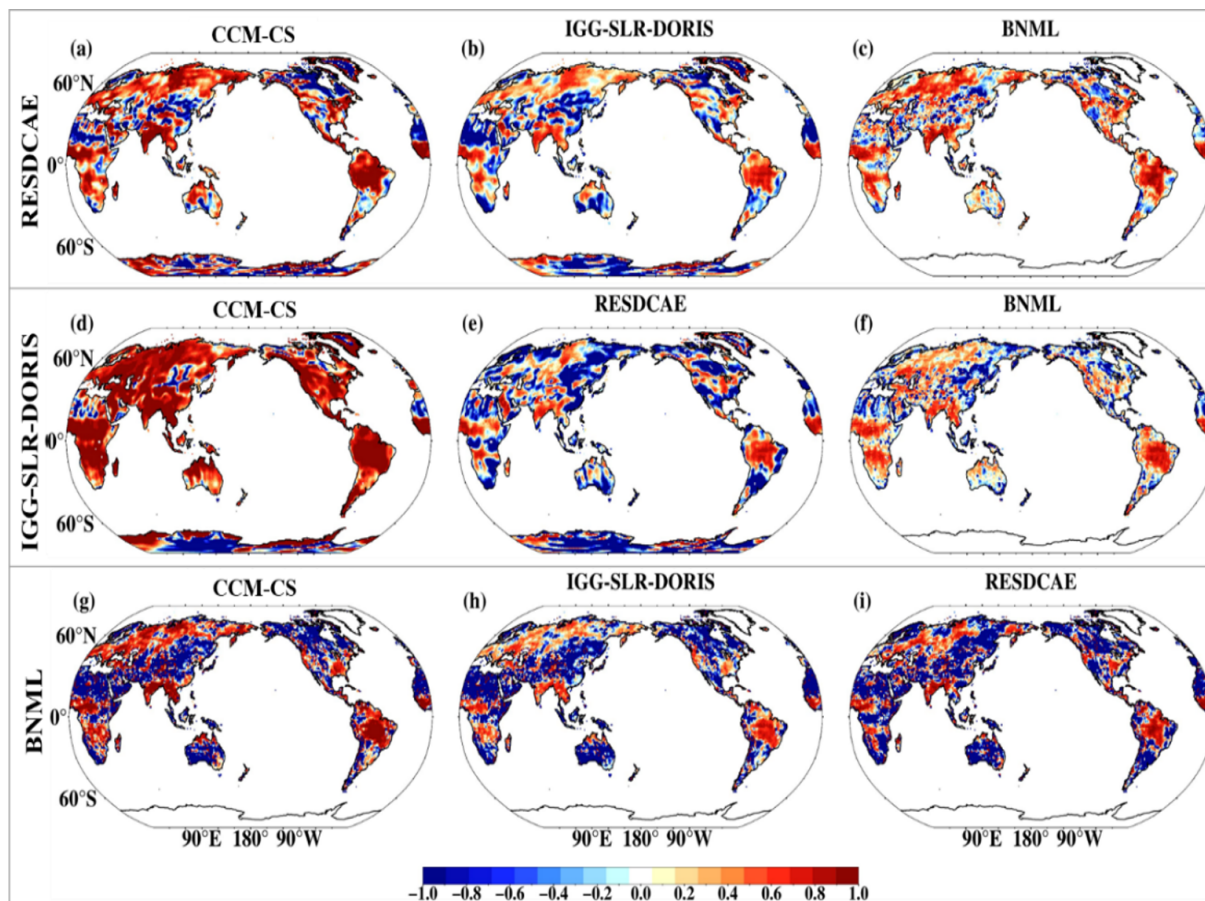
Figure 7. NSE values of global TWASs from various solutions relative to RESDCAE, IGG-SLR-DORIS, and BNML corresponding to the first to third rows (January 1994–December 2020).
