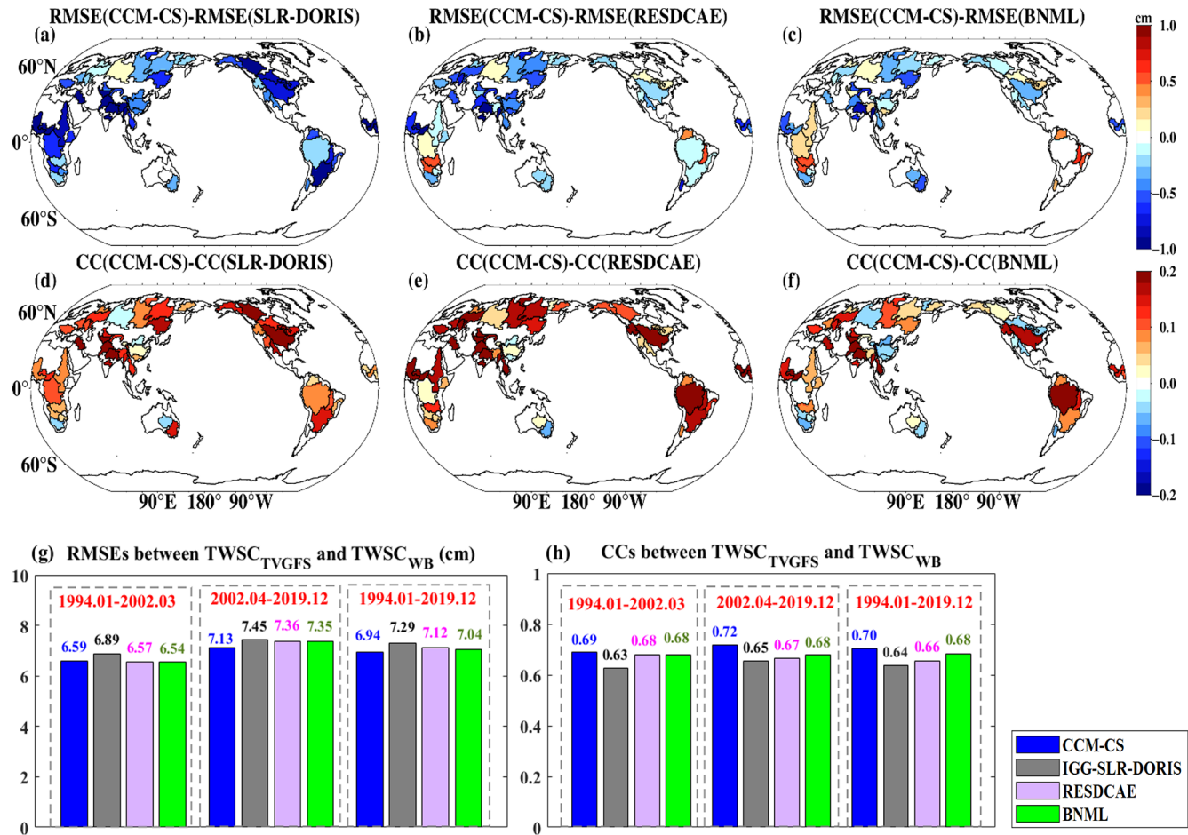
Figure 10. (a–c) RMSEs and (d–f) CCs between TWSC CCM and TWSC WB relative to those for TWSC SLR-DORIS , TWSC RESDDAE , and TWSC BNML ; and average (g) RMSEs and (h) CCs across 52 basins during pre-GRACE (January 1994 to March 2002), GRACE/-FO periods (April 2002 to December 2019), and the entire common period (January 1994 to December 2019).
