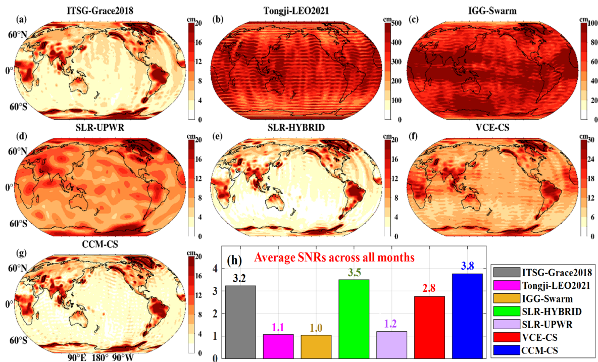
Figure 2. (a–g) RMS of spatial TWSAs and (h) average SNRs from individual and combined solutions over their respective available periods.
