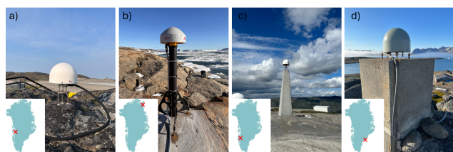
Figure 3. Comparison of the most common antenna monuments used in GNET. (a) bedrock-bolted plate (ILUL). (b) bedrock-bolted mast (NGFJ). (c) concrete monument (KLSQ). (d) older version of the concrete monument (KULU). Pictures: Thomas H. Nylen and Christian Solgaard.
