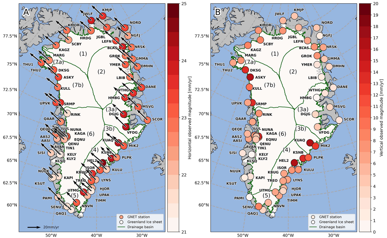
Figure 7. Derived horizontal and vertical linear motion from GNET measurements from 1995–2025. The uncertainty for the new stations (see Table 1) will be of a magnitude larger than the older installations, see Table A1. (a) Horizontal observed magnitude with absolute direction indicated as arrows, values provided in \text{mm yr}^{-1} . (b) Vertical observed magnitude given in \text{mm yr}^{-1} . For further information on the vertical and horizontal land motion of Greenland see Berg et al. (2024, 2025).
