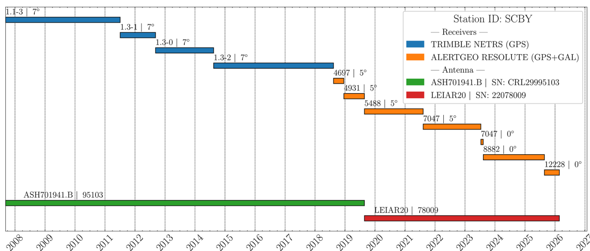
Figure 10. Representation of the IGS sitelog of station SCBY. Information for receivers is “Firmware Version” | “Elevation Cutoff Angle” and the antenna information is “Antenna Model” | “Short Serial Number”, the station sitelog shown here corresponds to the final ENU time series shown in Fig. 6.
