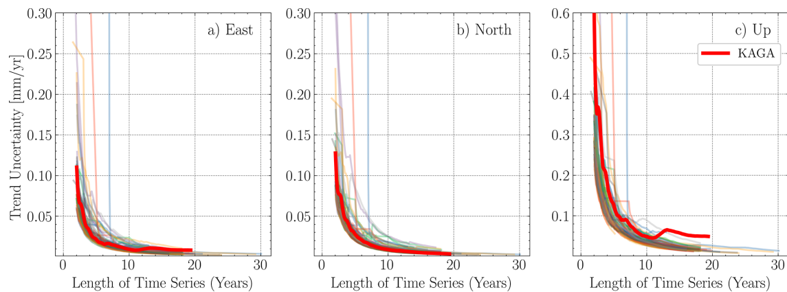
Figure 14. Trend uncertainty estimations as a function of time series length for all stations. Iteratively estimated trend uncertainty for the (a) East, (b) North, and (c) Up components. First estimate at time series length of 2 years, with each step adding 1 month to the time series.
