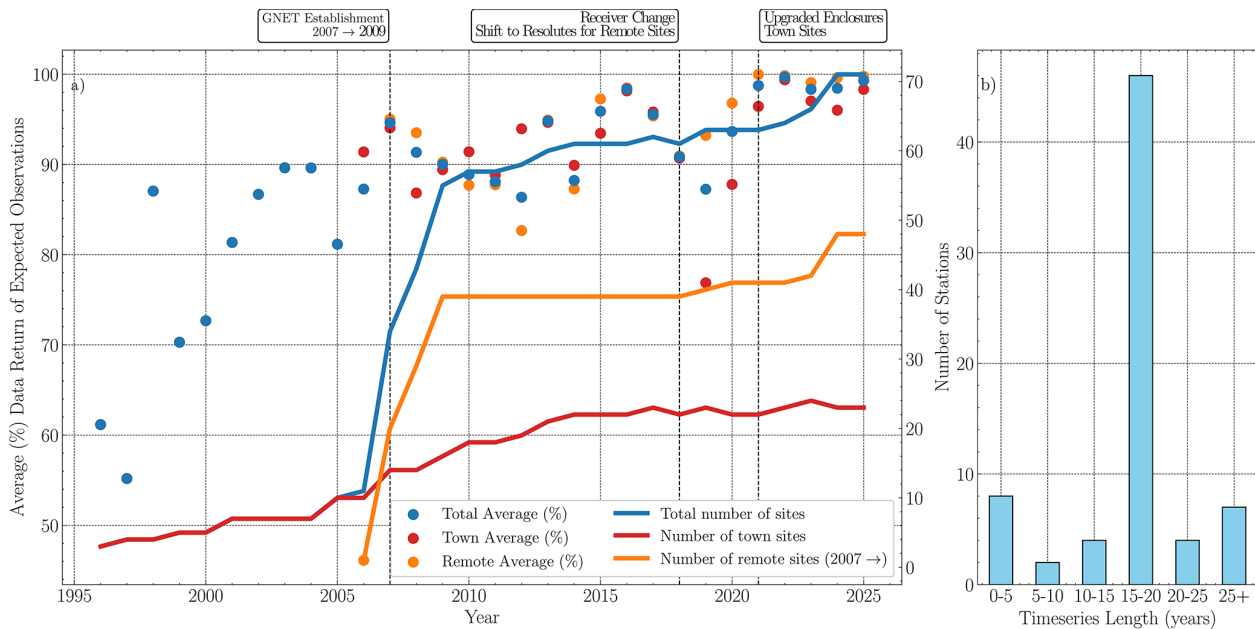
Figure 8. (a) Left y axis: Average data return [%] of expected observations per day, normalized to a sampling rate of 15 s over the full network. Right y axis: Total number of stations in the network, split into remote and town sites. The remote sites were first established during the establishment of GNET in the 2007–2009 summer seasons. Some town sites predate GNET back to 1995 (KULU). In 2024, the number of remote sites was expanded with 6 new sites: one in East Greenland (UPAK), one in North East Greenland (NGFJ), and four in the Icefjord area from Ilulissat towards Sermeq kujalleq (NUNA, AVAN, EQNU and QENU). (b) Length of the time series distributed over the number of stations in the network.
