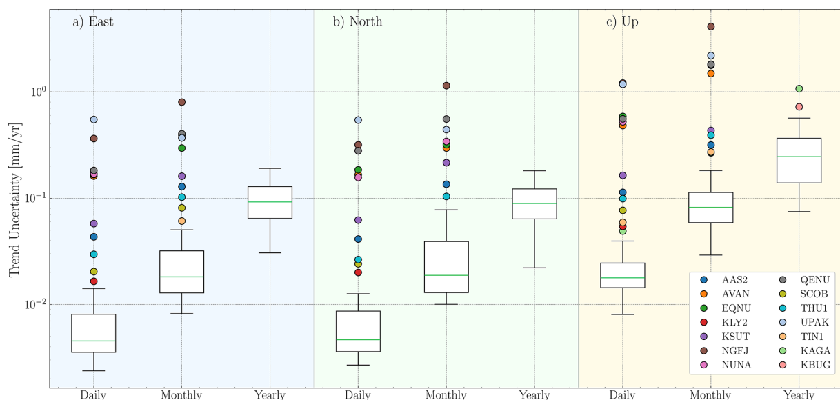
Figure 15. Velocity error distributions for daily estimates, monthly means, and yearly means. (a) Error estimates for the east direction for all 71 stations. (b) same as (a), but for the north direction. (c) same as (a) and (b), but for the upward direction. Note that the y axis is logarithmic.
