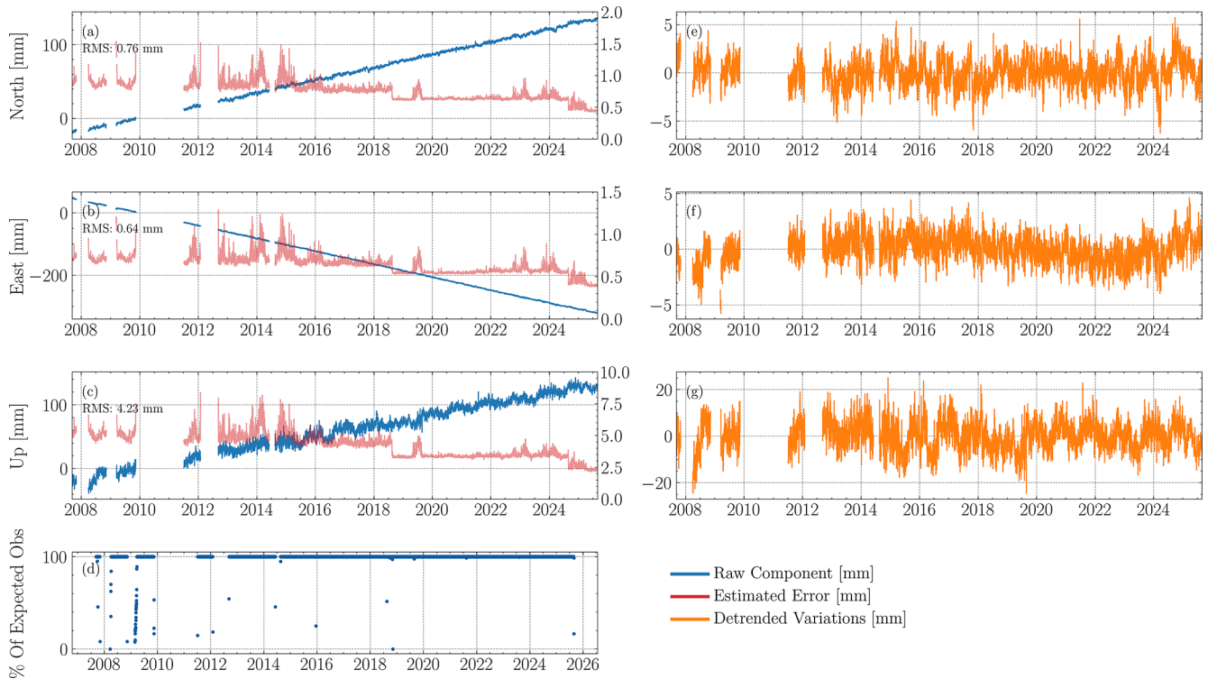
Figure 6. Time series of final processed ENU for station SCBY (Kap Scouby) in Northwest Greenland and the associated error estimates for each coordinate component. (a) north component, (b) east component, (c) up component, all represented in [mm], in reference to the starting coordinate as specified in the metadata for the station. Notice the different scales on the left- and right-hand y axes. The right y axis shows the error estimates of the PPP solution. The time series are provided as a daily product. (d) shows the % of expected observations for the site, normalized to a sampling rate of 15 s. The station results shown here correspond to the IGS logbook visualized in Fig. 10. (e–g) Short term variations for each component, derived by removing the linear trend from each component shown in (a)–(c).
