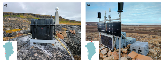
Figure 5. (a) The town site QEQE just outside of Qeqertarsuaq on Disko Island in Vest Greenland. The enclosure is provided with power from the town grid, connection is through a GSM antenna placed on top of the pelican case, current receiver type across all town sites is the Septentrio PolaRx5 GNSS receiver (Septentrio, 2025). (b) The remote site KMJP at Kap Morris Jessup, North Greenland. The power is provided by up to four solar panels and a total of up to 24 100 Ah lead-acid batteries in the MM36 pelican cases, depending on latitude. Communication is through the Iridium network; the current receiver across all remote sites is the AlertGEO Resolute GNSS receiver (Xeos Technologies Inc., 2024). Pictures: Christian Solgaard.
