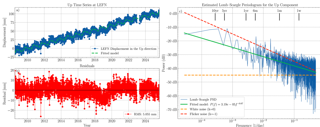
Figure 11. Example of fitting and removal of the deterministic trajectory model and evaluation of the Lomb-Scargle Periodogram. (a) Up component from station LEFN and fitted model. (b) Corresponding residual time series after the removal of the model. (c) Evaluated Lomb-Scargle Periodogram and the fitted power law model for estimation of the spectral index.
