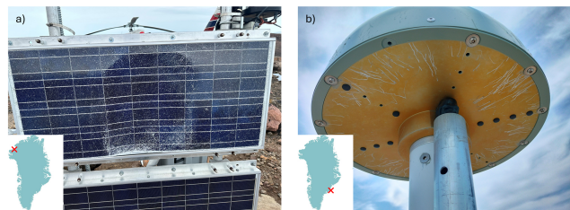
Figure 4. Examples of damaged GNSS equipment after the encounter with a polar bear. (a) destroyed the solar panel at KAGZ. (b) bite marks of a polar bear on the underside of the GNSS antenna at PLPK, no extra multipath error has been observed since the incident. Pictures: Thomas Nylen and Christian Solgaard.
