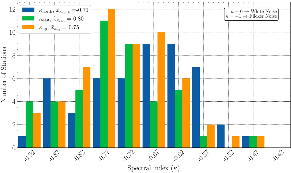
Figure 12. Spectral index \kappa histogram, of all stations included in the published dataset.
