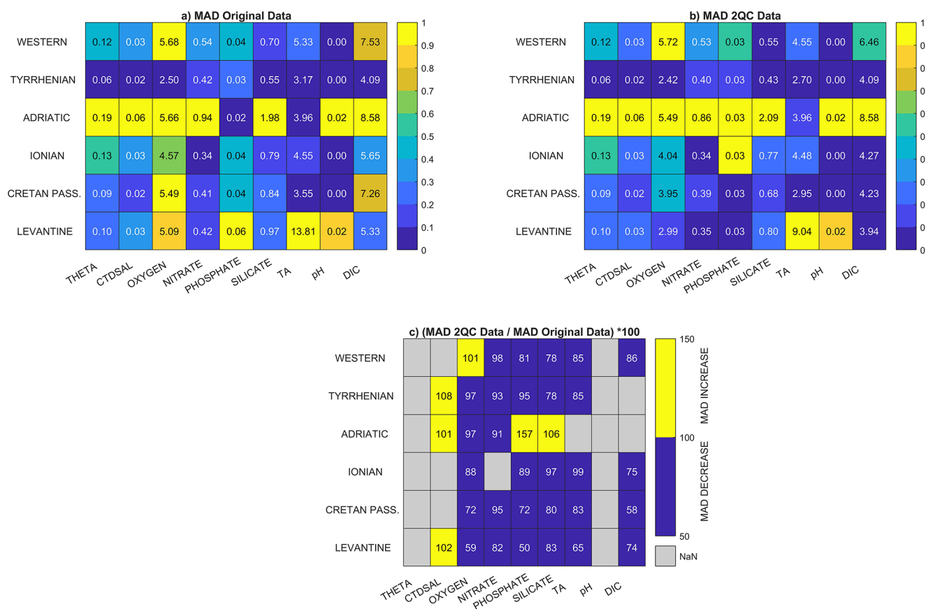
Figure 3. Overall Mean Absolute Deviation (MAD) (a) before and (b) after applying the 2QC adjustments to the CARIMED cruise collection. MAD are calculated for different Mediterranean Sea regions defined after Manca et al. (2004) and within the depth layers of minimum temporal variability (Sect. 5.1). Regions are shown in the y-axis and physical and biogeochemical variables in the x-axis: potential temperature (THETA, in °C), salinity (CTDSAL), dissolved oxygen (OXYGEN, in \mu\text{mol kg}^{-1} ), dissolved inorganic nutrients (NITRATE, PHOSPHATE, and SILICATE, all in \mu\text{mol kg}^{-1} ), total alkalinity (TA, in \mu\text{mol kg}^{-1} ), pH on the total hydrogen ion scale at 25 °C (pH), and total dissolved inorganic carbon (DIC, in \mu\text{mol kg}^{-1} ). The Western Basin comprises areas DF1 and DS4 (Algero-Provençal and Algerian East); the Tyrrhenian Basin comprises areas DT1 and DT3 (Tyrrhenian Sea North and Tyrrhenian Sea South); the Adriatic Basin comprises area DJ3 (Adriatic South); the Ionian Basin comprises areas DJ5, DJ7, and DJ8 (Ionian South, Middle East, and West, respectively); the Cretan Passage region comprises area DH3 (Cretan Passage), and the Levantine Basin comprises areas DL1, DL2, DL3, and DL4 (Levantine North, North East, South and South East, respectively) (see Figs. 1 and S3 and Table 2 for more information).
