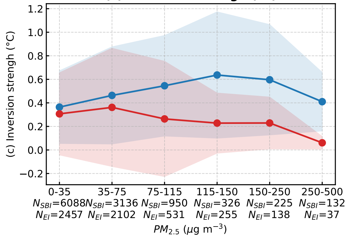
(c) Inversion strength ( ^{\circ}C )
