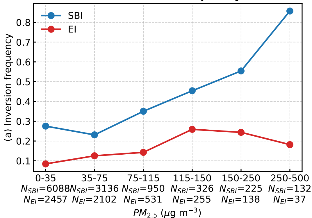
(a) Inversion frequency
