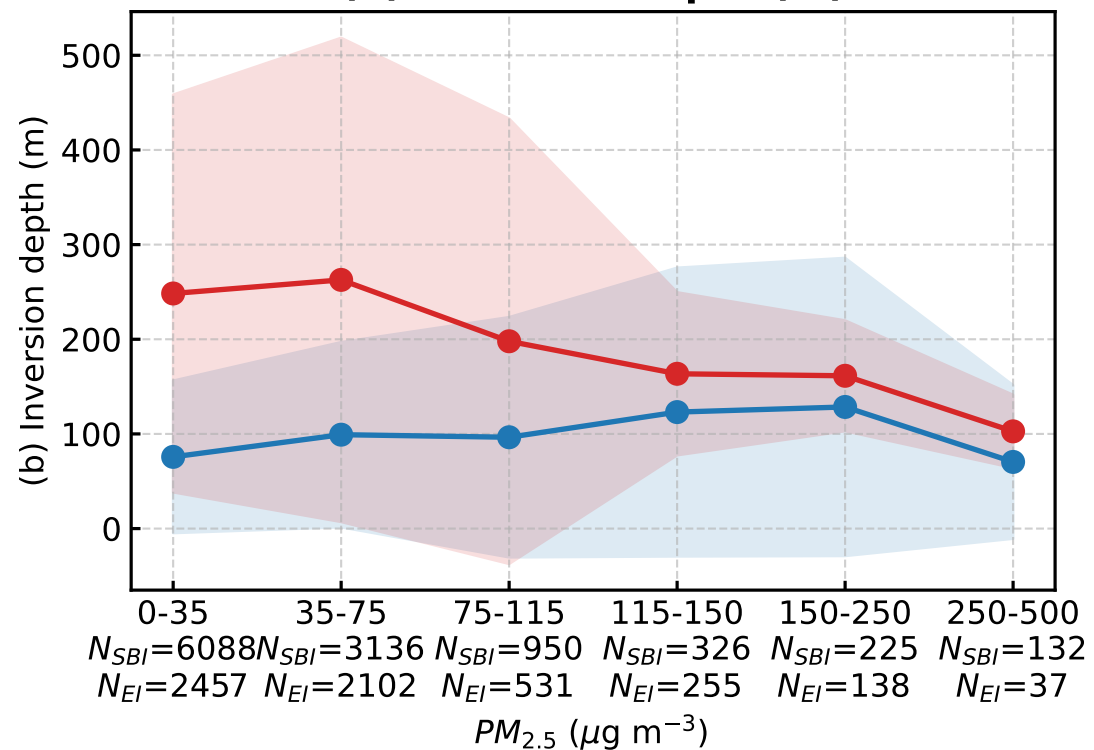
(b) Inversion depth (m)
