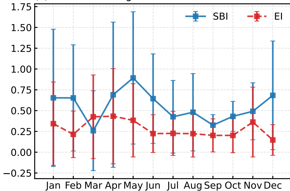
(c) Inversion strength
