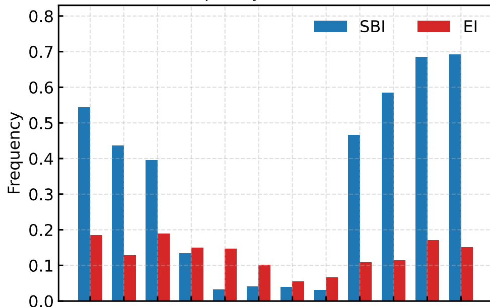
(a) Inversion frequency
