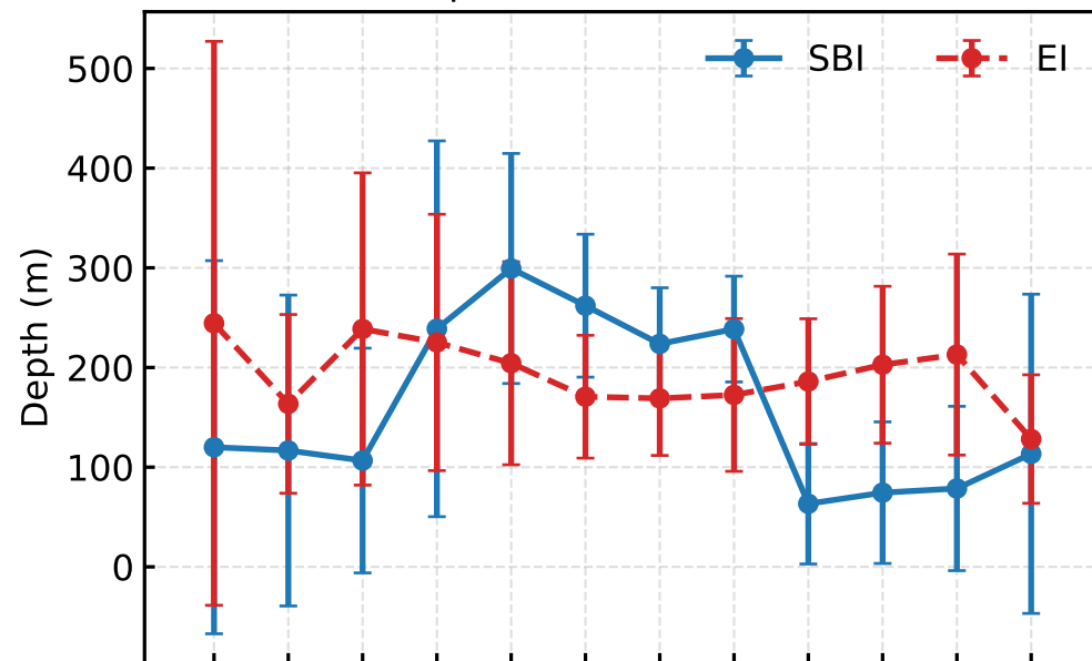
(b) Inversion depth
