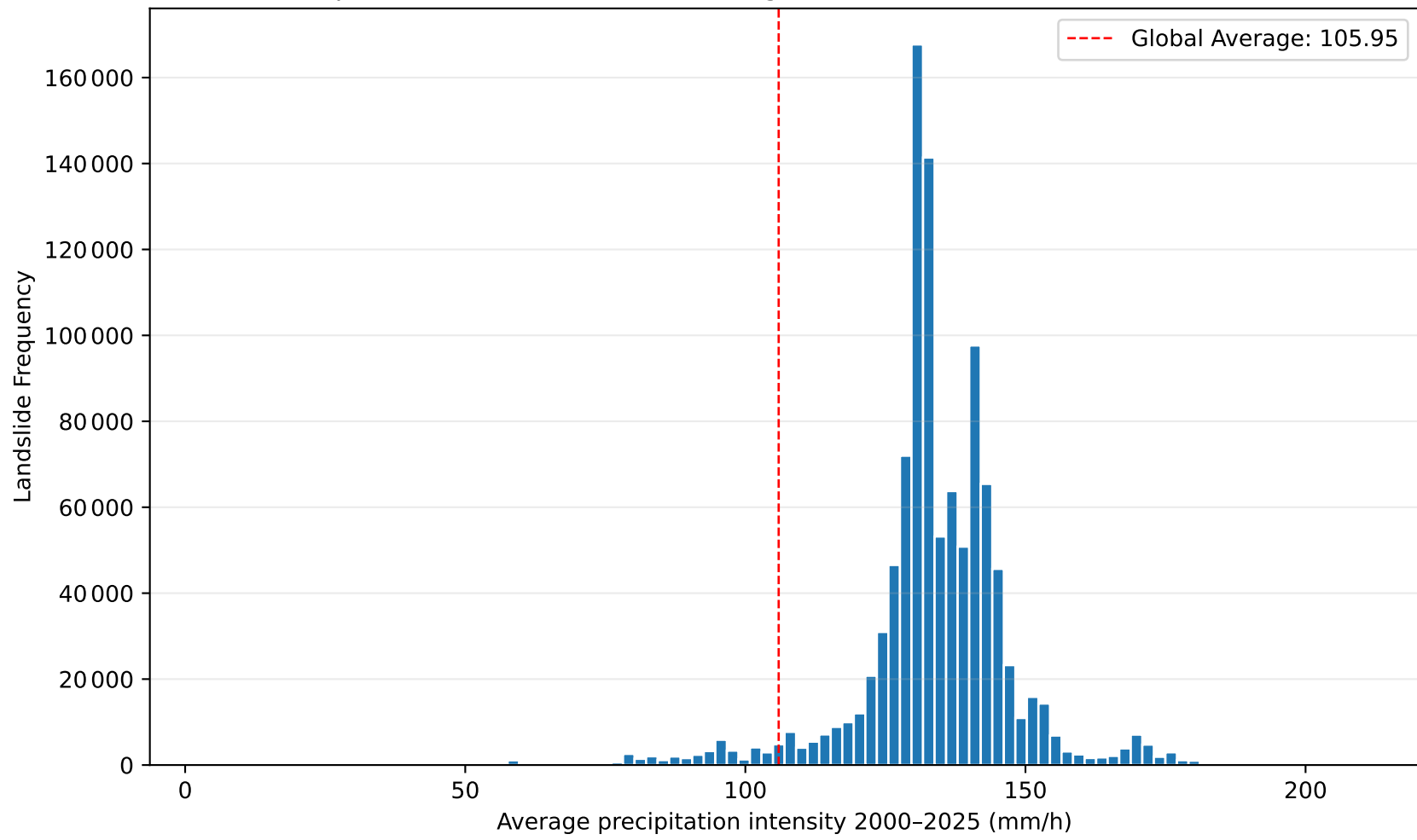
UGLC points - NASA GPM-IMERG (Integrated Multi-satellite Retrievals for GPM)
