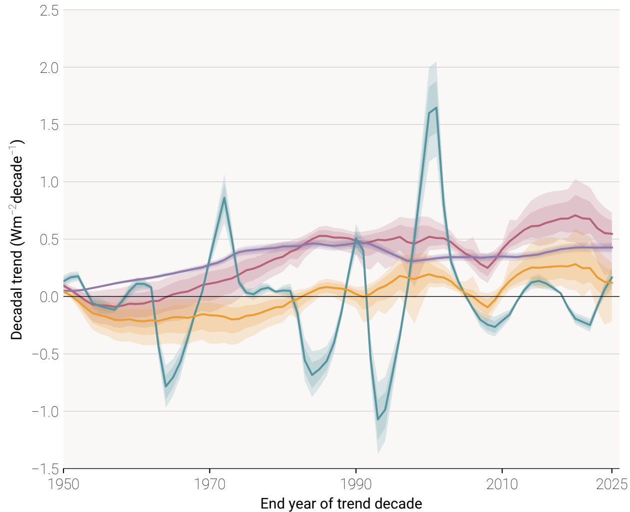
(b) Effective Radiative Forcing
