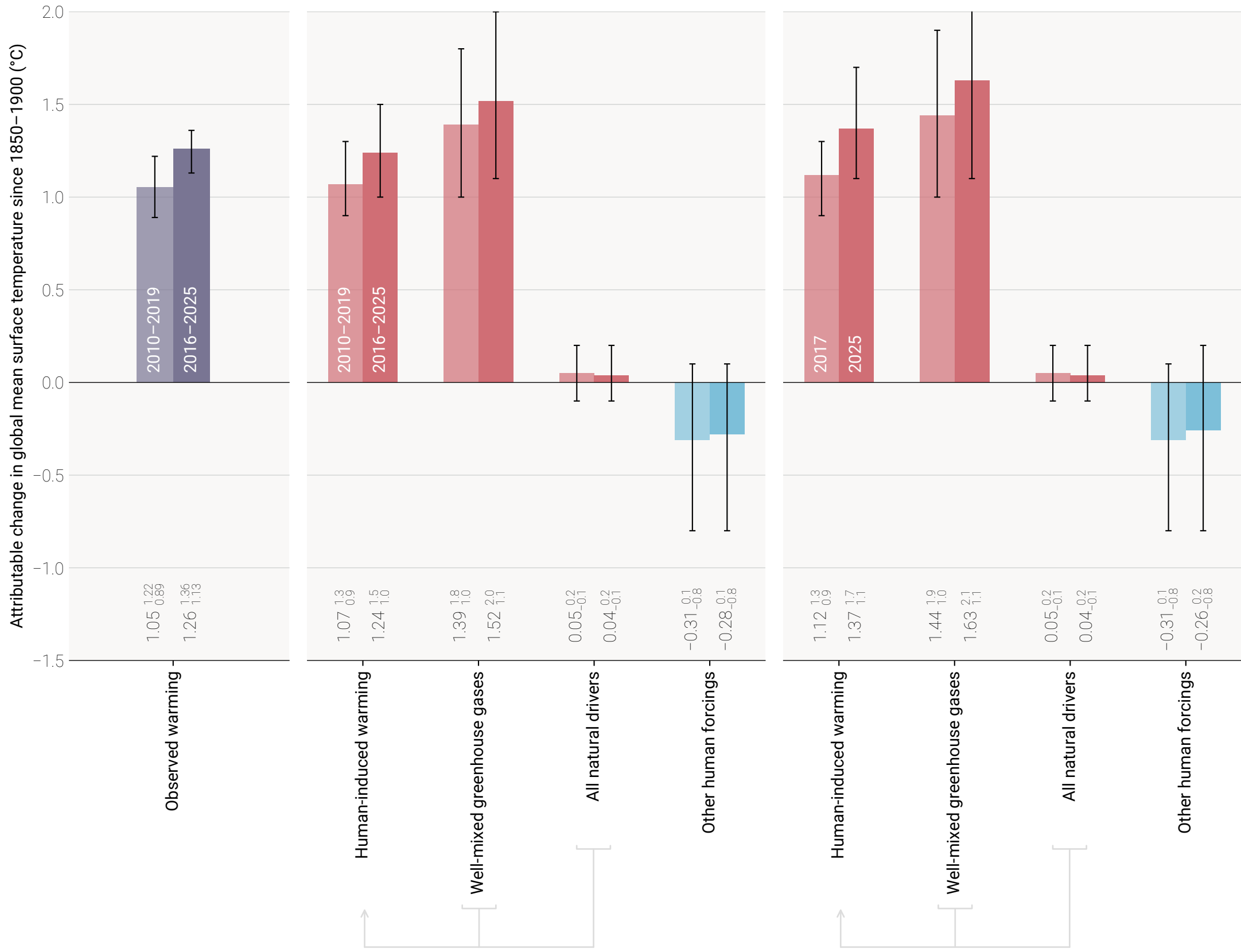
(a) Decade-average warming given by observations
