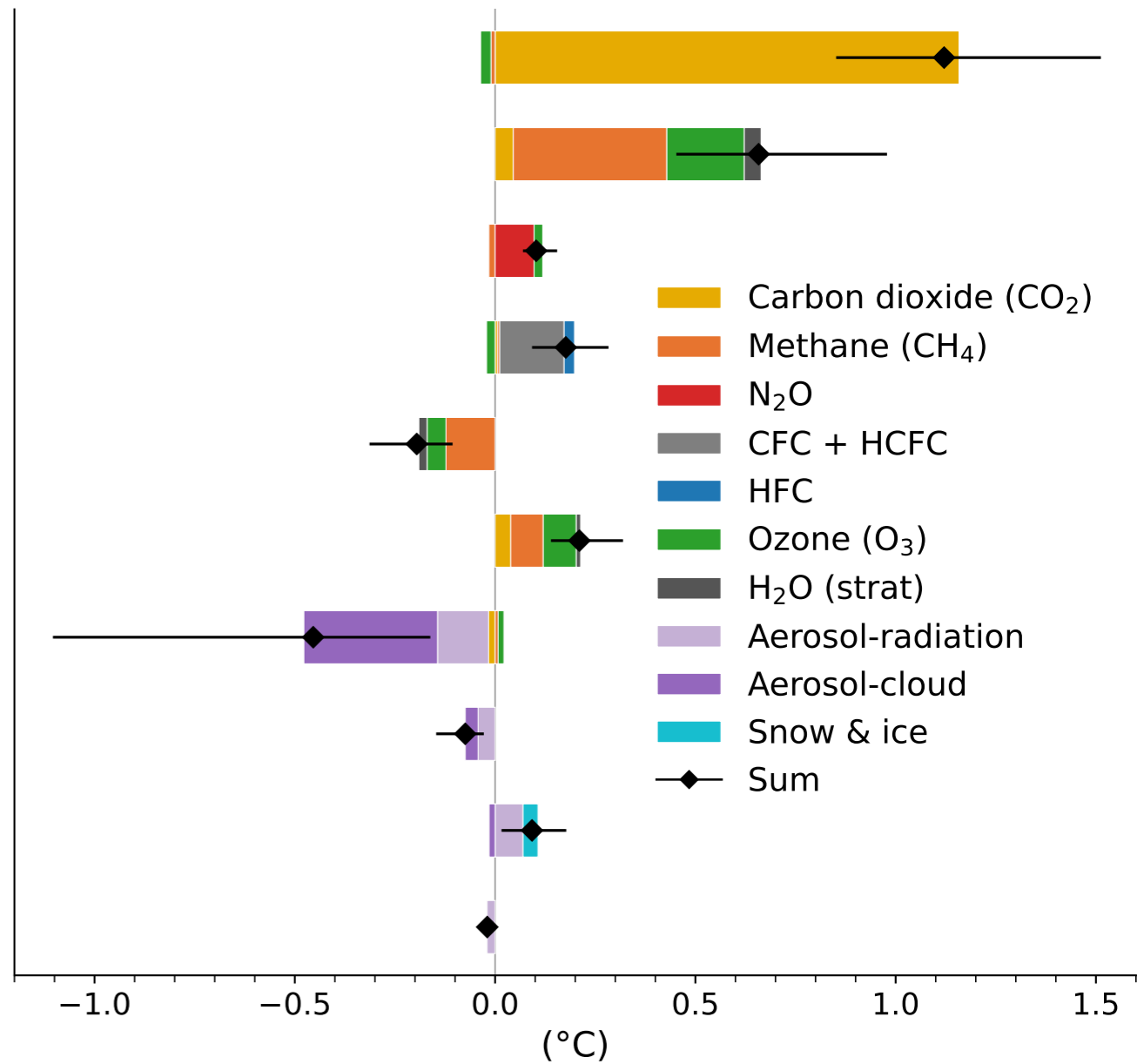
(b) Change in GSAT, 1750 to 2025
