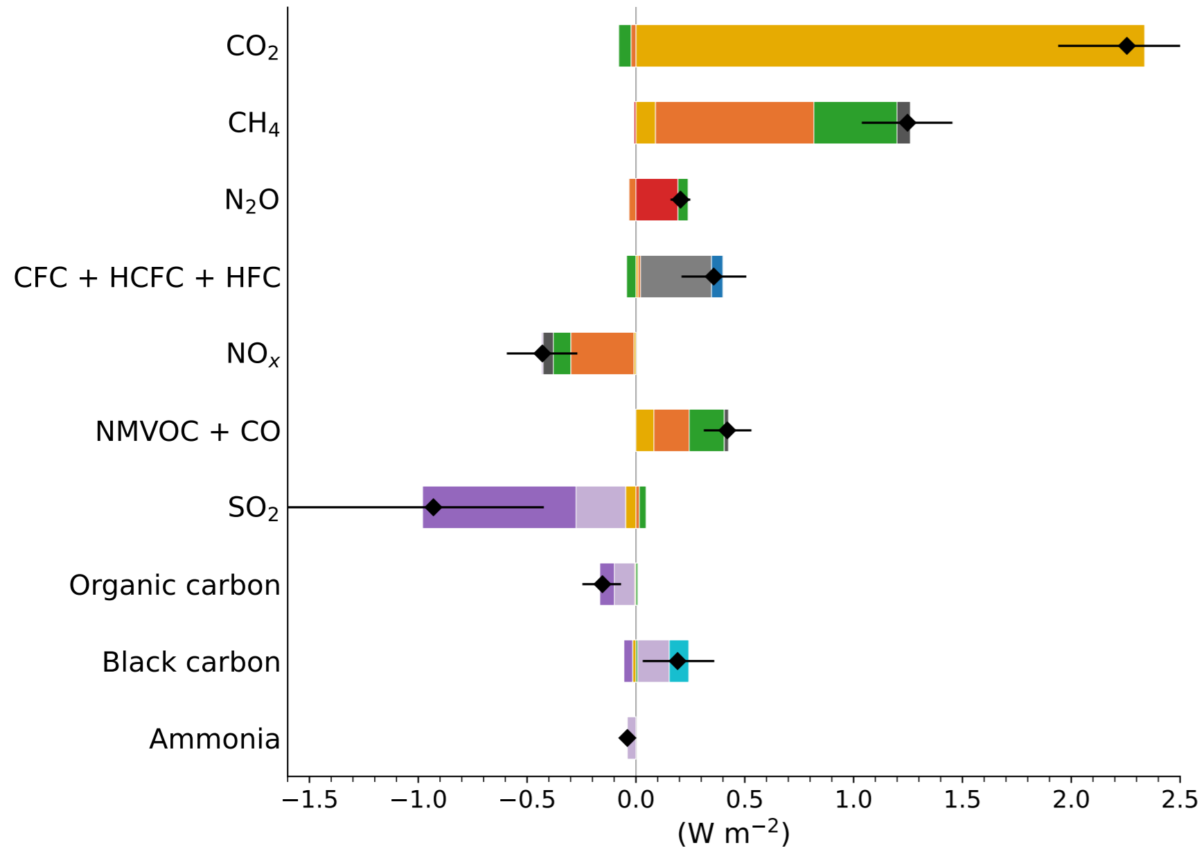
(a) Effective radiative forcing, 1750 to 2025
